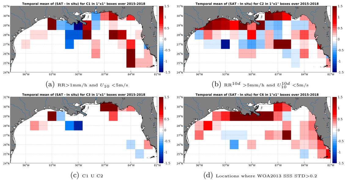
Figure 12: Temporal mean gridded over spatial boxes of size 1^\circ \times 1^\circ of \Delta SSS (SMAP-L3-RSS-V2-MONTHLY-0.25DEG-40KM - TSG-SAMOS) for 4 different subdatasets corresponding to:RR > 1 mm/h and U_{10} < 5 m/s (a), RR^{10d} > 5 mm/h and U_{10}^{10d} < 5 m/s (b), C1 U C2 (c),Locations where WOA2013 SSS STD > 0.2 (d).
