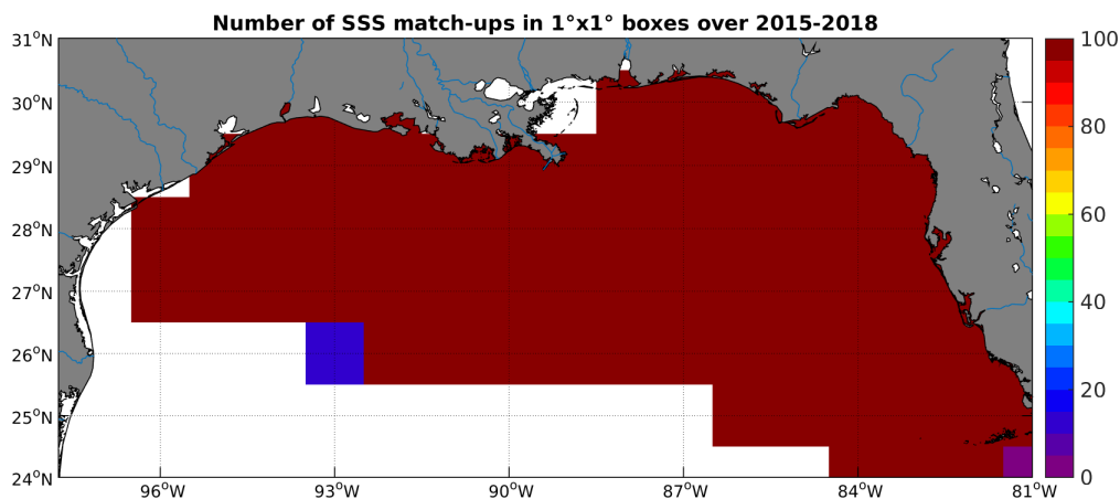
Figure 4: Number of SSS match-ups between TSG-SAMOS SSS and the SMAP-L3-RSS-V2-MONTHLY-0.25DEG-40KM SSS product for the Mississippi river plume Pi-MEP region over 1^\circ \times 1^\circ boxes and for the full satellite product period.
