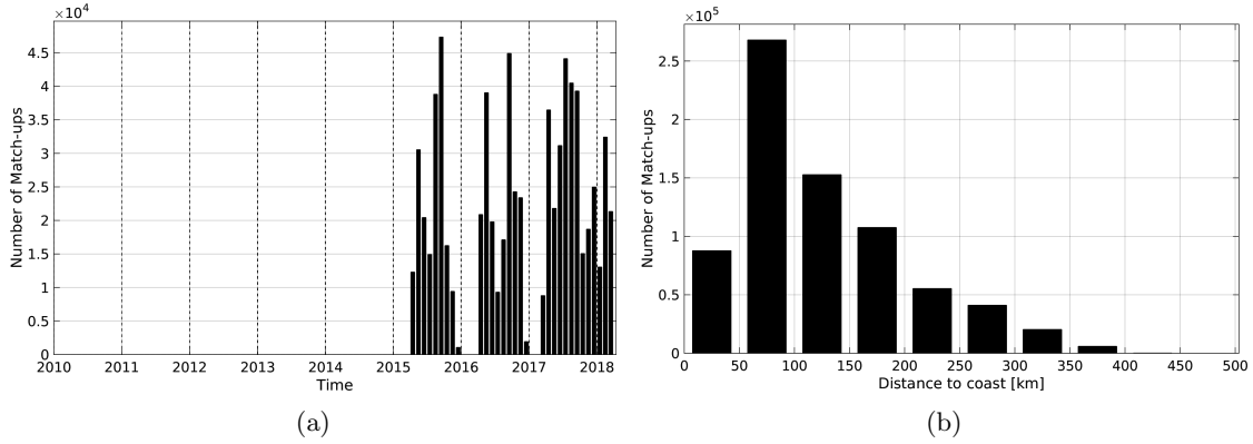
Figure 1: Number of match-ups between TSG-SAMOS and SMAP-L3-RSS-V2-MONTHLY-0.25DEG-40KM SSS as a function of time (a) and as function of the distance to coast (b) over the Mississippi river plume Pi-MEP region and for the full satellite product period.
