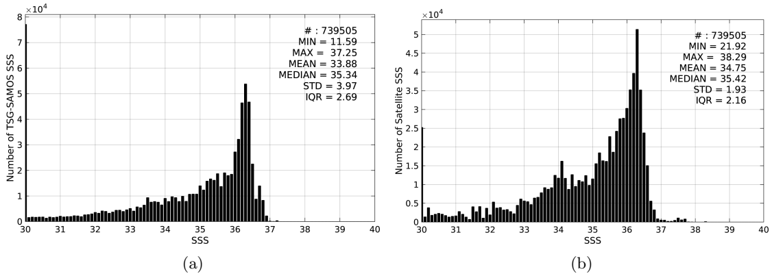
Figure 2: Histograms of SSS from TSG-SAMOS (a) and SMAP-L3-RSS-V2-MONTHLY-0.25DEG-40KM (b) considering all match-up pairs per bins of 0.1 over the Mississippi river plume Pi-MEP region and for the full satellite product period.
