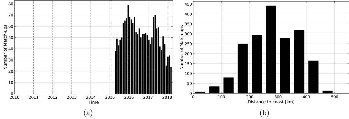
Figure 1: Number of match-ups between Argo and SMAP-L3-RSS-V2-MONTHLY-0.25DEG-40KM SSS as a function of time (a) and as function of the distance to coast (b) over the Mississippi river plume Pi-MEP region and for the full satellite product period.
