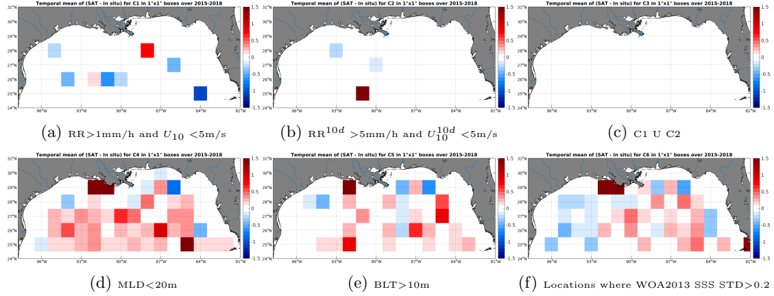
Figure 12: Temporal mean gridded over spatial boxes of size 1^\circ \times 1^\circ of \Delta SSS (SMAP-L3-RSS-V2-MONTHLY-0.25DEG-40KM - Argo) for 6 different subdatasets corresponding to: RR > 1\text{mm/h} and U_{10} < 5\text{m/s} (a), RR^{10d} > 5\text{mm/h} and U_{10}^{10d} < 5\text{m/s} (b), C1 U C2 (c), MLD < 20\text{m} (d), BLT > 10\text{m} (e), Locations where WOA2013 SSS STD > 0.2 (f).
