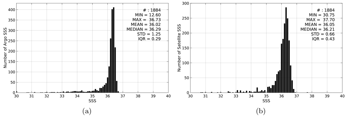
Figure 2: Histograms of SSS from Argo (a) and SMAP-L3-RSS-V2-MONTHLY-0.25DEG-40KM (b) considering all match-up pairs per bins of 0.1 over the Mississippi river plume Pi-MEP region and for the full satellite product period.
