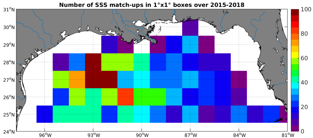
Figure 4: Number of SSS match-ups between Argo SSS and the SMAP-L3-RSS-V2-MONTHLY-0.25DEG-40KM SSS product for the Mississippi river plume Pi-MEP region over 1^\circ \times 1^\circ boxes and for the full satellite product period.
