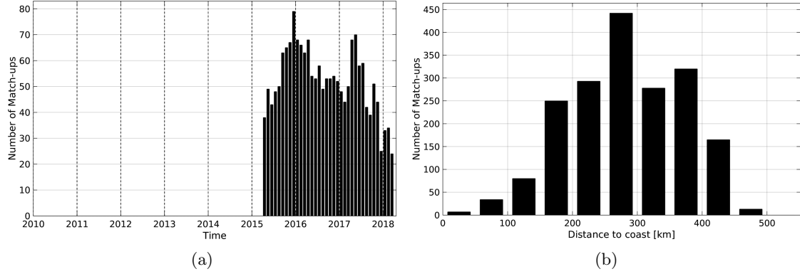
Figure 1: Number of match-ups between Argo and SMAP-L3-RSS-V2-MONTHLY-70KM SSS as a function of time (a) and as function of the distance to coast (b) over the Mississippi river plume Pi-MEP region and for the full satellite product period.
