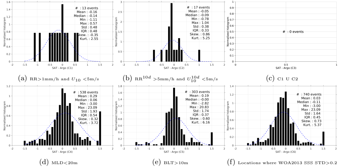
Figure 13: Normalized histogram of \Delta\text{SSS} (SMAP-L3-RSS-V2-MONTHLY-70KM - Argo) for 6 different subdatasets corresponding to: RR>1\text{mm/h} and U_{10}<5\text{m/s} (a), RR^{10d}>5\text{mm/h} and U_{10}^{10d}<5\text{m/s} (b), C1 U C2 (c), MLD<20\text{m} (d), BLT>10\text{m} (e), Locations where WOA2013 SSS STD>0.2 (f).
