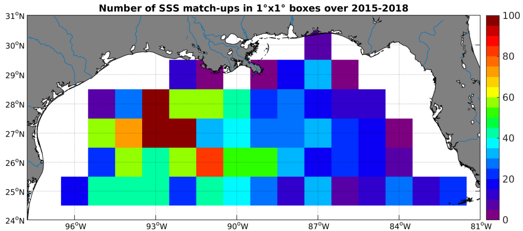
Figure 4: Number of SSS match-ups between Argo SSS and the SMAP-L3-RSS-V2-MONTHLY-70KM SSS product for the Mississippi river plume Pi-MEP region over 1^\circ \times 1^\circ boxes and for the full satellite product period.
