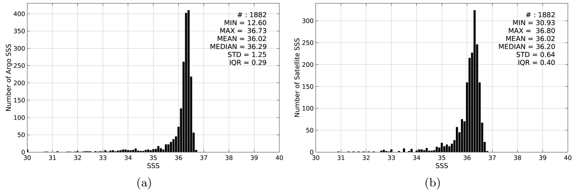
Figure 2: Histograms of SSS from Argo (a) and SMAP-L3-RSS-V2-MONTHLY-70KM (b) considering all match-up pairs per bins of 0.1 over the Mississippi river plume Pi-MEP region and for the full satellite product period.
