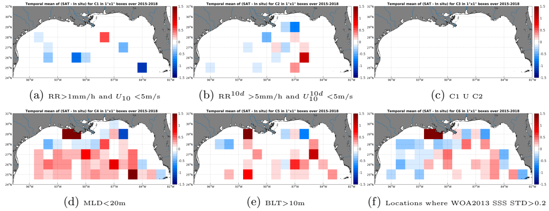
Figure 12: Temporal mean gridded over spatial boxes of size 1^\circ \times 1^\circ of \Delta SSS (SMAP-L3-RSS-V2-MONTHLY-70KM - Argo) for 6 different subdatasets corresponding to: RR > 1\text{mm/h} and U_{10} < 5\text{m/s} (a), RR^{10d} > 5\text{mm/h} and U_{10}^{10d} < 5\text{m/s} (b), C1 U C2 (c), MLD < 20\text{m} (d), BLT > 10\text{m} (e), Locations where WOA2013 SSS STD > 0.2 (f).
