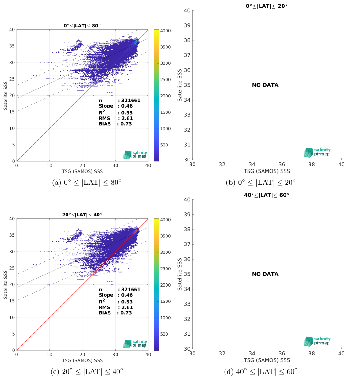
Figure 10: Contour maps of the concentration of SMAP SSS L3 v5.0 - 8-Day running (JPL) SSS (y-axis) versus TSG (SAMOS) SSS (x-axis) at match-up pairs for different latitude bands. For each plot, the red line shows x=y . The black thin and dashed lines indicate a linear fit through the data cloud and the \pm 95\% confidence levels, respectively. The number match-up pairs n , the slope and R^2 coefficient of the linear fit, the root mean square (RMS) and the mean bias between satellite and in situ data are indicated for each latitude band in each plots.
