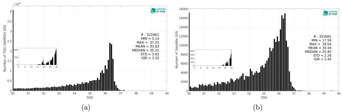
Figure 3: Histograms of SSS from TSG (SAMOS) (a) and SMAP SSS L3 v5.0 - 8-Day running (JPL) (b) considering all match-up pairs per bins of 0.1 over the Mississippi river plume Pi-MEP region and for the full satellite product period.
