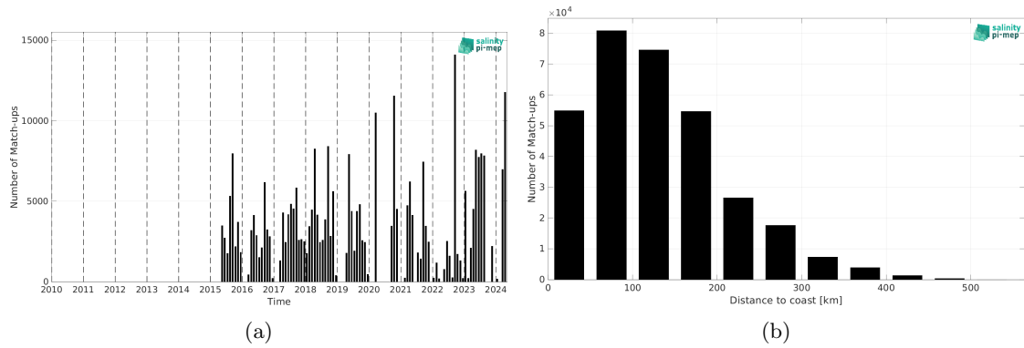
Figure 2: Number of match-ups between TSG (SAMOS) and SMAP SSS L3 v5.0 - 8-Day running (JPL) SSS as a function of time (a) and as function of the distance to coast (b) over the Mississippi river plume Pi-MEP region and for the full satellite product period.
