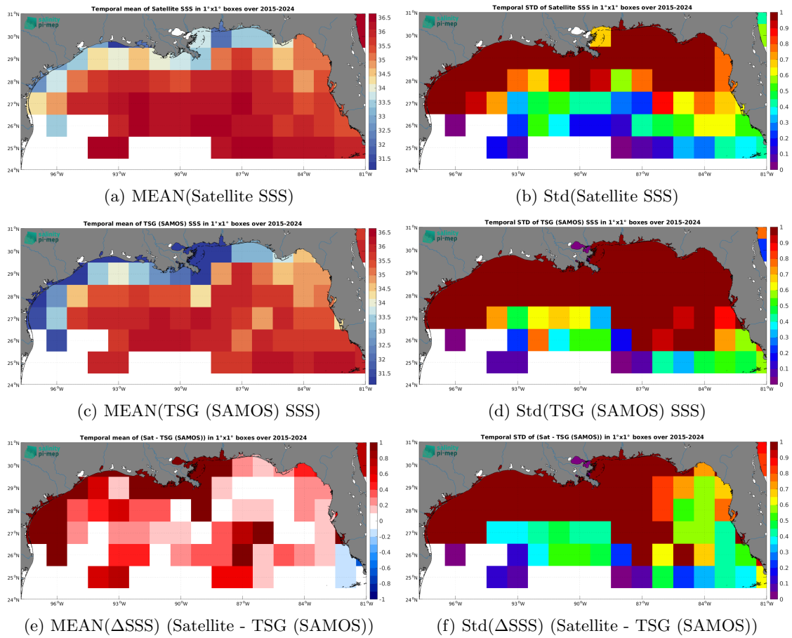
Figure 7: Temporal mean (left) and Std (right) of SSS from SMAP SSS L3 v5.0 - 8-Day running (JPL) (top), TSG (SAMOS) (middle), and of \Delta SSS (Satellite - TSG (SAMOS)). Only match-up pairs are used to generate these maps.
