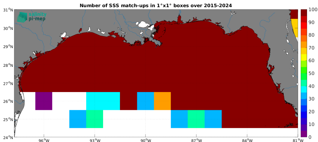
Figure 5: Number of SSS match-ups between TSG (SAMOS) SSS and the SMAP SSS L3 v5.0 - 8-Day running (JPL) SSS product for the Mississippi river plume Pi-MEP region over 1^\circ \times 1^\circ boxes and for the full satellite product period.
