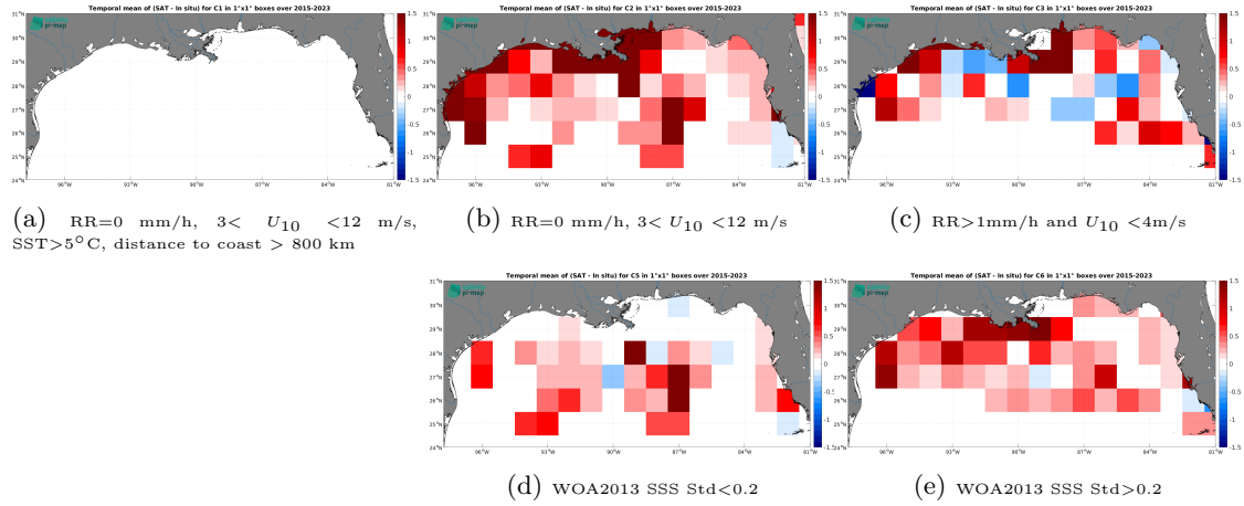
Figure 12: Temporal mean gridded over spatial boxes of size 1^{\circ}\times 1^{\circ} of \Delta\text{SSS} (SMAP SSS L3 v5.0 - 8-Day running (JPL) - TSG (SAMOS)) for 5 different subdatasets corresponding to:RR=0 mm/h, 3 < U_{10} < 12 m/s, SST >5^{\circ}\text{C} , distance to coast > 800 km (a), RR=0 mm/h, 3 < U_{10} < 12 m/s (b), RR >1 mm/h and U_{10} < 4 m/s (c), WOA2013 SSS Std <0.2 (d), WOA2013 SSS Std >0.2 (e).
