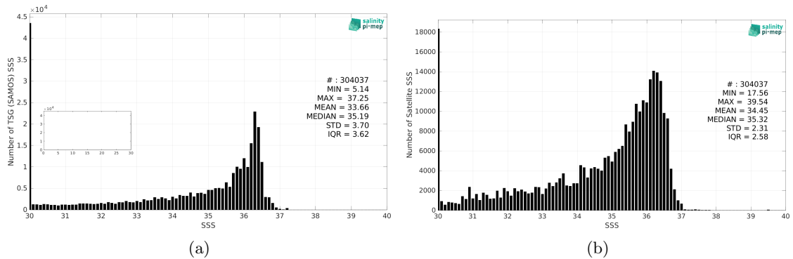
Figure 2: Histograms of SSS from TSG (SAMOS) (a) and SMAP SSS L3 v5.0 - 8-Day running (JPL) (b) considering all match-up pairs per bins of 0.1 over the Mississippi river plume Pi-MEP region and for the full satellite product period.
