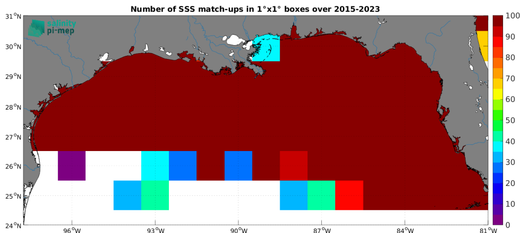
Figure 4: Number of SSS match-ups between TSG (SAMOS) SSS and the SMAP SSS L3 v5.0 - 8-Day running (JPL) SSS product for the Mississippi river plume Pi-MEP region over 1^\circ \times 1^\circ boxes and for the full satellite product period.
