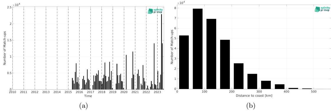
Figure 1: Number of match-ups between TSG (SAMOS) and SMAP SSS L3 v5.0 - 8-Day running (JPL) SSS as a function of time (a) and as function of the distance to coast (b) over the Mississippi river plume Pi-MEP region and for the full satellite product period.
