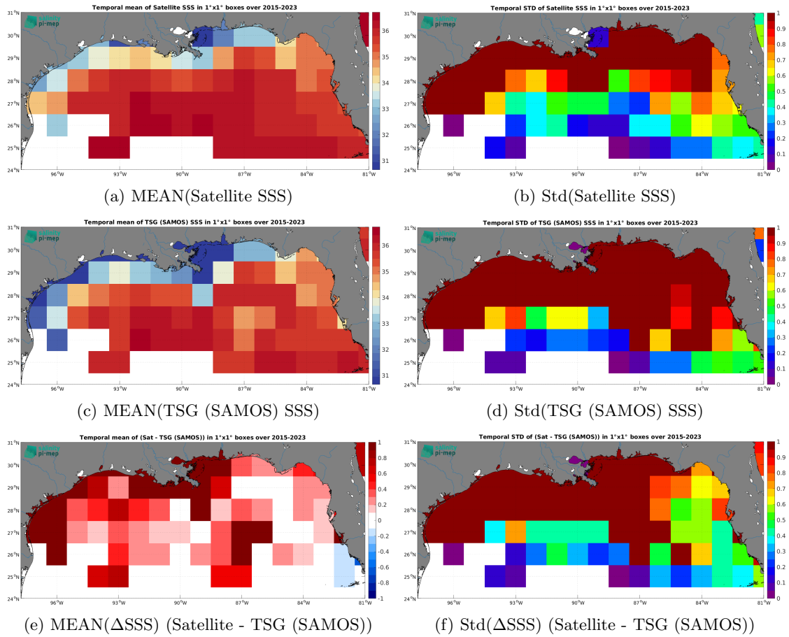
Figure 6: Temporal mean (left) and Std (right) of SSS from SMAP SSS L3 v5.0 - 8-Day running (JPL) (top), TSG (SAMOS) (middle), and of \Delta SSS (Satellite - TSG (SAMOS)). Only match-up pairs are used to generate these maps.
