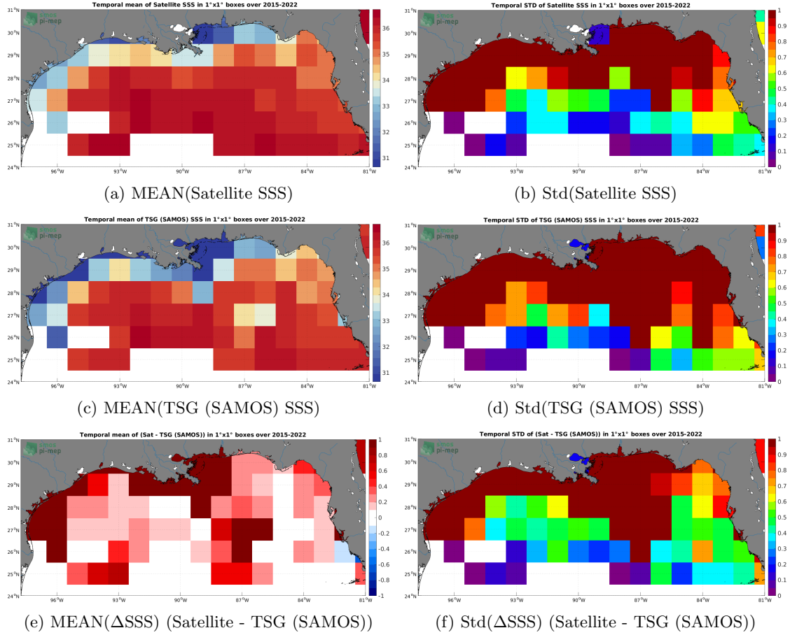
Figure 6: Temporal mean (left) and Std (right) of SSS from SMAP SSS L3 v5.0 - 8-Day running (JPL) (top), TSG (SAMOS) (middle), and of \Delta\text{SSS} (Satellite - TSG (SAMOS)). Only match-up pairs are used to generate these maps.
