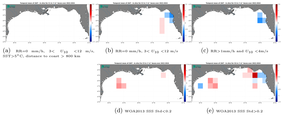
Figure 14: Temporal mean gridded over spatial boxes of size 1^\circ \times 1^\circ of \Delta SSS (SMAP SSS L3 v5.0 - 8-Day running (JPL) - Sairdrone) for 5 different subdatasets corresponding to:RR=0 mm/h, 3 < U_{10} < 12 m/s, SST > 5°C, distance to coast > 800 km (a), RR=0 mm/h, 3 < U_{10} < 12 m/s (b), RR > 1mm/h and U_{10} < 4 m/s (c), WOA2013 SSS Std < 0.2 (d), WOA2013 SSS Std > 0.2 (e).
