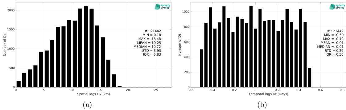
Figure 6: Histograms of the spatial (a) and temporal (b) lags between the location/time of the Sairdronc measurement and the date of the corresponding SMAP SSS L3 v5.0 - 8-Day running (JPL) SSS pixel.
