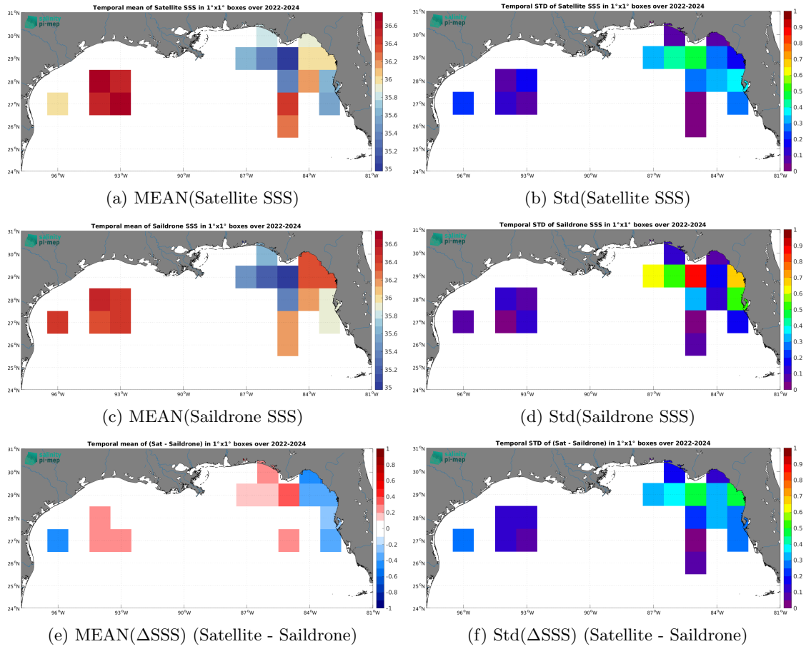
Figure 7: Temporal mean (left) and Std (right) of SSS from SMAP SSS L3 v5.0 - 8-Day running (JPL) (top), Saildrone (middle), and of \Delta SSS (Satellite - Saildrone). Only match-up pairs are used to generate these maps.
