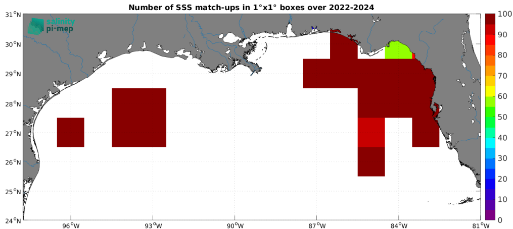
Figure 5: Number of SSS match-ups between Saildrone SSS and the SMAP SSS L3 v5.0 - 8-Day running (JPL) SSS product for the Mississippi river plume Pi-MEP region over 1^\circ \times 1^\circ boxes and for the full satellite product period.
