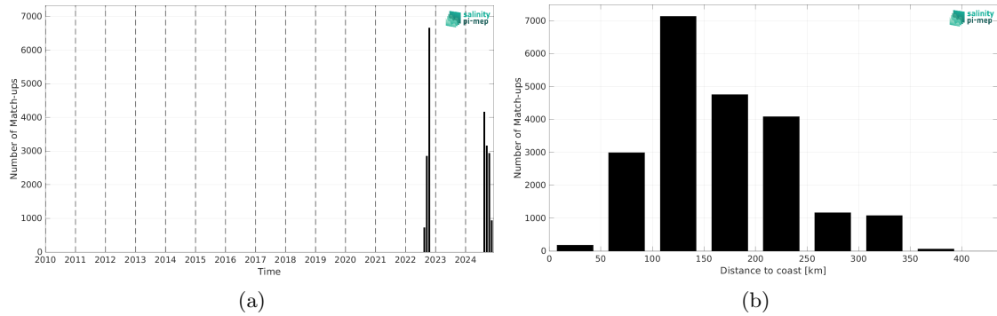
Figure 2: Number of match-ups between Saildrone and SMAP SSS L3 v5.0 - 8-Day running (JPL) SSS as a function of time (a) and as function of the distance to coast (b) over the Mississippi river plume Pi-MEP region and for the full satellite product period.
