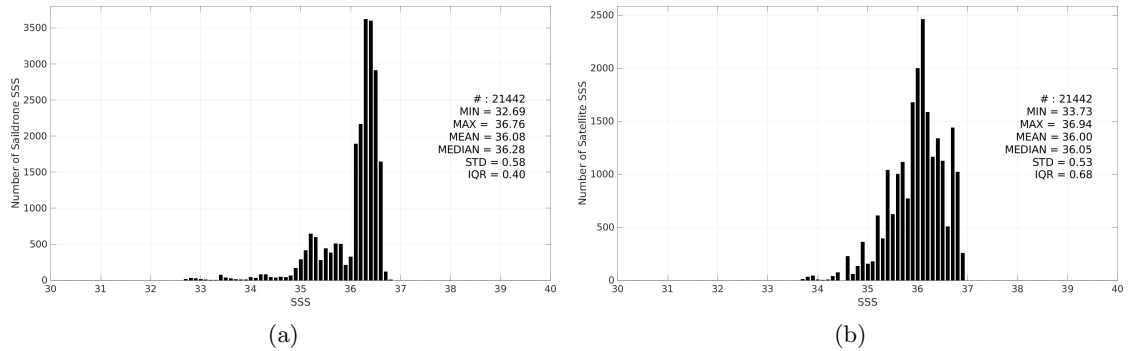
Figure 3: Histograms of SSS from Saildrone (a) and SMAP SSS L3 v5.0 - 8-Day running (JPL) (b) considering all match-up pairs per bins of 0.1 over the Mississippi river plume Pi-MEP region and for the full satellite product period.
