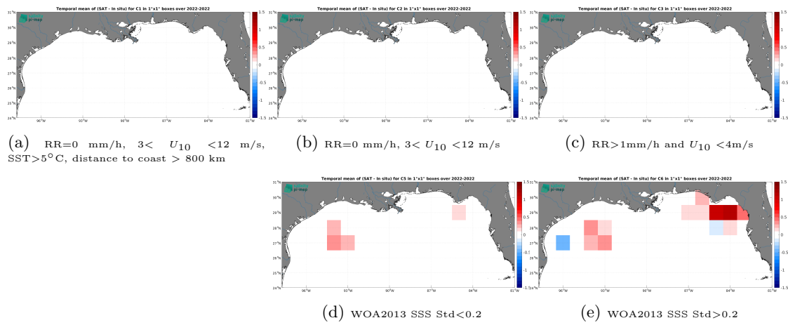
Figure 14: Temporal mean gridded over spatial boxes of size 1^\circ \times 1^\circ of \Delta SSS (SMAP SSS L3 v5.0 - 8-Day running (JPL) - Saildrone) for 5 different subdatasets corresponding to: RR=0 mm/h, 3 < U_{10} < 12 m/s, SST > 5°C, distance to coast > 800 km (a), RR=0 mm/h, 3 < U_{10} < 12 m/s (b), RR > 1mm/h and U_{10} < 4 m/s (c), WOA2013 SSS Std < 0.2 (d), WOA2013 SSS Std > 0.2 (e).
