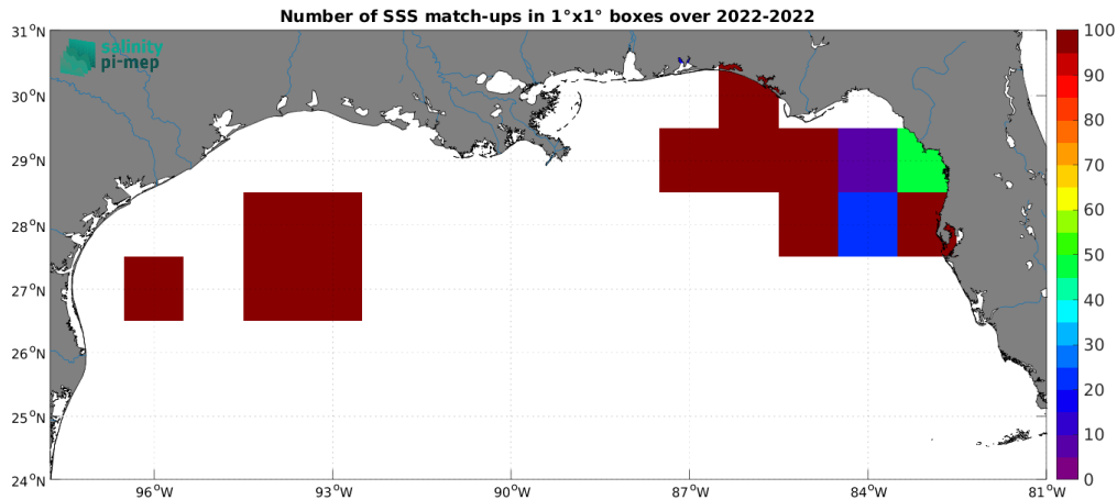
Figure 4: Number of SSS match-ups between Saildrone SSS and the SMAP SSS L3 v5.0 - 8-Day running (JPL) SSS product for the Mississippi river plume Pi-MEP region over 1^\circ \times 1^\circ boxes and for the full satellite product period.
