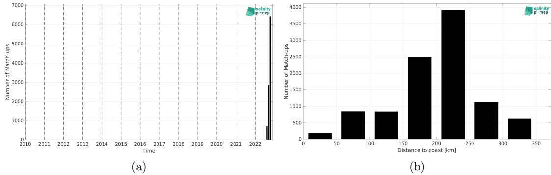
Figure 1: Number of match-ups between Sairdron and SMAP SSS L3 v5.0 - 8-Day running (JPL) SSS as a function of time (a) and as function of the distance to coast (b) over the Mississippi river plume Pi-MEP region and for the full satellite product period.
