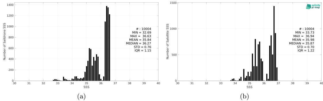
Figure 2: Histograms of SSS from Sairdron (a) and SMAP SSS L3 v5.0 - 8-Day running (JPL) (b) considering all match-up pairs per bins of 0.1 over the Mississippi river plume Pi-MEP region and for the full satellite product period.
