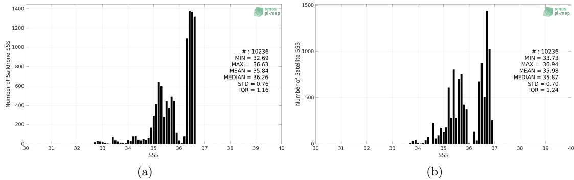
Figure 2: Histograms of SSS from Saildrone (a) and SMAP SSS L3 v5.0 - 8-Day running (JPL) (b) considering all match-up pairs per bins of 0.1 over the Mississippi river plume Pi-MEP region and for the full satellite product period.
