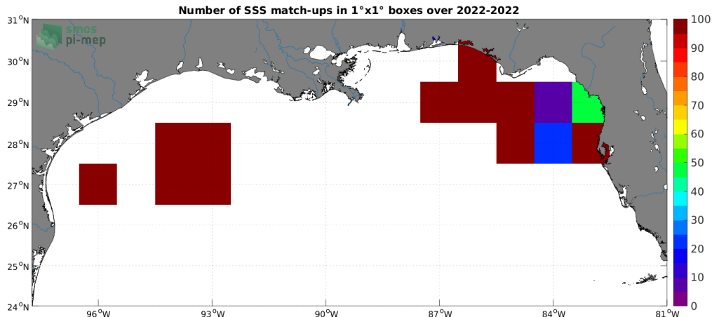
Figure 4: Number of SSS match-ups between Saildrone SSS and the SMAP SSS L3 v5.0 - 8-Day running (JPL) SSS product for the Mississippi river plume Pi-MEP region over 1^{\circ} \times 1^{\circ} boxes and for the full satellite product period.
