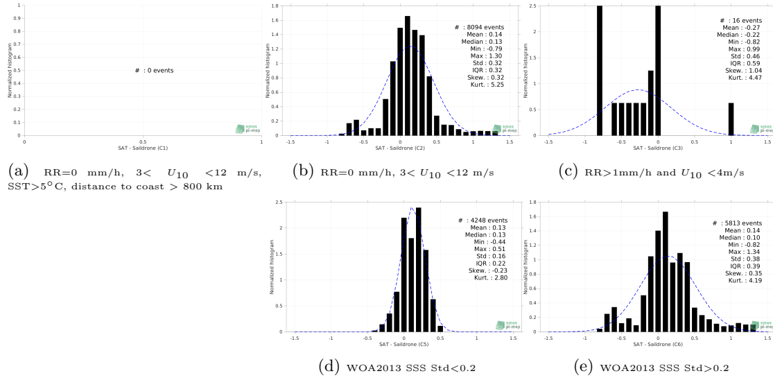
Figure 13: Normalized histogram of \Delta SSS (SMAP SSS L3 v5.0 - 8-Day running (JPL) - Saldrone) for 5 different subdatasets corresponding to: RR=0 mm/h, 3 < U_{10} < 12 m/s, SST > 5°C, distance to coast > 800 km (a), RR=0 mm/h, 3 < U_{10} < 12 m/s (b), RR > 1mm/h and U_{10} < 4 m/s (c), WOA2013 SSS Std < 0.2 (d), WOA2013 SSS Std > 0.2 (e).
