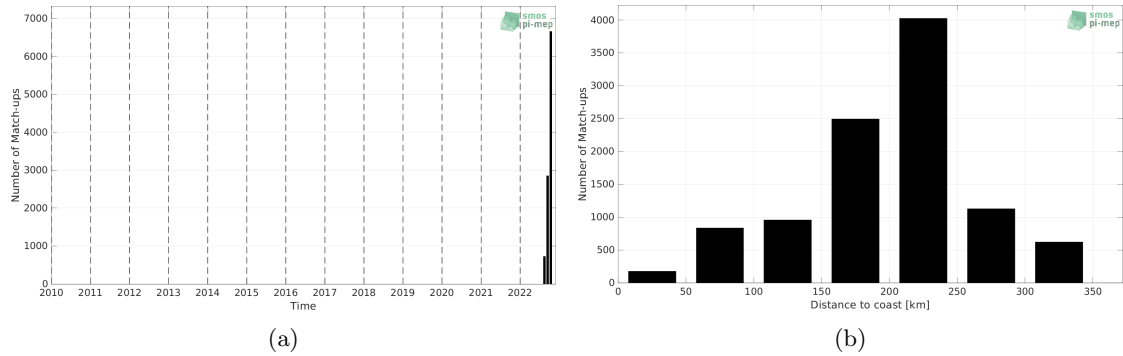
Figure 1: Number of match-ups between Saildrone and SMAP SSS L3 v5.0 - 8-Day running (JPL) SSS as a function of time (a) and as function of the distance to coast (b) over the Mississippi river plume Pi-MEP region and for the full satellite product period.
