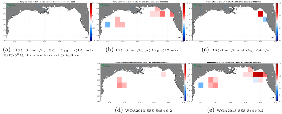
Figure 12: Temporal mean gridded over spatial boxes of size 1^{\circ}\times 1^{\circ} of \Delta\text{SSS} (SMAP SSS L3 v5.0 - 8-Day running (JPL) - Saifdrone) for 5 different subdatasets corresponding to:RR=0 mm/h, 3 < U_{10} < 12 m/s, SST >5^{\circ}\text{C} , distance to coast > 800 km (a), RR=0 mm/h, 3 < U_{10} < 12 m/s (b), RR >1 mm/h and U_{10} < 4 m/s (c), WOA2013 SSS Std <0.2 (d), WOA2013 SSS Std >0.2 (e).
