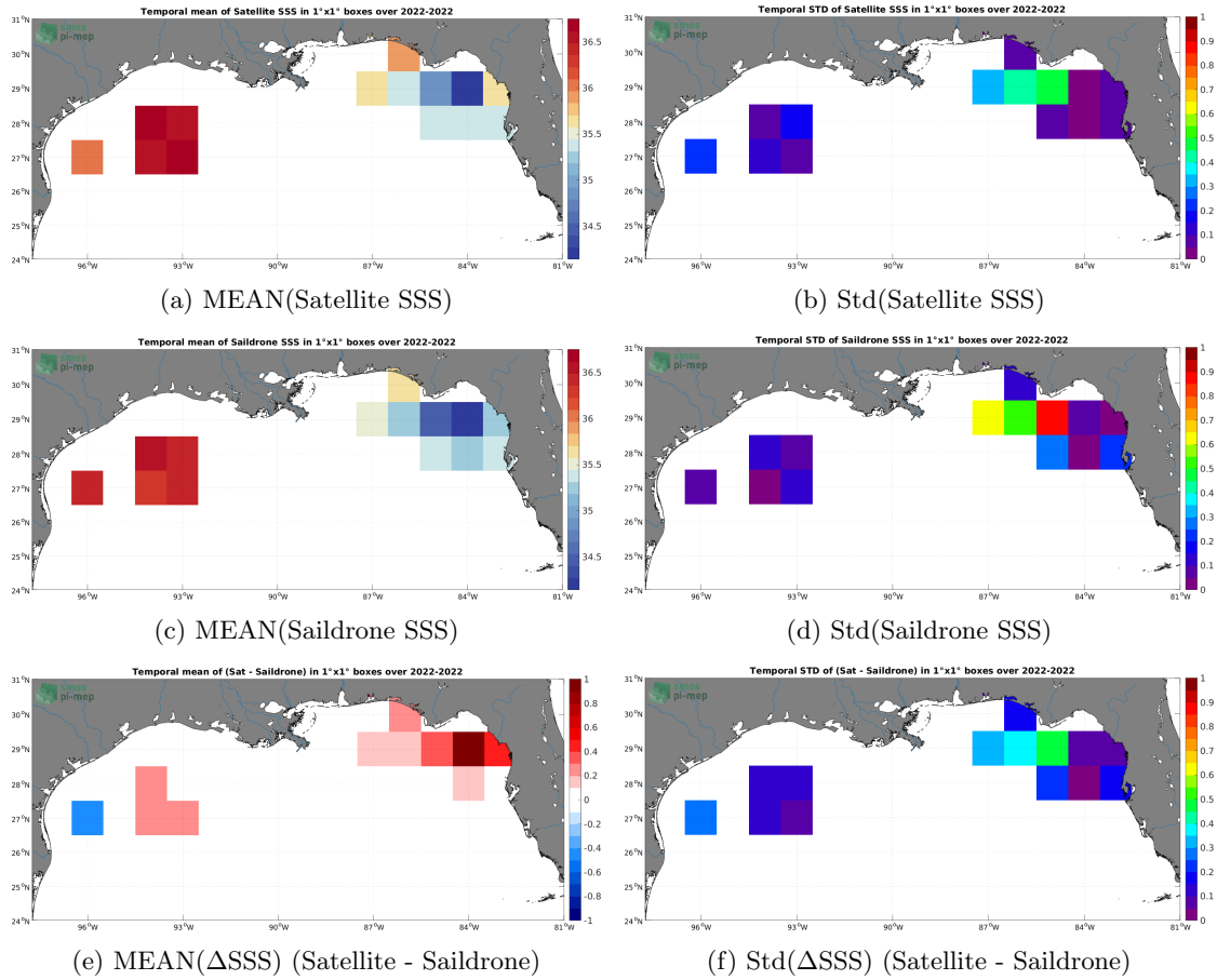
Figure 6: Temporal mean (left) and Std (right) of SSS from SMAP SSS L3 v5.0 - 8-Day running (JPL) (top), Saildrone (middle), and of \Delta SSS (Satellite - Saildrone). Only match-up pairs are used to generate these maps.
