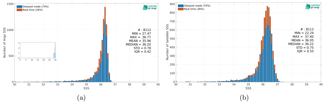
Figure 2: Histograms of SSS from Argo (a) and SMAP SSS L3 v5.0 - 8-Day running (JPL) (b) considering all match-up pairs per bins of 0.1 over the Mississippi river plume Pi-MEP region and for the full satellite product period.
