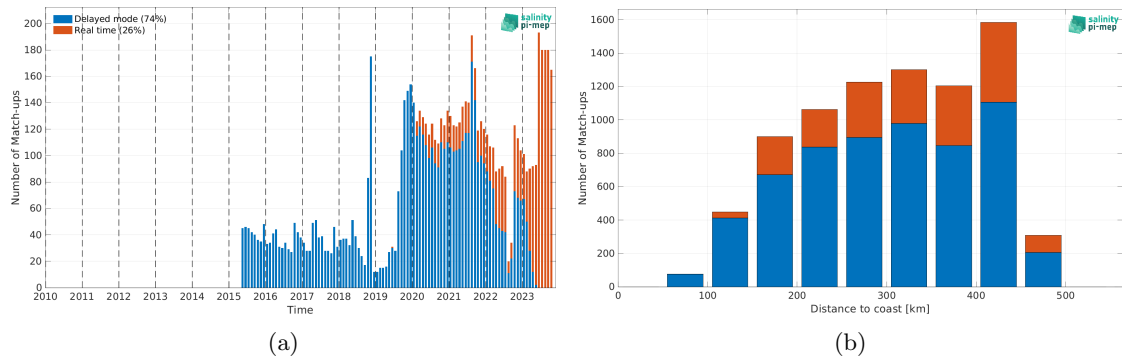
Figure 1: Number of match-ups between Argo and SMAP SSS L3 v5.0 - 8-Day running (JPL) SSS as a function of time (a) and as function of the distance to coast (b) over the Mississippi river plume Pi-MEP region and for the full satellite product period.
