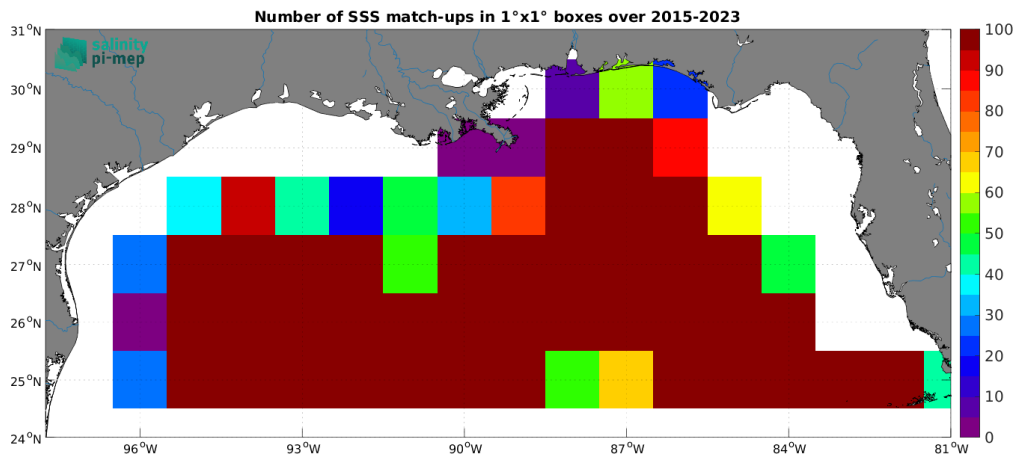
Figure 4: Number of SSS match-ups between Argo SSS and the SMAP SSS L3 v5.0 - 8-Day running (JPL) SSS product for the Mississippi river plume Pi-MEP region over 1^{\circ} \times 1^{\circ} boxes and for the full satellite product period.
