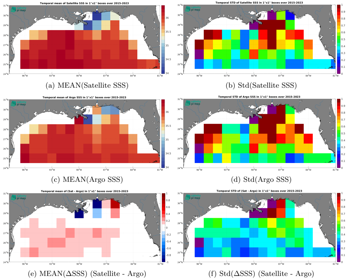
Figure 6: Temporal mean (left) and Std (right) of SSS from SMAP SSS L3 v5.0 - 8-Day running (JPL) (top), Argo (middle), and of \Delta SSS (Satellite - Argo). Only match-up pairs are used to generate these maps.
