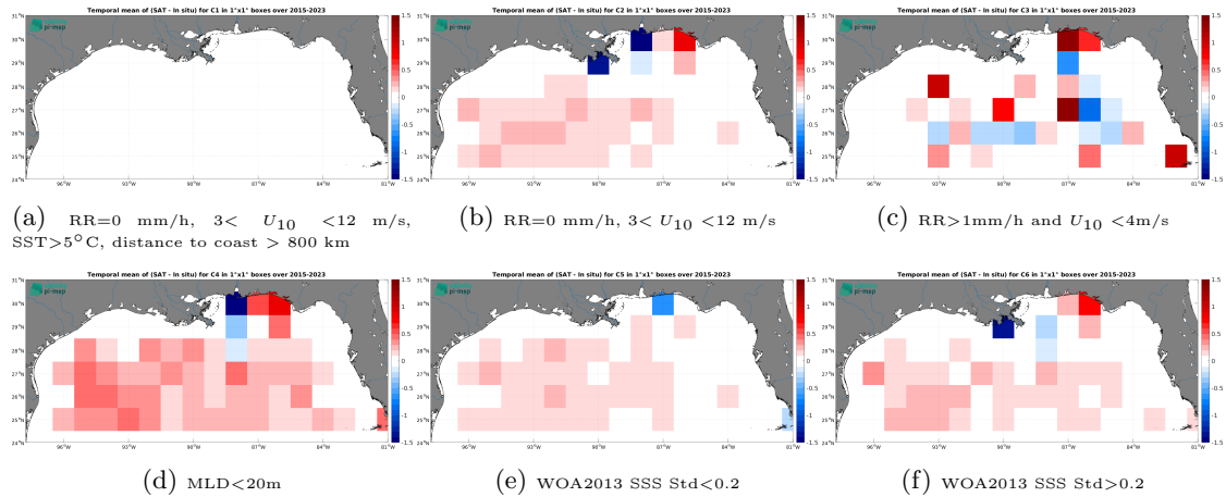
Figure 12: Temporal mean gridded over spatial boxes of size 1^{\circ}\times 1^{\circ} of \Delta\text{SSS} (SMAP SSS L3 v5.0 - 8-Day running (JPL) - Argo) for 6 different subdatasets corresponding to:RR=0 mm/h, 3 < U_{10} < 12 m/s, SST > 5^{\circ}\text{C} , distance to coast > 800 km (a), RR=0 mm/h, 3 < U_{10} < 12 m/s (b), RR > 1 mm/h and U_{10} < 4 m/s (c),MLD < 20 m (d),WOA2013 SSS Std < 0.2 (e),WOA2013 SSS Std > 0.2 (f).
