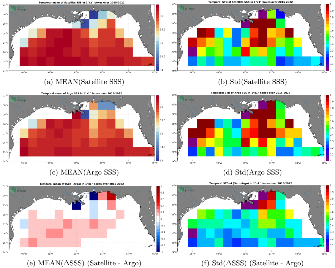
Figure 6: Temporal mean (left) and Std (right) of SSS from SMAP SSS L3 v5.0 - 8-Day running (JPL) (top), Argo (middle), and of \Delta\text{SSS} (Satellite - Argo). Only match-up pairs are used to generate these maps.
