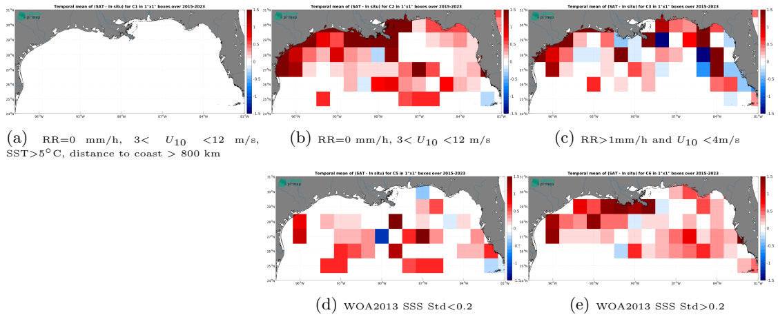
Figure 14: Temporal mean gridded over spatial boxes of size 1^\circ \times 1^\circ of \Delta SSS (SMAP SSS L3 v5.0 - Monthly (JPL) - TSG (SAMOS)) for 5 different subdatasets corresponding to:RR=0 mm/h, 3 < U_{10} < 12 m/s, SST>5°C, distance to coast > 800 km (a), RR=0 mm/h, 3 < U_{10} < 12 m/s (b), RR>1mm/h and U_{10} < 4 m/s (c), WOA2013 SSS Std<0.2 (d), WOA2013 SSS Std>0.2 (e).
