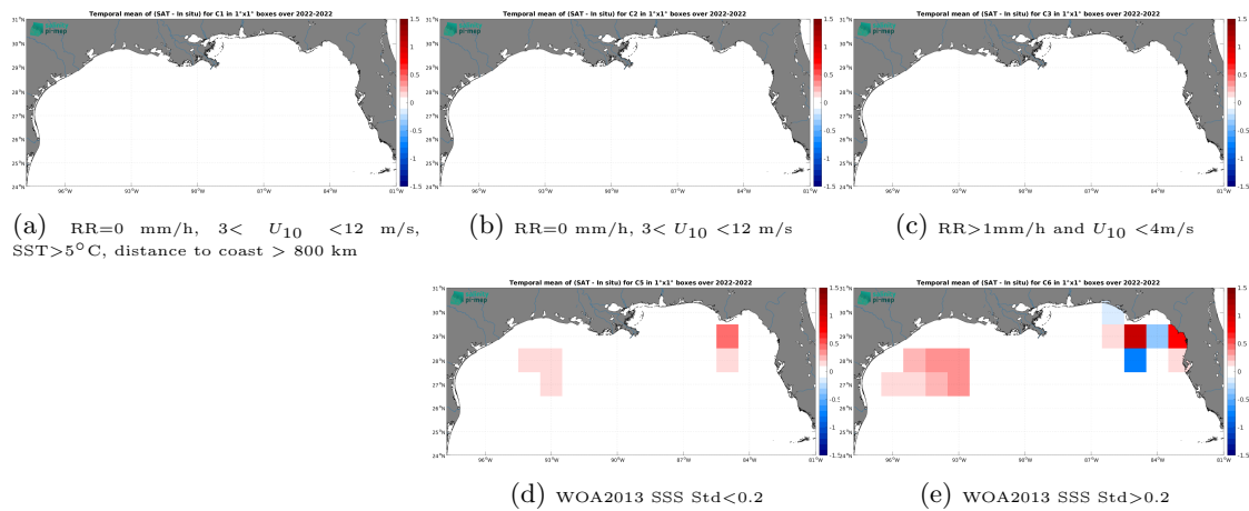
Figure 14: Temporal mean gridded over spatial boxes of size 1^\circ \times 1^\circ of \Delta SSS (SMAP SSS L3 v5.0 - Monthly (JPL) - Sairdrone) for 5 different subdatasets corresponding to: RR=0 mm/h, 3 < U_{10} < 12 m/s, SST > 5°C, distance to coast > 800 km (a), RR=0 mm/h, 3 < U_{10} < 12 m/s (b), RR > 1mm/h and U_{10} < 4 m/s (c), WOA2013 SSS Std < 0.2 (d), WOA2013 SSS Std > 0.2 (e).
