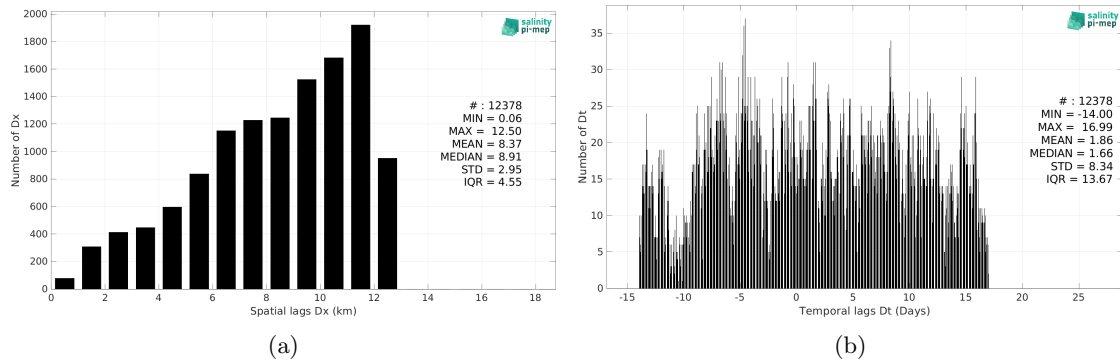
Figure 6: Histograms of the spatial (a) and temporal (b) lags between the location/time of the Saildrone measurement and the date of the corresponding SMAP SSS L3 v5.0 - Monthly (JPL) SSS pixel.
