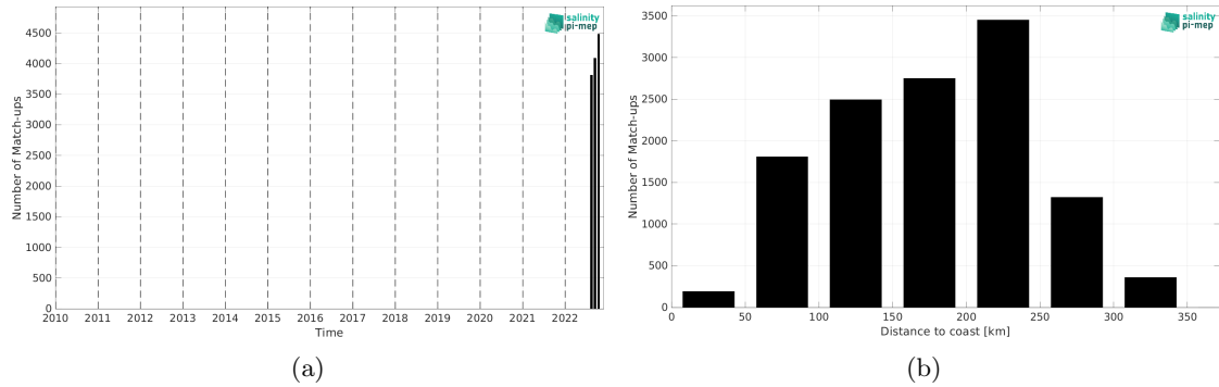
Figure 2: Number of match-ups between Saildrone and SMAP SSS L3 v5.0 - Monthly (JPL) SSS as a function of time (a) and as function of the distance to coast (b) over the Mississippi river plume Pi-MEP region and for the full satellite product period.
