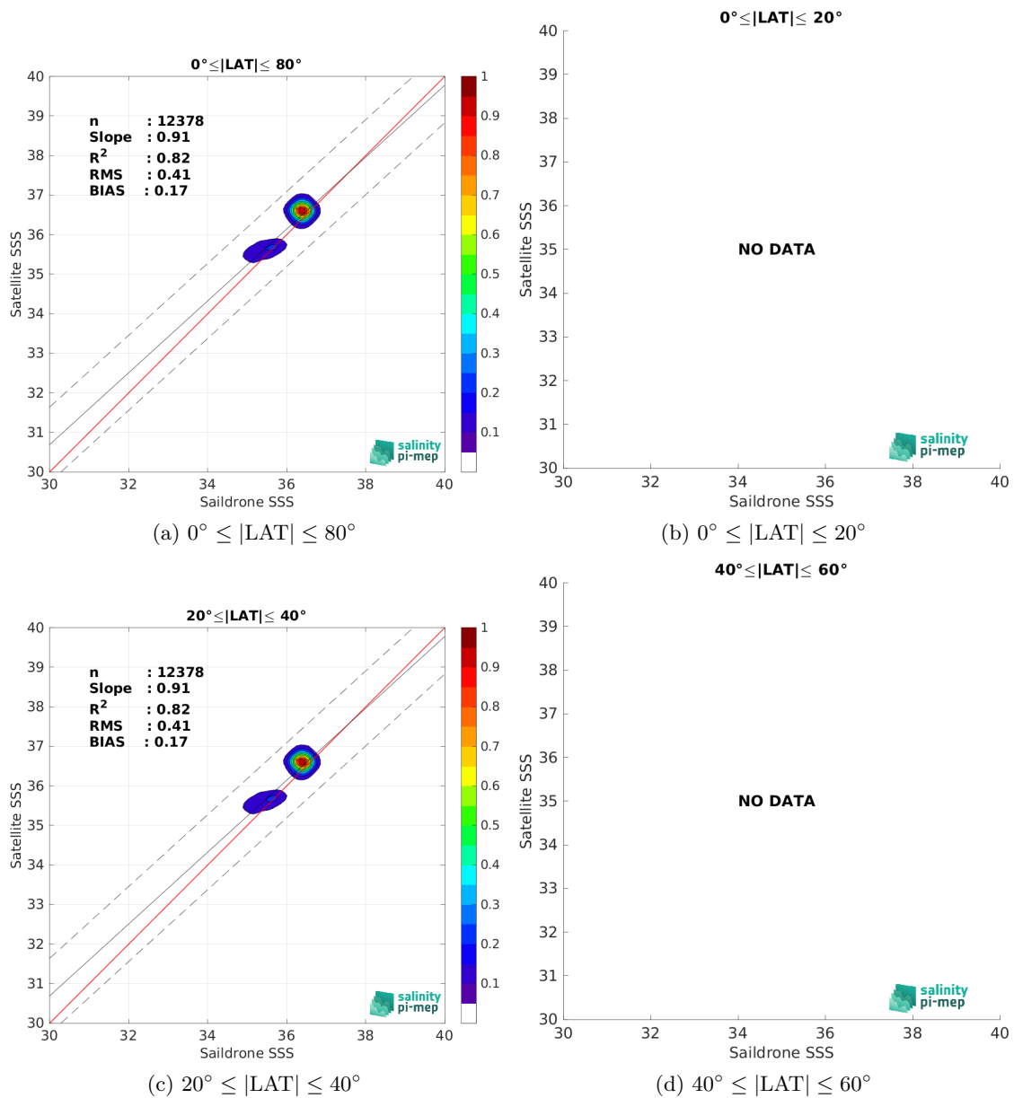
Figure 10: Contour maps of the concentration of SMAP SSS L3 v5.0 - Monthly (JPL) SSS (y-axis) versus Saildrone SSS (x-axis) at match-up pairs for different latitude bands. For each plot, the red line shows x=y . The black thin and dashed lines indicate a linear fit through the data cloud and the \pm 95\% confidence levels, respectively. The number match-up pairs n , the slope and R^2 coefficient of the linear fit, the root mean square (RMS) and the mean bias between satellite and in situ data are indicated for each latitude band in each plots.
