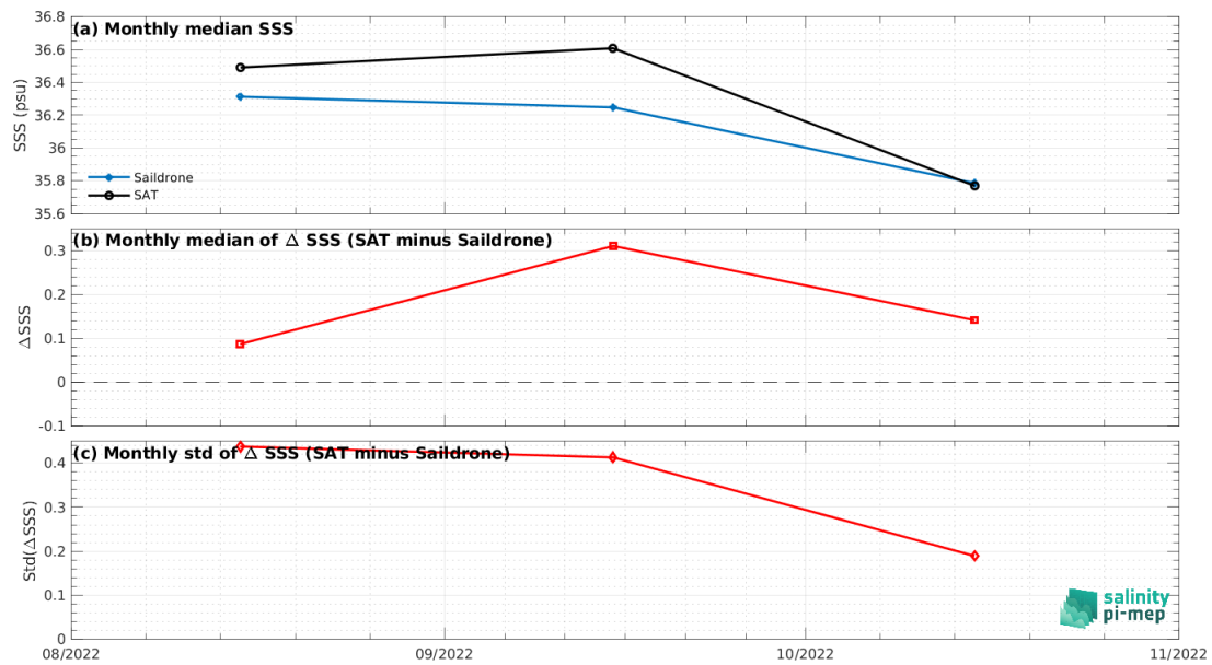
Figure 8: Time series of the monthly median SSS (top), median of \Delta SSS (Satellite - Sairdrone) and Std of \Delta SSS (Satellite - Sairdrone) over the Mississippi river plume Pi-MEP region considering all match-ups collected by the Pi-MEP.
