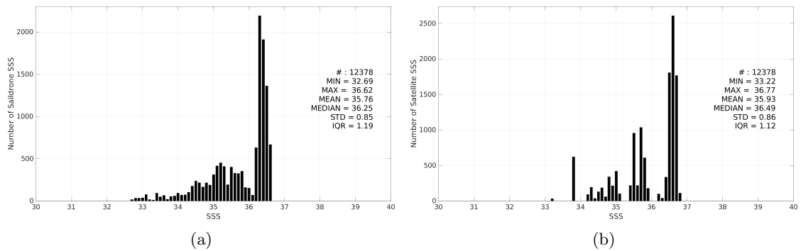
Figure 3: Histograms of SSS from Saildrone (a) and SMAP SSS L3 v5.0 - Monthly (JPL) (b) considering all match-up pairs per bins of 0.1 over the Mississippi river plume Pi-MEP region and for the full satellite product period.
