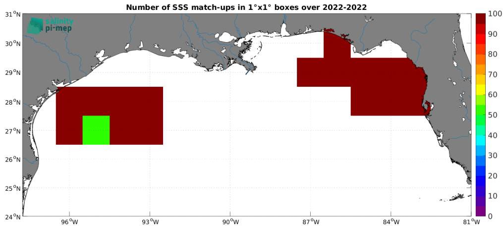
Figure 5: Number of SSS match-ups between Saildrone SSS and the SMAP SSS L3 v5.0 - Monthly (JPL) SSS product for the Mississippi river plume Pi-MEP region over 1^\circ \times 1^\circ boxes and for the full satellite product period.
