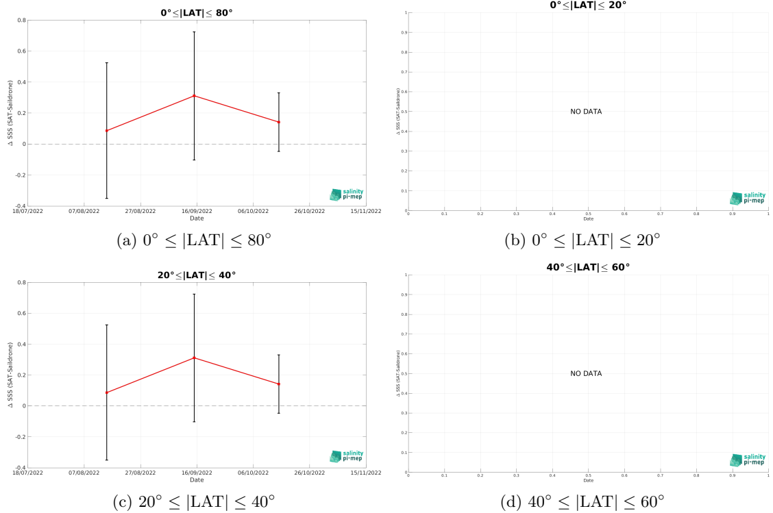
Figure 11: Monthly median (red curves) of \Delta SSS (Satellite - Sairdron) and \pm 1 Std (black vertical thick bars) as function of time for all the collected Pi-MEP match-up pairs estimated over the Mississippi river plume Pi-MEP region and for the full satellite product period are shown for different latitude bands: (a) 80^\circ\text{S}-80^\circ\text{N} , (b) 20^\circ\text{S}-20^\circ\text{N} , (c) 40^\circ\text{S}-20^\circ\text{S} and 20^\circ\text{N}-40^\circ\text{N} and (d) 60^\circ\text{S}-40^\circ\text{S} and 40^\circ\text{N}-60^\circ\text{N} .
