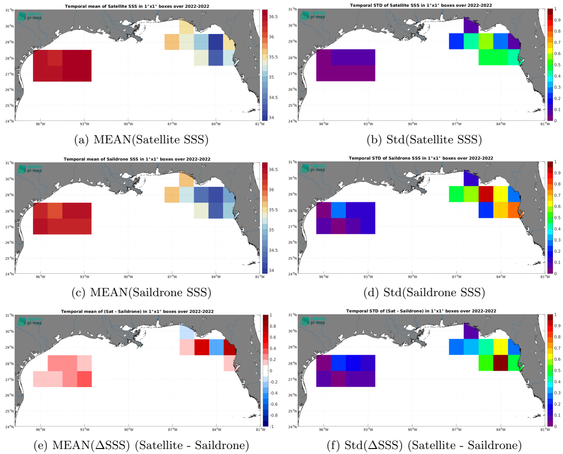
Figure 7: Temporal mean (left) and Std (right) of SSS from SMAP SSS L3 v5.0 - Monthly (JPL) (top), Saildrone (middle), and of \Delta SSS (Satellite - Saildrone). Only match-up pairs are used to generate these maps.
