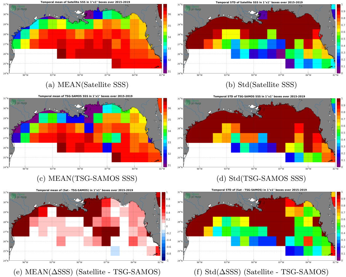
Figure 6: Temporal mean (left) and Std (right) of SSS from SMAP-L3-JPL-V4.2-8DAY-RUNNING-60KM (top), TSG-SAMOS (middle), and of \Delta\text{SSS} (Satellite - TSG-SAMOS). Only match-up pairs are used to generate these maps.
