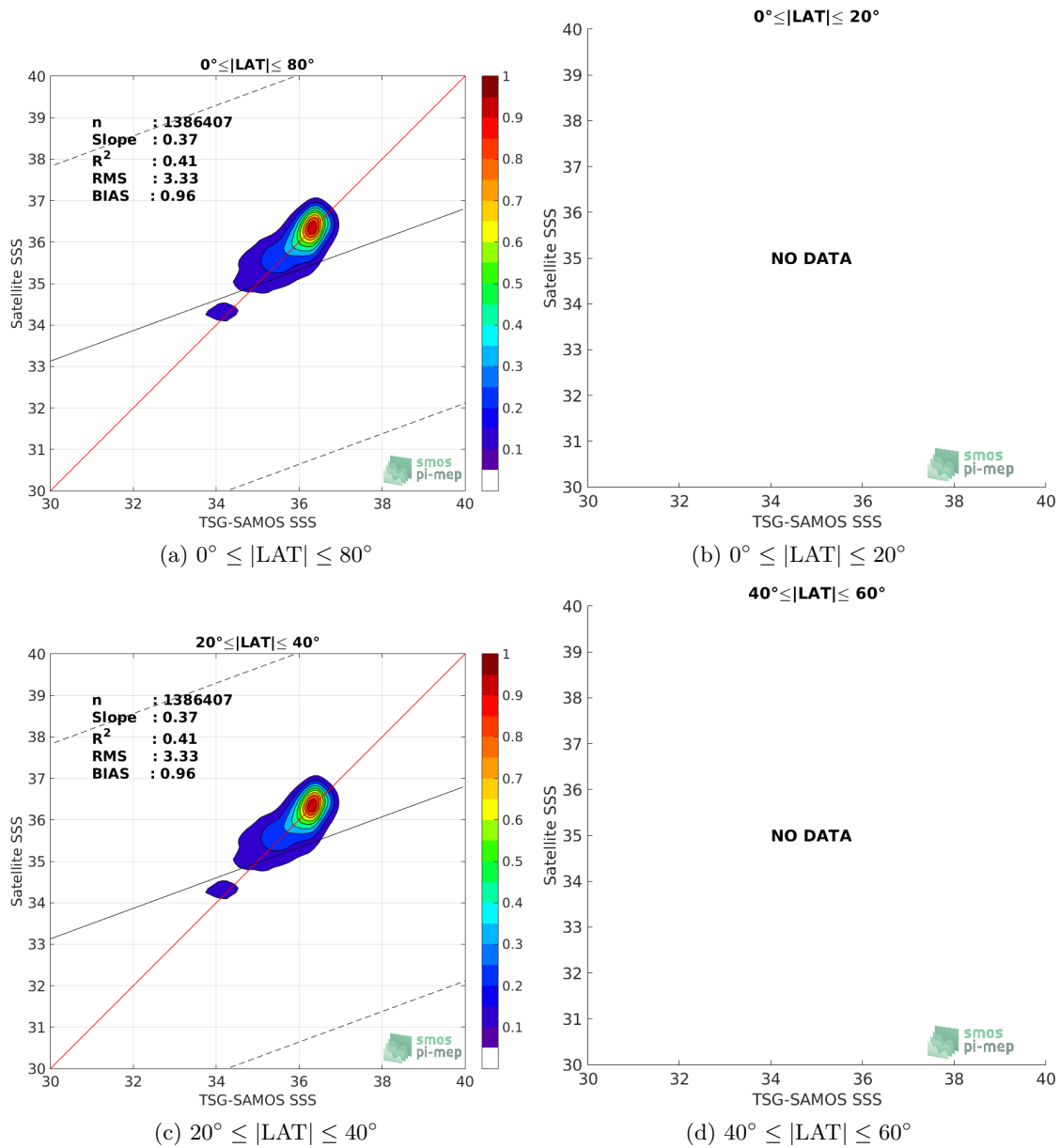
Figure 9: Contour maps of the concentration of SMAP-L3-JPL-V4.2-8DAY-RUNNING-60KM SSS (y-axis) versus TSG-SAMOS SSS (x-axis) at match-up pairs for different latitude bands. For each plot, the red line shows x=y . The black thin and dashed lines indicate a linear fit through the data cloud and the \pm 95\% confidence levels, respectively. The number match-up pairs n , the slope and R^2 coefficient of the linear fit, the root mean square (RMS) and the mean bias between satellite and in situ data are indicated for each latitude band in each plots.
