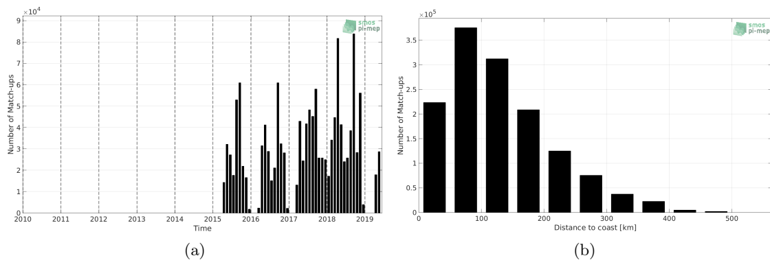
Figure 1: Number of match-ups between TSG-SAMOS and SMAP-L3-JPL-V4.2-8DAY-RUNNING-60KM SSS as a function of time (a) and as function of the distance to coast (b) over the Mississippi river plume Pi-MEP region and for the full satellite product period.
