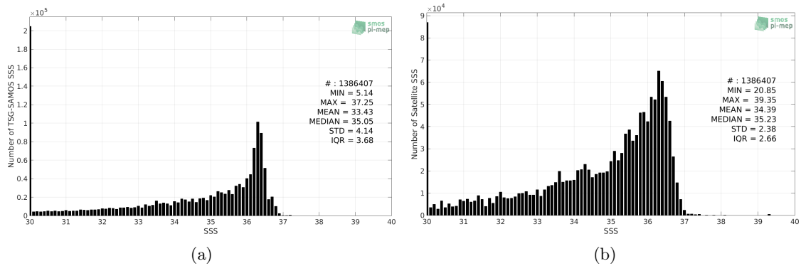
Figure 2: Histograms of SSS from TSG-SAMOS (a) and SMAP-L3-JPL-V4.2-8DAY-RUNNING-60KM (b) considering all match-up pairs per bins of 0.1 over the Mississippi river plume Pi-MEP region and for the full satellite product period.
