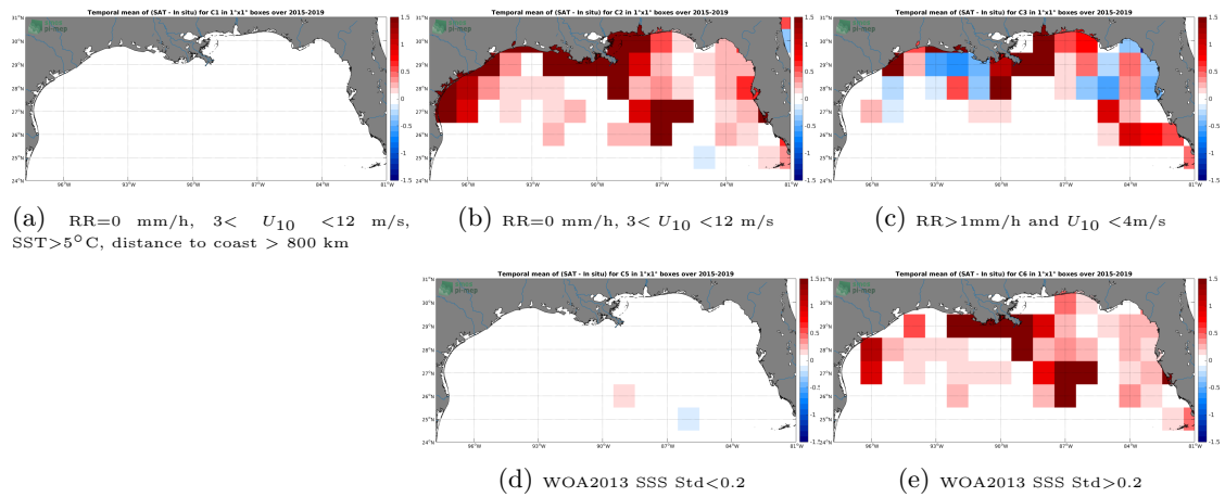
Figure 12: Temporal mean gridded over spatial boxes of size 1^\circ \times 1^\circ of \Delta SSS (SMAP-L3-JPL-V4.2-8DAY-RUNNING-60KM - TSG-SAMOS) for 5 different subdatasets corresponding to:RR=0 mm/h, 3 < U_{10} < 12 m/s, SST >5^\circ C, distance to coast > 800 km (a), RR=0 mm/h, 3 < U_{10} < 12 m/s (b), RR >1 mm/h and U_{10} < 4 m/s (c), WOA2013 SSS Std <0.2 (d), WOA2013 SSS Std >0.2 (e).
