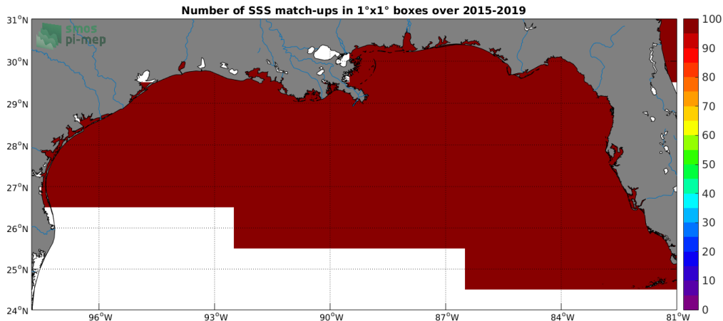
Figure 4: Number of SSS match-ups between TSG-SAMOS SSS and the SMAP-L3-JPL-V4.2-8DAY-RUNNING-60KM SSS product for the Mississippi river plume Pi-MEP region over 1^\circ \times 1^\circ boxes and for the full satellite product period.
