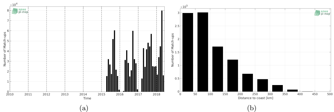
Figure 1: Number of match-ups between TSG-SAMOS and SMAP-L3-JPL-V4-8DAY-RUNNING-60KM SSS as a function of time (a) and as function of the distance to coast (b) over the Mississippi river plume Pi-MEP region and for the full satellite product period.
