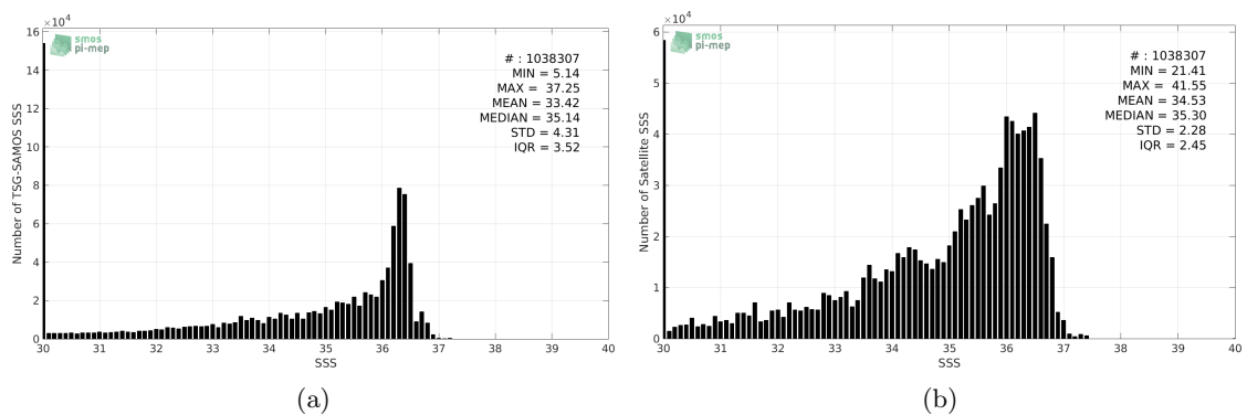
Figure 2: Histograms of SSS from TSG-SAMOS (a) and SMAP-L3-JPL-V4-8DAY-RUNNING-60KM (b) considering all match-up pairs per bins of 0.1 over the Mississippi river plume Pi-MEP region and for the full satellite product period.
