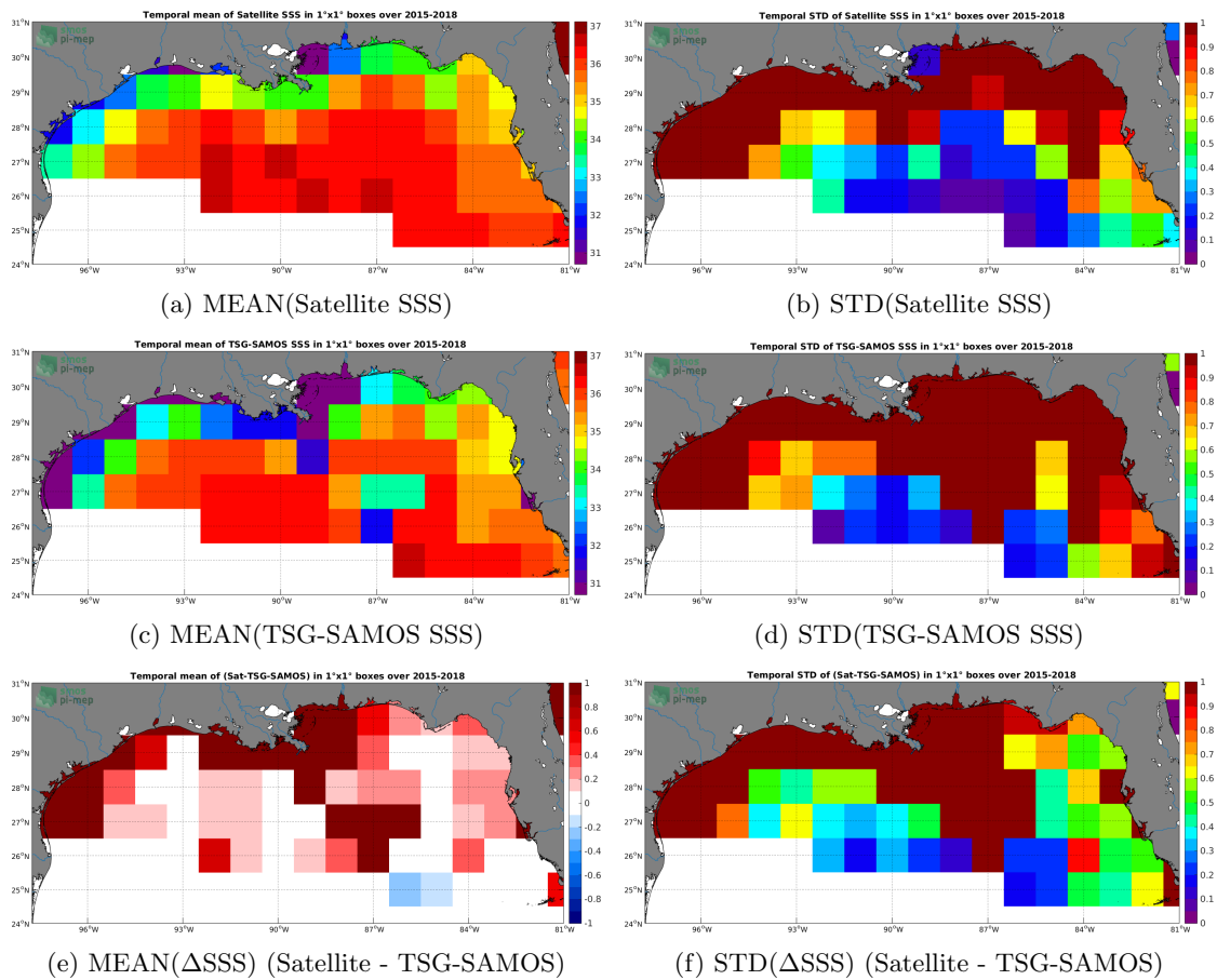
Figure 6: Temporal mean (left) and STD (right) of SSS from SMAP-L3-JPL-V4-8DAY-RUNNING-60KM (top), TSG-SAMOS (middle), and of \Delta SSS (Satellite - TSG-SAMOS). Only match-up pairs are used to generate these maps.
