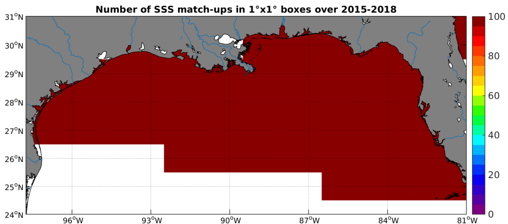
Figure 4: Number of SSS match-ups between TSG-SAMOS SSS and the SMAP-L3-JPL-V4-8DAY-RUNNING-60KM SSS product for the Mississippi river plume Pi-MEP region over 1^\circ \times 1^\circ boxes and for the full satellite product period.
