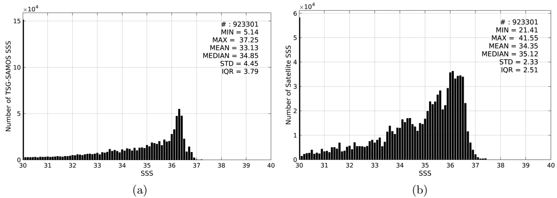
Figure 2: Histograms of SSS from TSG-SAMOS (a) and SMAP-L3-JPL-V4-8DAY-RUNNING-60KM (b) considering all match-up pairs per bins of 0.1 over the Mississippi river plume Pi-MEP region and for the full satellite product period.
