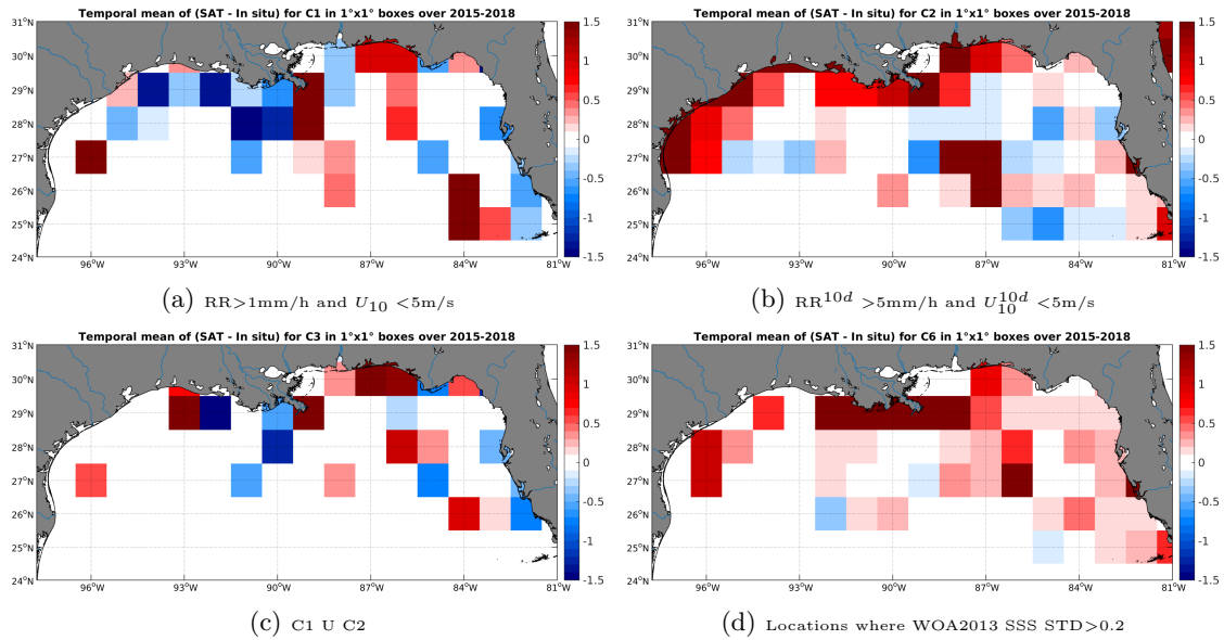
Figure 12: Temporal mean gridded over spatial boxes of size 1^\circ \times 1^\circ of \Delta SSS (SMAP-L3-JPL-V4-8DAY-RUNNING-60KM - TSG-SAMOS) for 4 different subdatasets corresponding to:RR > 1 mm/h and U_{10} < 5 m/s (a), RR^{10d} > 5 mm/h and U_{10}^{10d} < 5 m/s (b), C1 U C2 (c),Locations where WOA2013 SSS STD > 0.2 (d).
