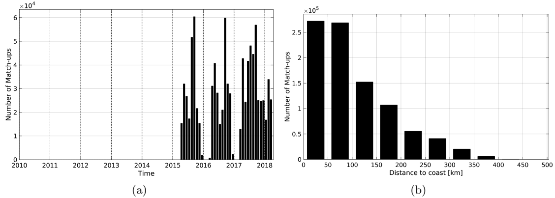
Figure 1: Number of match-ups between TSG-SAMOS and SMAP-L3-JPL-V4-8DAY-RUNNING-60KM SSS as a function of time (a) and as function of the distance to coast (b) over the Mississippi river plume Pi-MEP region and for the full satellite product period.
