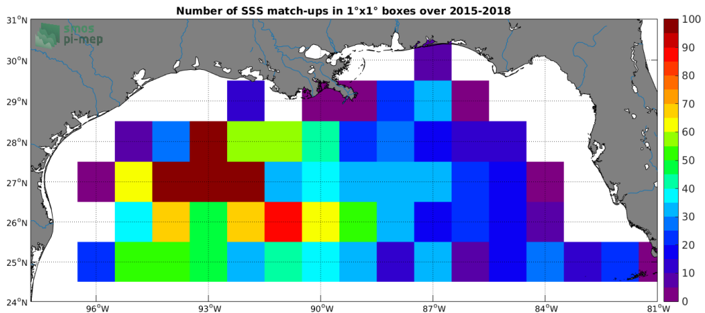
Figure 4: Number of SSS match-ups between Argo SSS and the SMAP-L3-JPL-V4-8DAY-RUNNING-60KM SSS product for the Mississippi river plume Pi-MEP region over 1°x1° boxes and for the full satellite product period.
