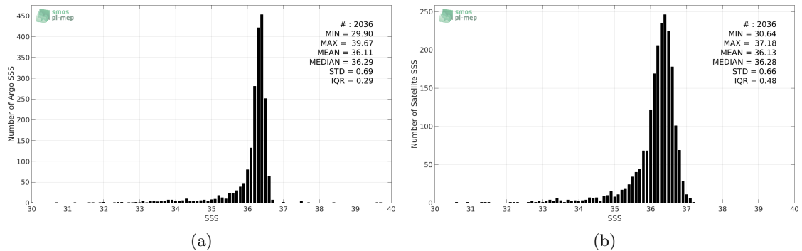
Figure 2: Histograms of SSS from Argo (a) and SMAP-L3-JPL-V4-8DAY-RUNNING-60KM (b) considering all match-up pairs per bins of 0.1 over the Mississippi river plume Pi-MEP region and for the full satellite product period.
