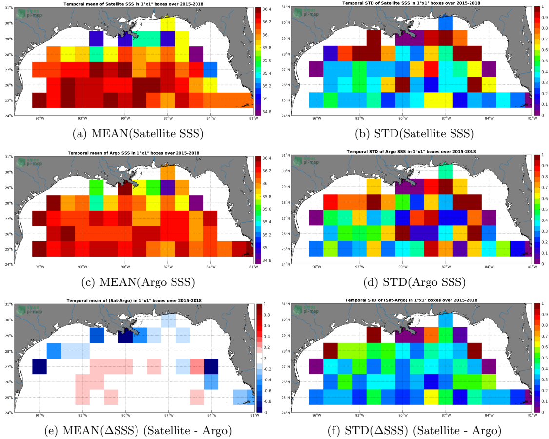
Figure 6: Temporal mean (left) and STD (right) of SSS from SMAP-L3-JPL-V4-8DAY-RUNNING-60KM (top), Argo (middle), and of \Delta SSS (Satellite - Argo). Only match-up pairs are used to generate these maps.
