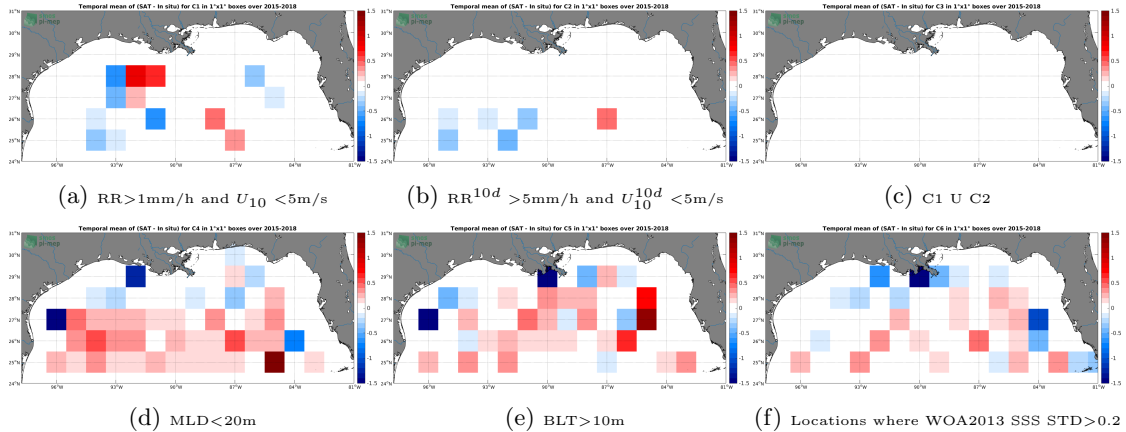
Figure 12: Temporal mean gridded over spatial boxes of size 1^\circ \times 1^\circ of \Delta\text{SSS} (SMAP-L3-JPL-V4-8DAY-RUNNING-60KM - Argo) for 6 different subdatasets corresponding to:RR >1\text{mm/h} and U_{10} < 5\text{m/s} (a), RR^{10d} > 5\text{mm/h} and U_{10}^{10d} < 5\text{m/s} (b), C1 U C2 (c),MLD <20\text{m} (d),BLT >10\text{m} (e),Locations where WOA2013 SSS STD >0.2 (f).
