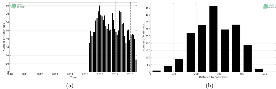
Figure 1: Number of match-ups between Argo and SMAP-L3-JPL-V4-8DAY-RUNNING-60KM SSS as a function of time (a) and as function of the distance to coast (b) over the Mississippi river plume Pi-MEP region and for the full satellite product period.
