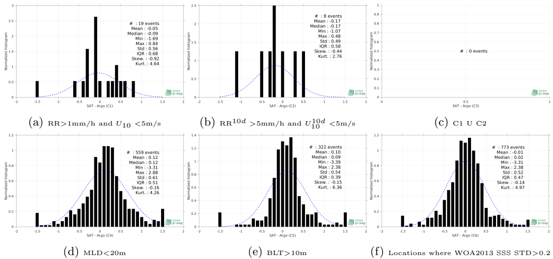
Figure 13: Normalized histogram of \Delta\text{SSS} (SMAP-L3-JPL-V4-8DAY-RUNNING-60KM - Argo) for 6 different subdatasets corresponding to: RR >1\text{mm/h} and U_{10} < 5\text{m/s} (a), RR^{10d} > 5\text{mm/h} and U_{10}^{10d} < 5\text{m/s} (b), C1 U C2 (c),MLD <20\text{m} (d),BLT >10\text{m} (e),Locations where WOA2013 SSS STD >0.2 (f).
