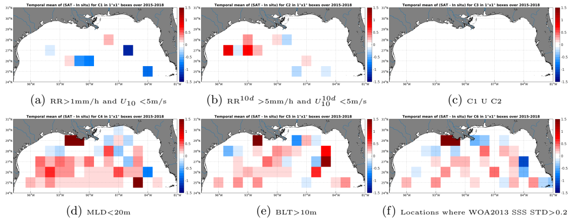
Figure 12: Temporal mean gridded over spatial boxes of size 1^\circ \times 1^\circ of \Delta SSS (SMAP-L3-JPL-V4-8DAY-RUNNING-60KM - Argo) for 6 different subdatasets corresponding to: RR > 1\text{mm/h} and U_{10} < 5\text{m/s} (a), RR^{10d} > 5\text{mm/h} and U_{10}^{10d} < 5\text{m/s} (b), C1 U C2 (c), MLD < 20\text{m} (d), BLT > 10\text{m} (e), Locations where WOA2013 SSS STD > 0.2 (f).
