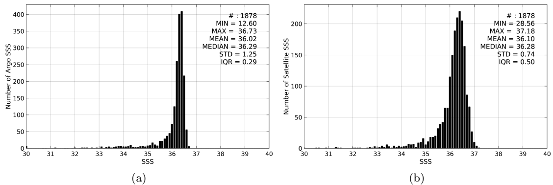
Figure 2: Histograms of SSS from Argo (a) and SMAP-L3-JPL-V4-8DAY-RUNNING-60KM (b) considering all match-up pairs per bins of 0.1 over the Mississippi river plume Pi-MEP region and for the full satellite product period.
