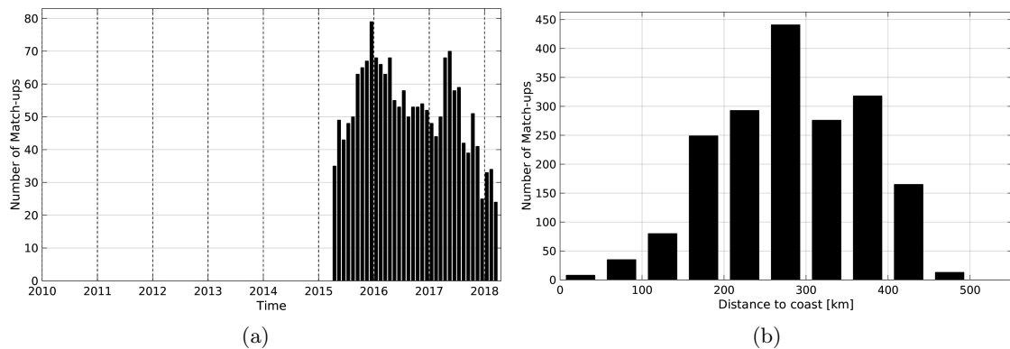
Figure 1: Number of match-ups between Argo and SMAP-L3-JPL-V4-8DAY-RUNNING-60KM SSS as a function of time (a) and as function of the distance to coast (b) over the Mississippi river plume Pi-MEP region and for the full satellite product period.
