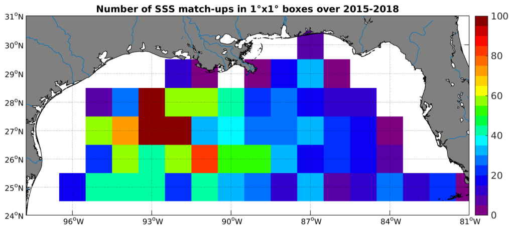
Figure 4: Number of SSS match-ups between Argo SSS and the SMAP-L3-JPL-V4-8DAY-RUNNING-60KM SSS product for the Mississippi river plume Pi-MEP region over 1^\circ \times 1^\circ boxes and for the full satellite product period.
