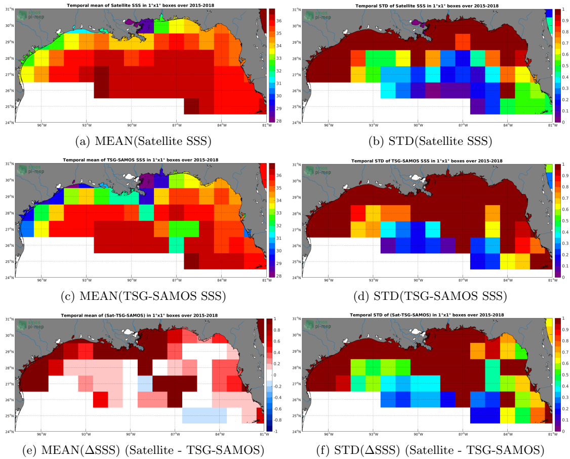
Figure 6: Temporal mean (left) and STD (right) of SSS from SMAP-L3-JPL-V4-MONTHLY-60KM (top), TSG-SAMOS (middle), and of \Delta SSS (Satellite - TSG-SAMOS). Only match-up pairs are used to generate these maps.
