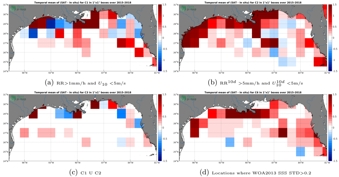
Figure 12: Temporal mean gridded over spatial boxes of size 1^\circ \times 1^\circ of \Delta SSS (SMAP-L3-JPL-V4-MONTHLY-60KM - TSG-SAMOS) for 4 different subdatasets corresponding to: RR > 1mm/h and U_{10} < 5\text{m/s} (a), RR^{10d} > 5\text{mm/h} and U_{10}^{10d} < 5\text{m/s} (b), C1 U C2 (c), Locations where WOA2013 SSS STD > 0.2 (d).
