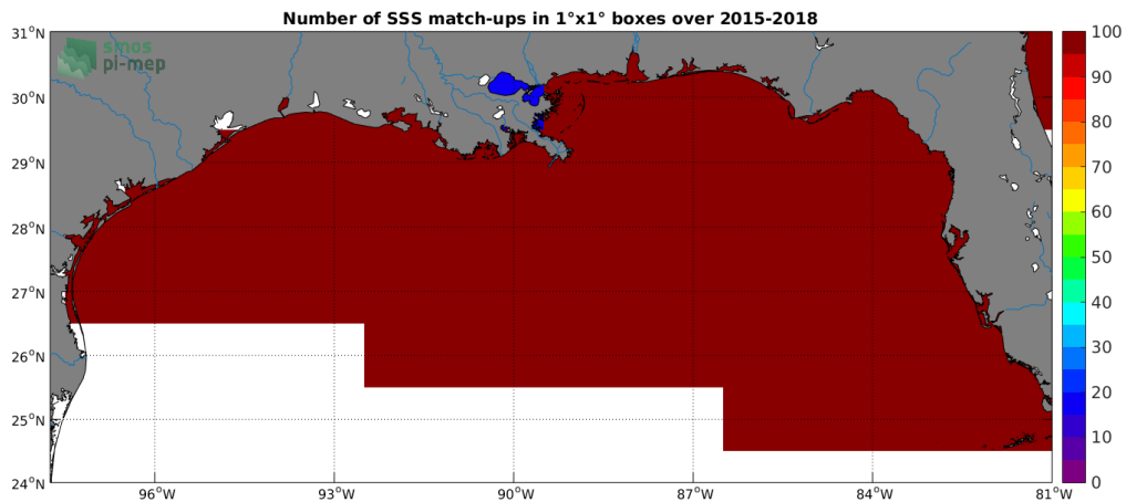
Figure 4: Number of SSS match-ups between TSG-SAMOS SSS and the SMAP-L3-JPL-V4-MONTHLY-60KM SSS product for the Mississippi river plume Pi-MEP region over 1^\circ \times 1^\circ boxes and for the full satellite product period.
