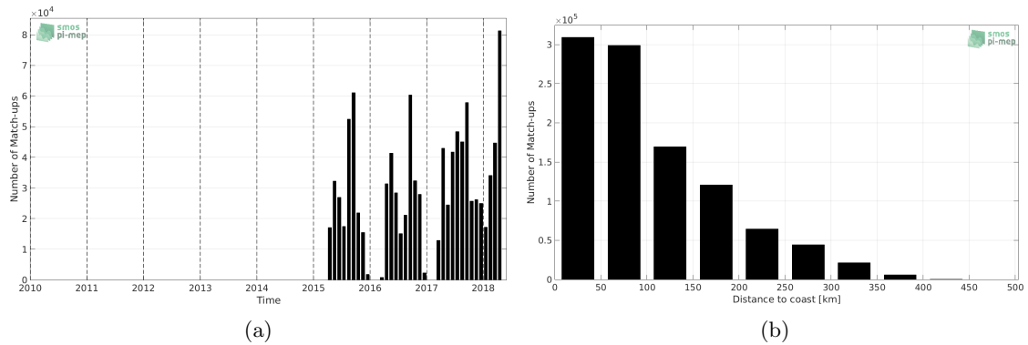
Figure 1: Number of match-ups between TSG-SAMOS and SMAP-L3-JPL-V4-MONTHLY-60KM SSS as a function of time (a) and as function of the distance to coast (b) over the Mississippi river plume Pi-MEP region and for the full satellite product period.
