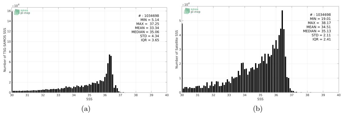
Figure 2: Histograms of SSS from TSG-SAMOS (a) and SMAP-L3-JPL-V4-MONTHLY-60KM (b) considering all match-up pairs per bins of 0.1 over the Mississippi river plume Pi-MEP region and for the full satellite product period.
