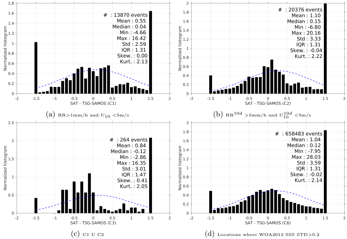
Figure 13: Normalized histogram of \Delta SSS (SMAP-L3-JPL-V4-MONTHLY-60KM - TSG-SAMOS) for 6 different subdatasets corresponding to: RR > 1\text{mm/h} and U_{10} < 5\text{m/s} (a), RR^{10d} > 5\text{mm/h} and U_{10}^{10d} < 5\text{m/s} (b), C1 U C2 (c), Locations where WOA2013 SSS STD > 0.2 (d).
