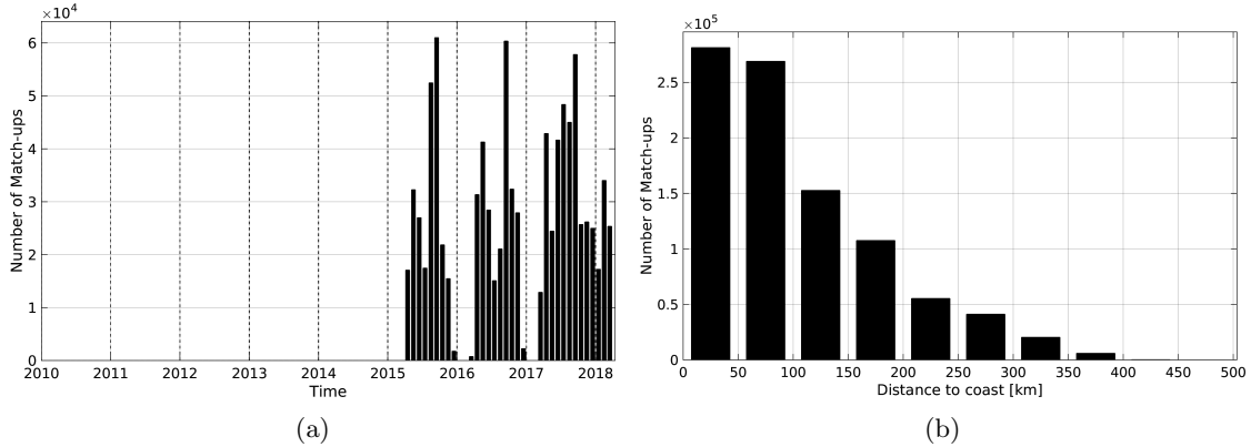
Figure 1: Number of match-ups between TSG-SAMOS and SMAP-L3-JPL-V4-MONTHLY-60KM SSS as a function of time (a) and as function of the distance to coast (b) over the Mississippi river plume Pi-MEP region and for the full satellite product period.
