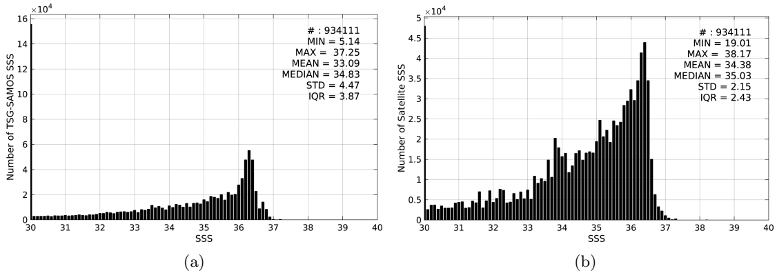
Figure 2: Histograms of SSS from TSG-SAMOS (a) and SMAP-L3-JPL-V4-MONTHLY-60KM (b) considering all match-up pairs per bins of 0.1 over the Mississippi river plume Pi-MEP region and for the full satellite product period.
