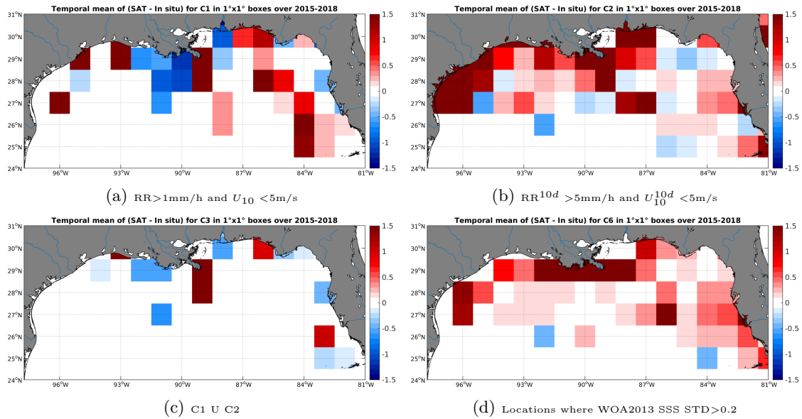
Figure 12: Temporal mean gridded over spatial boxes of size 1^\circ \times 1^\circ of \Delta SSS (SMAP-L3-JPL-V4-MONTHLY-60KM - TSG-SAMOS) for 4 different subdatasets corresponding to:RR >1 mm/h and U_{10} < 5 m/s (a), RR^{10d} > 5 mm/h and U_{10}^{10d} < 5 m/s (b), C1 U C2 (c),Locations where WOA2013 SSS STD >0.2 (d).
