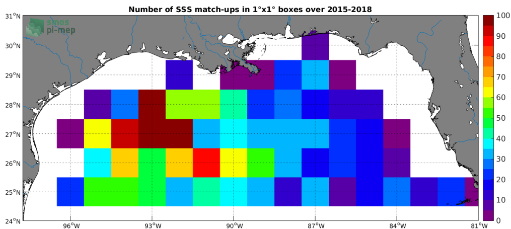
Figure 4: Number of SSS match-ups between Argo SSS and the SMAP-L3-JPL-V4-MONTHLY-60KM SSS product for the Mississippi river plume Pi-MEP region over 1^\circ \times 1^\circ boxes and for the full satellite product period.
