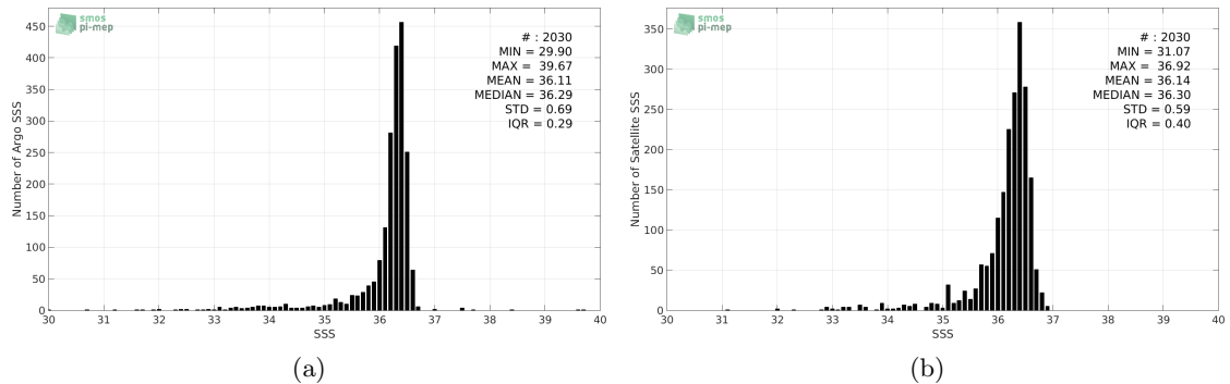
Figure 2: Histograms of SSS from Argo (a) and SMAP-L3-JPL-V4-MONTHLY-60KM (b) considering all match-up pairs per bins of 0.1 over the Mississippi river plume Pi-MEP region and for the full satellite product period.
