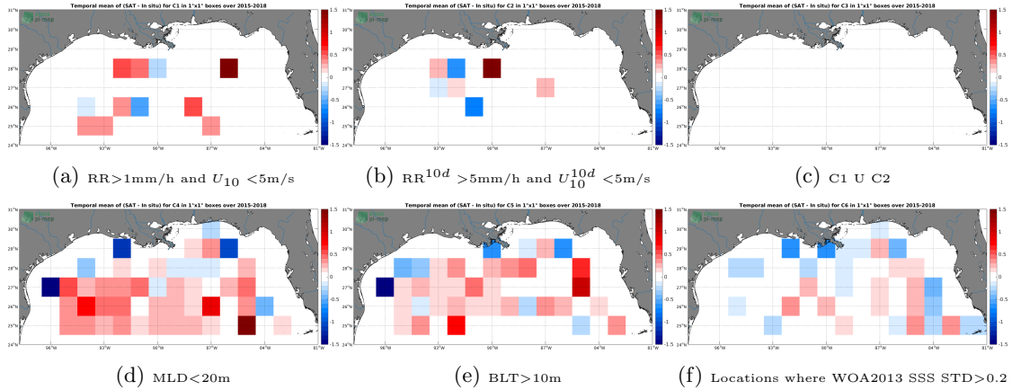
Figure 12: Temporal mean gridded over spatial boxes of size 1^\circ \times 1^\circ of \Delta SSS (SMAP-L3-JPL-V4-MONTHLY-60KM - Argo) for 6 different subdatasets corresponding to: RR>1mm/h and U_{10} < 5\text{m/s} (a), RR^{10d} > 5\text{mm/h} and U_{10}^{10d} < 5\text{m/s} (b), C1 U C2 (c),MLD<20m (d),BLT>10m (e),Locations where WOA2013 SSS STD>0.2 (f).
