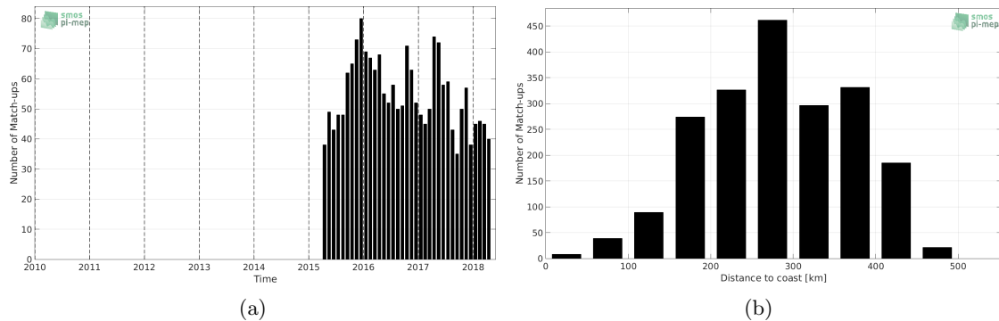
Figure 1: Number of match-ups between Argo and SMAP-L3-JPL-V4-MONTHLY-60KM SSS as a function of time (a) and as function of the distance to coast (b) over the Mississippi river plume Pi-MEP region and for the full satellite product period.
