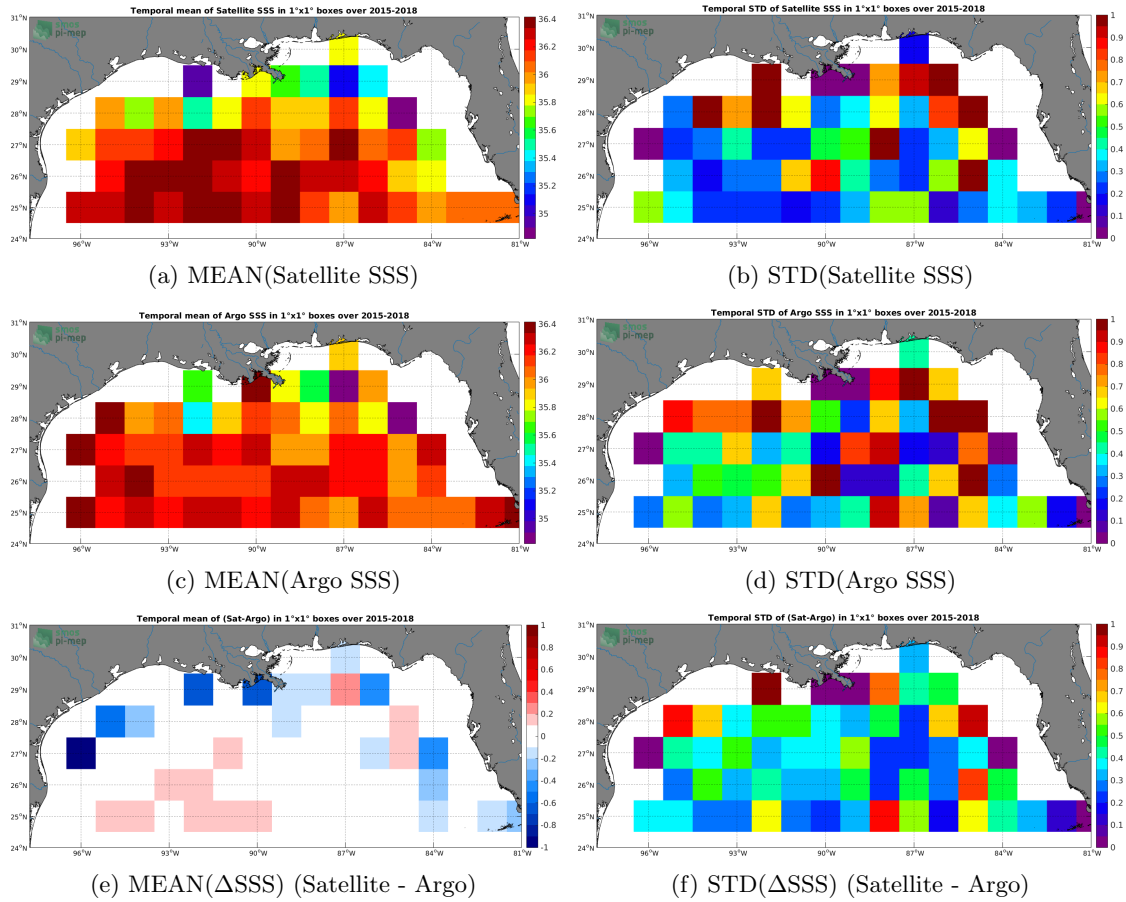
Figure 6: Temporal mean (left) and STD (right) of SSS from SMAP-L3-JPL-V4-MONTHLY-60KM (top), Argo (middle), and of \Delta SSS (Satellite - Argo). Only match-up pairs are used to generate these maps.
