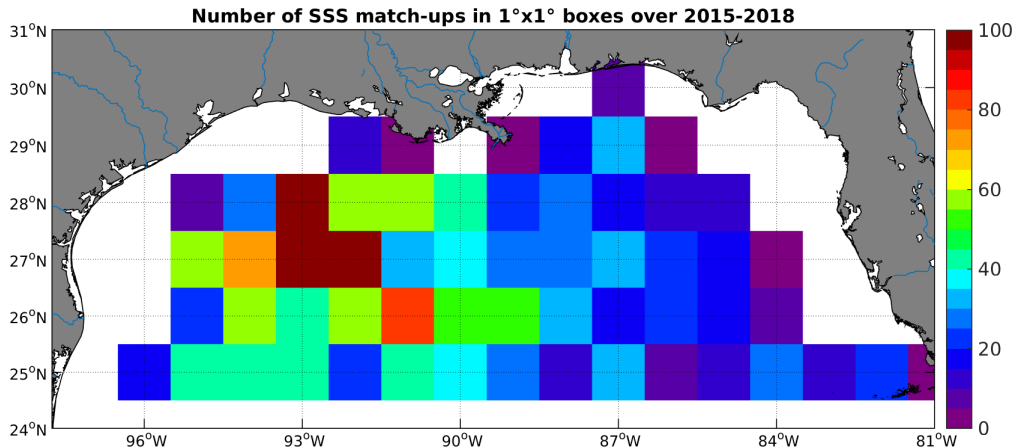
Figure 4: Number of SSS match-ups between Argo SSS and the SMAP-L3-JPL-V4-MONTHLY-60KM SSS product for the Mississippi river plume Pi-MEP region over 1°x1° boxes and for the full satellite product period.
