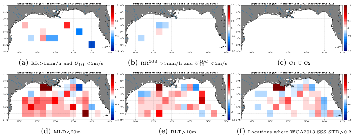
Figure 12: Temporal mean gridded over spatial boxes of size 1^\circ \times 1^\circ of \Delta SSS (SMAP-L3-JPL-V4-MONTHLY-60KM - Argo) for 6 different subdatasets corresponding to: RR > 1\text{mm/h} and U_{10} < 5\text{m/s} (a), RR^{10d} > 5\text{mm/h} and U_{10}^{10d} < 5\text{m/s} (b), C1 U C2 (c), MLD < 20\text{m} (d), BLT > 10\text{m} (e), Locations where WOA2013 SSS STD > 0.2 (f).
