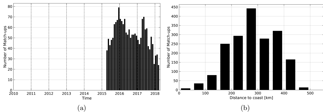
Figure 1: Number of match-ups between Argo and SMAP-L3-JPL-V4-MONTHLY-60KM SSS as a function of time (a) and as function of the distance to coast (b) over the Mississippi river plume Pi-MEP region and for the full satellite product period.
