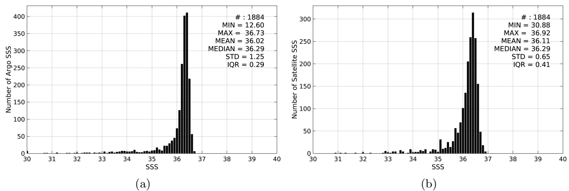
Figure 2: Histograms of SSS from Argo (a) and SMAP-L3-JPL-V4-MONTHLY-60KM (b) considering all match-up pairs per bins of 0.1 over the Mississippi river plume Pi-MEP region and for the full satellite product period.
