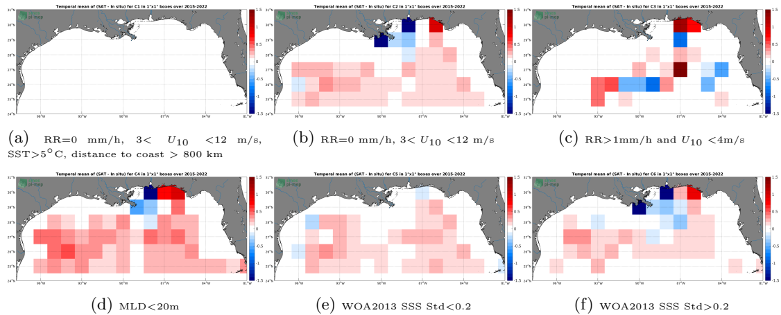
Figure 12: Temporal mean gridded over spatial boxes of size 1^{\circ}\times 1^{\circ} of \Delta\text{SSS} (SMAP SSS L2-AVERAGED v5 (RSS) - Argo) for 6 different subdatasets corresponding to:RR=0 mm/h, 3 < U_{10} < 12 m/s, SST > 5^{\circ}\text{C} , distance to coast > 800 km (a), RR=0 mm/h, 3 < U_{10} < 12 m/s (b), RR > 1\text{mm/h} and U_{10} < 4\text{m/s} (c),MLD < 20\text{m} (d),WOA2013 SSS Std < 0.2 (e),WOA2013 SSS Std > 0.2 (f).
