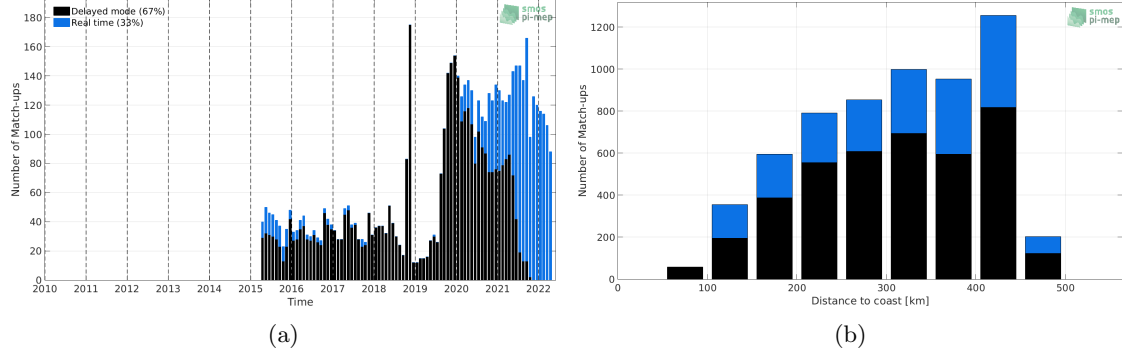
Figure 1: Number of match-ups between Argo and SMAP SSS L2-AVERAGED v5 (RSS) SSS as a function of time (a) and as function of the distance to coast (b) over the Mississippi river plume Pi-MEP region and for the full satellite product period.
