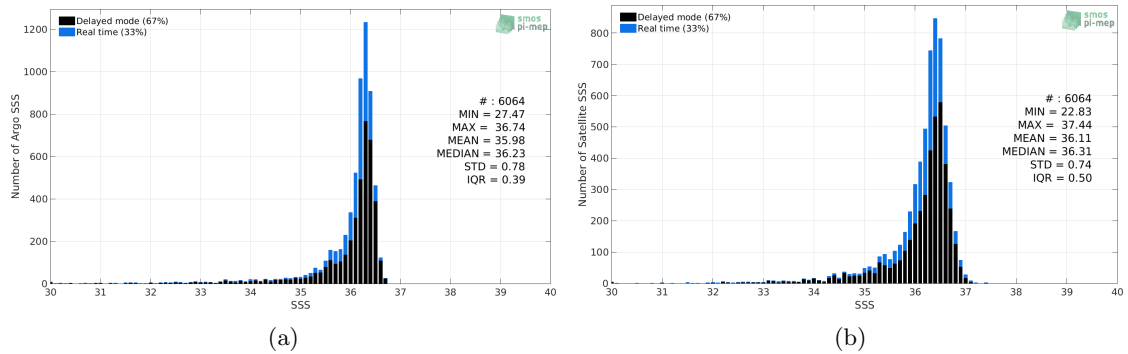
Figure 2: Histograms of SSS from Argo (a) and SMAP SSS L2-AVERAGED v5 (RSS) (b) considering all match-up pairs per bins of 0.1 over the Mississippi river plume Pi-MEP region and for the full satellite product period.
