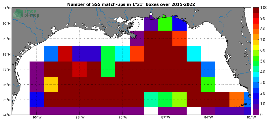
Figure 4: Number of SSS match-ups between Argo SSS and the SMAP SSS L2-AVERAGED v5 (RSS) SSS product for the Mississippi river plume Pi-MEP region over 1^{\circ} \times 1^{\circ} boxes and for the full satellite product period.
