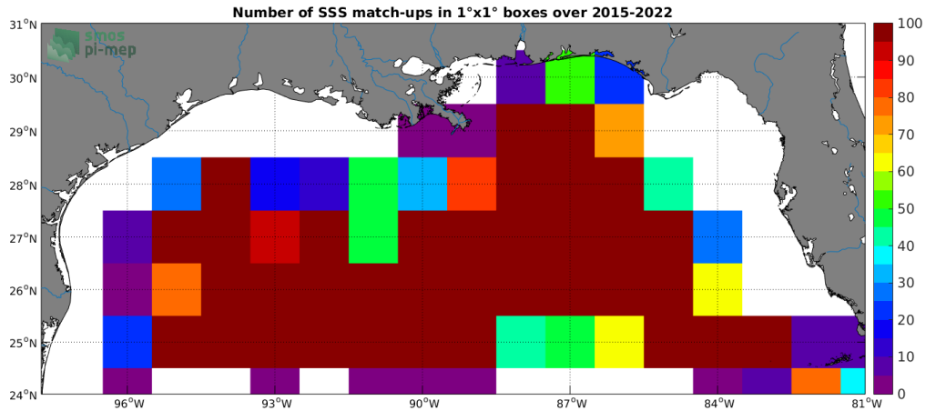
Figure 4: Number of SSS match-ups between Argo SSS and the SMAP SSS L2-AVERAGED v5.0 (JPL) SSS product for the Mississippi river plume Pi-MEP region over 1^\circ \times 1^\circ boxes and for the full satellite product period.
