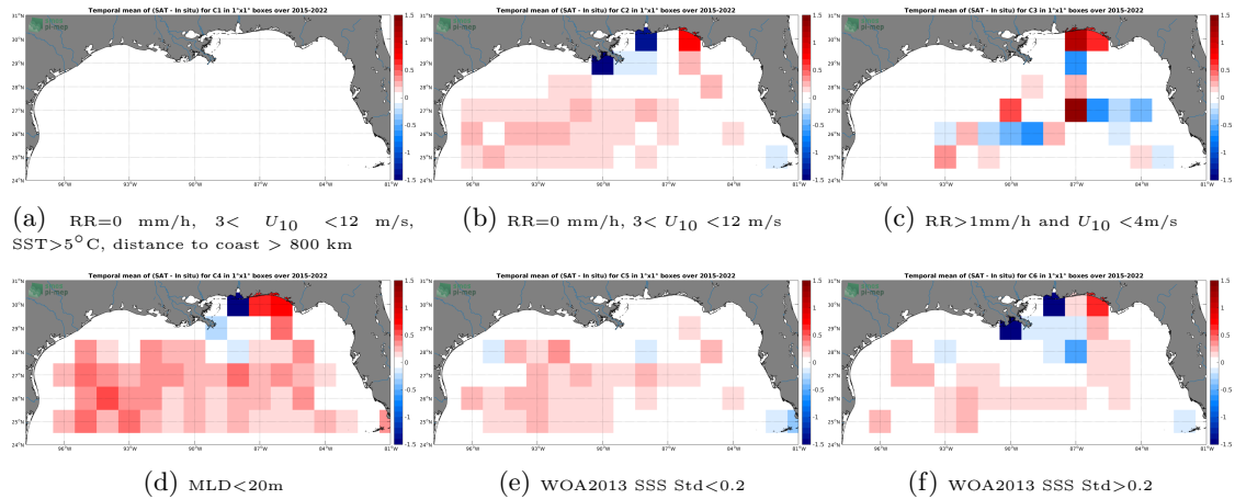
Figure 12: Temporal mean gridded over spatial boxes of size 1^{\circ}\times 1^{\circ} of \Delta\text{SSS} (SMAP SSS L2-AVERAGED v5.0 (JPL) - Argo) for 6 different subdatasets corresponding to:RR=0 mm/h, 3 < U_{10} < 12 m/s, SST > 5^{\circ}\text{C} , distance to coast > 800 km (a), RR=0 mm/h, 3 < U_{10} < 12 m/s (b), RR > 1\text{mm/h} and U_{10} < 4\text{m/s} (c),MLD < 20\text{m} (d),WOA2013 SSS Std < 0.2 (e),WOA2013 SSS Std > 0.2 (f).
