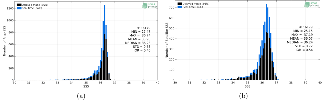
Figure 2: Histograms of SSS from Argo (a) and SMAP SSS L2-AVERAGED v5.0 (JPL) (b) considering all match-up pairs per bins of 0.1 over the Mississippi river plume Pi-MEP region and for the full satellite product period.
