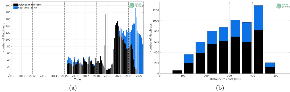
Figure 1: Number of match-ups between Argo and SMAP SSS L2-AVERAGED v5.0 (JPL) SSS as a function of time (a) and as function of the distance to coast (b) over the Mississippi river plume Pi-MEP region and for the full satellite product period.
