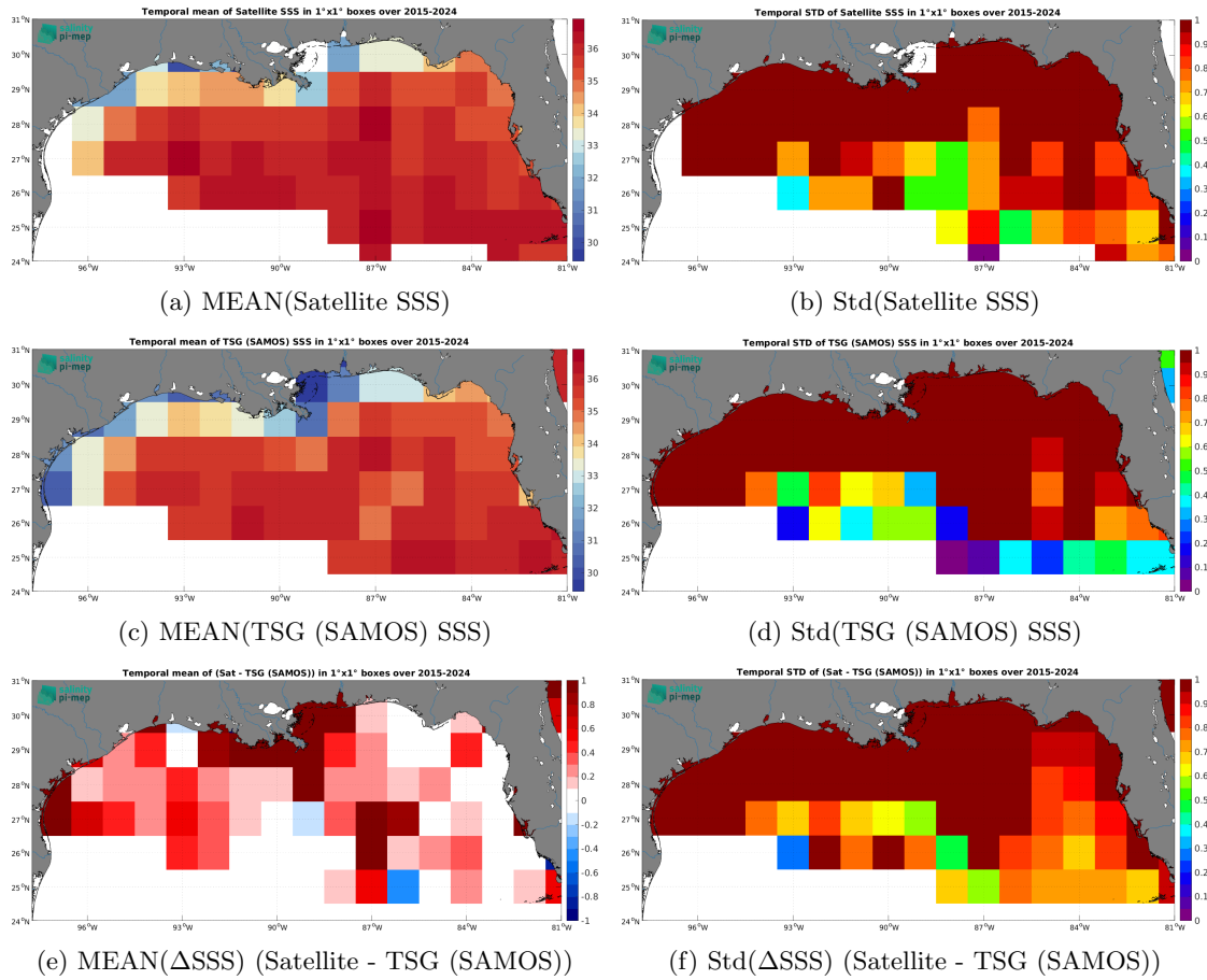
Figure 7: Temporal mean (left) and Std (right) of SSS from SMAP SSS L2 v6 - 40 km (RSS) (top), TSG (SAMOS) (middle), and of \Delta SSS (Satellite - TSG (SAMOS)). Only match-up pairs are used to generate these maps.
