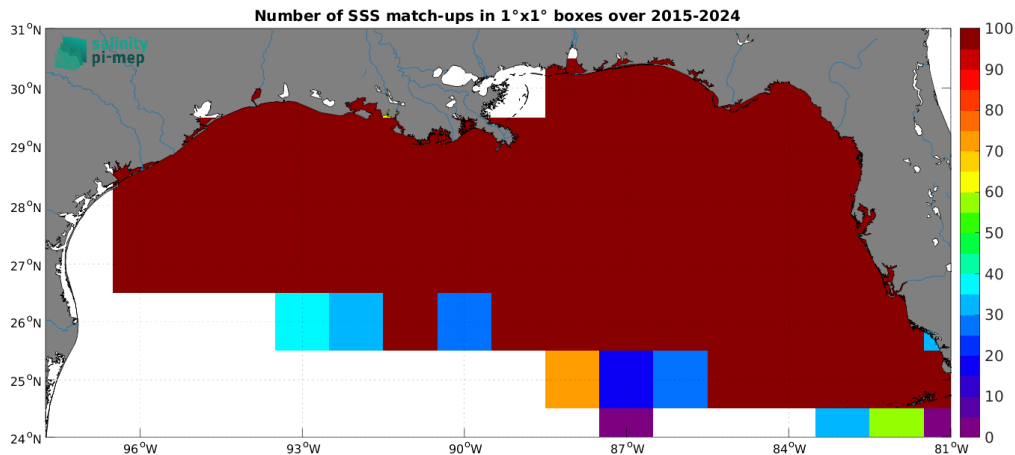
Figure 5: Number of SSS match-ups between TSG (SAMOS) SSS and the SMAP SSS L2 v6 - 40 km (RSS) SSS product for the Mississippi river plume Pi-MEP region over 1^\circ \times 1^\circ boxes and for the full satellite product period.
