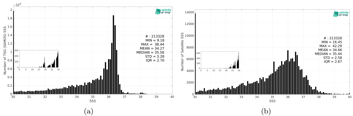
Figure 3: Histograms of SSS from TSG (SAMOS) (a) and SMAP SSS L2 v6 - 40 km (RSS) (b) considering all match-up pairs per bins of 0.1 over the Mississippi river plume Pi-MEP region and for the full satellite product period.
