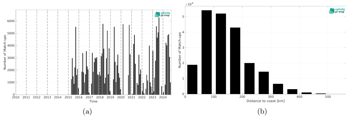
Figure 2: Number of match-ups between TSG (SAMOS) and SMAP SSS L2 v6 - 40 km (RSS) SSS as a function of time (a) and as function of the distance to coast (b) over the Mississippi river plume Pi-MEP region and for the full satellite product period.
