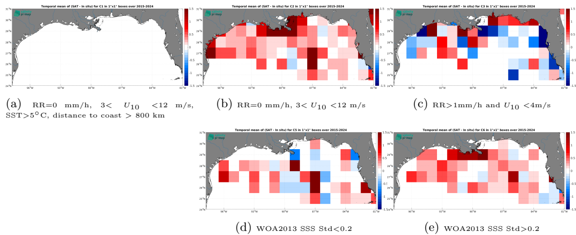
Figure 14: Temporal mean gridded over spatial boxes of size 1^\circ \times 1^\circ of \Delta SSS (SMAP SSS L2 v6 - 40 km (RSS) - TSG (SAMOS)) for 5 different subdatasets corresponding to:RR=0 mm/h, 3 < U_{10} < 12 m/s, SST > 5°C, distance to coast > 800 km (a), RR=0 mm/h, 3 < U_{10} < 12 m/s (b), RR > 1mm/h and U_{10} < 4 m/s (c), WOA2013 SSS Std < 0.2 (d), WOA2013 SSS Std > 0.2 (e).
