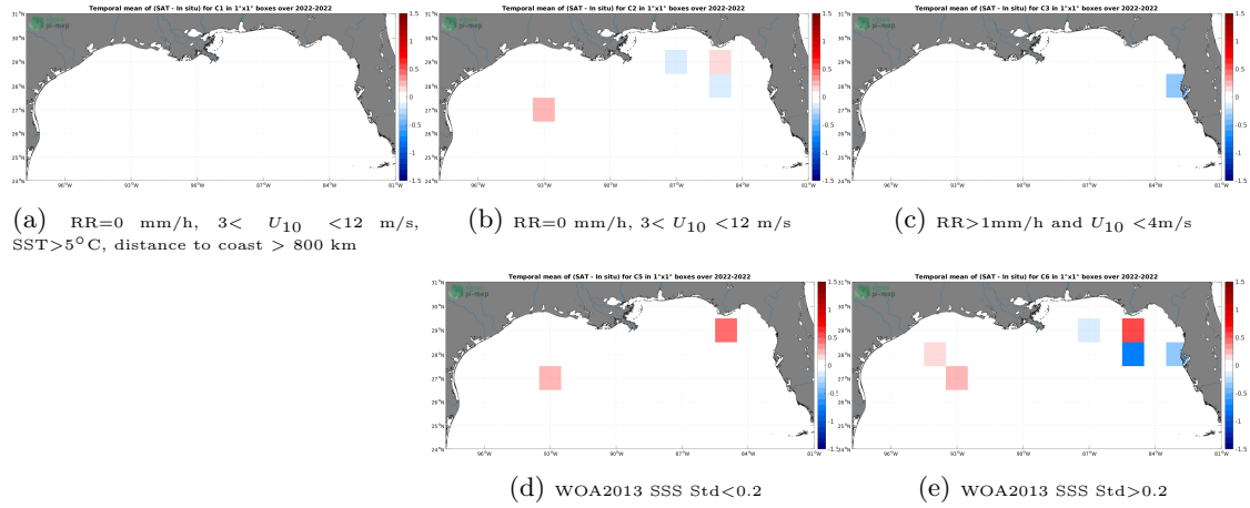
Figure 12: Temporal mean gridded over spatial boxes of size 1^{\circ}\times 1^{\circ} of \Delta\text{SSS} (SMAP SSS L2 v5 (RSS) - Saildrone) for 5 different subdatasets corresponding to:RR=0 mm/h, 3 < U_{10} < 12 m/s, SST >5^{\circ}\text{C} , distance to coast > 800 km (a), RR=0 mm/h, 3 < U_{10} < 12 m/s (b), RR >1 mm/h and U_{10} < 4 m/s (c), WOA2013 SSS Std <0.2 (d), WOA2013 SSS Std >0.2 (e).
