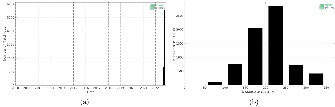
Figure 1: Number of match-ups between Sairdron and SMAP SSS L2 v5 (RSS) SSS as a function of time (a) and as function of the distance to coast (b) over the Mississippi river plume Pi-MEP region and for the full satellite product period.
