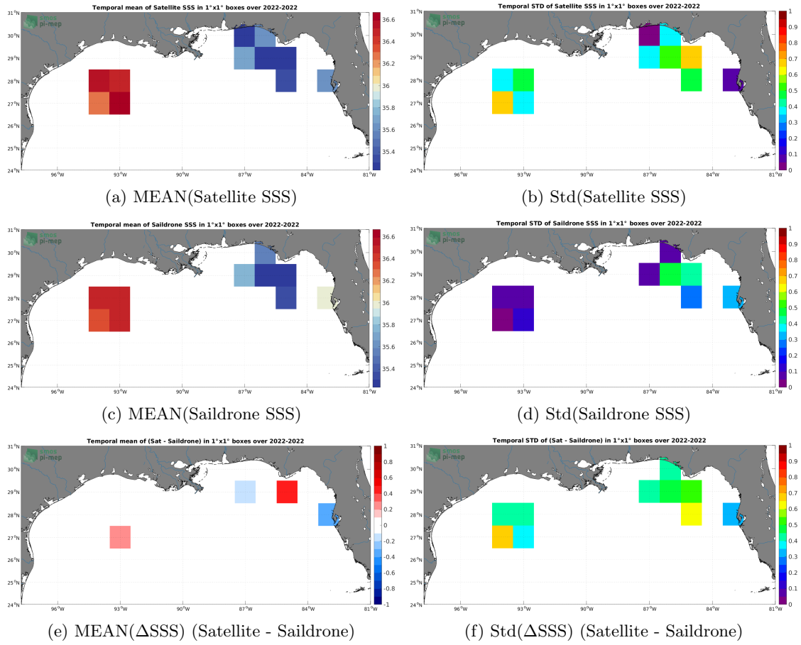
Figure 6: Temporal mean (left) and Std (right) of SSS from SMAP SSS L2 v5 (RSS) (top), Saildrone (middle), and of \Delta SSS (Satellite - Saildrone). Only match-up pairs are used to generate these maps.
