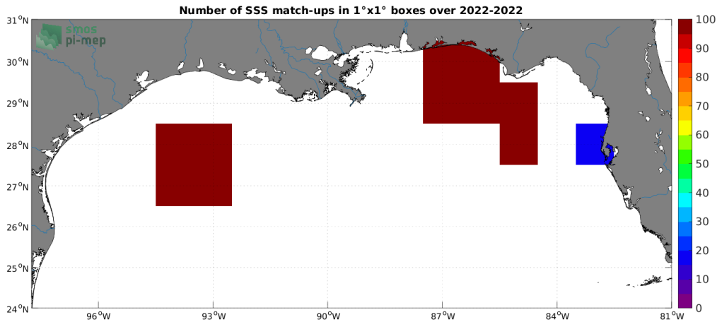
Figure 4: Number of SSS match-ups between Saildrone SSS and the SMAP SSS L2 v5 (RSS) SSS product for the Mississippi river plume Pi-MEP region over 1^\circ \times 1^\circ boxes and for the full satellite product period.
