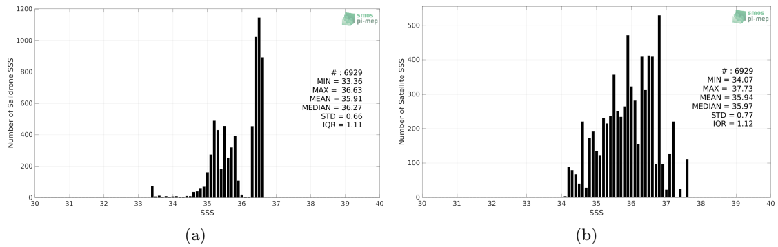
Figure 2: Histograms of SSS from Sairdron (a) and SMAP SSS L2 v5 (RSS) (b) considering all match-up pairs per bins of 0.1 over the Mississippi river plume Pi-MEP region and for the full satellite product period.
