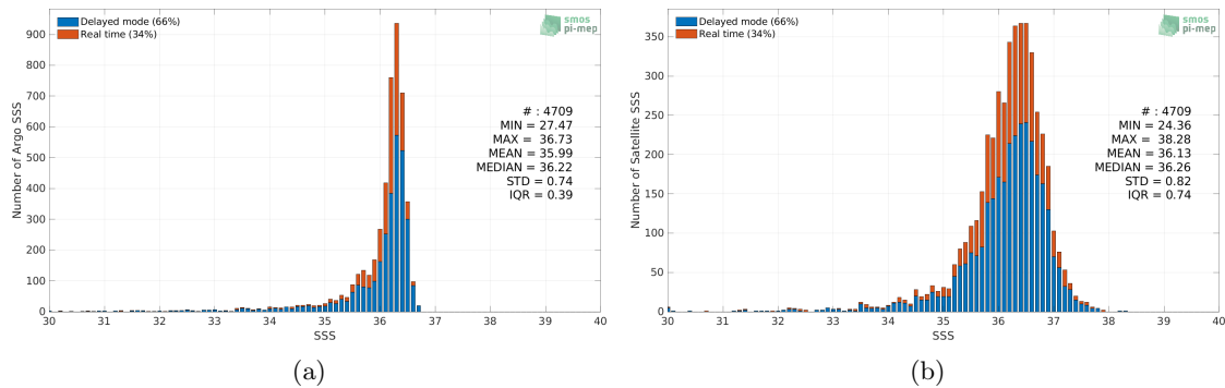
Figure 2: Histograms of SSS from Argo (a) and SMAP SSS L2 v5 (RSS) (b) considering all match-up pairs per bins of 0.1 over the Mississippi river plume Pi-MEP region and for the full satellite product period.
