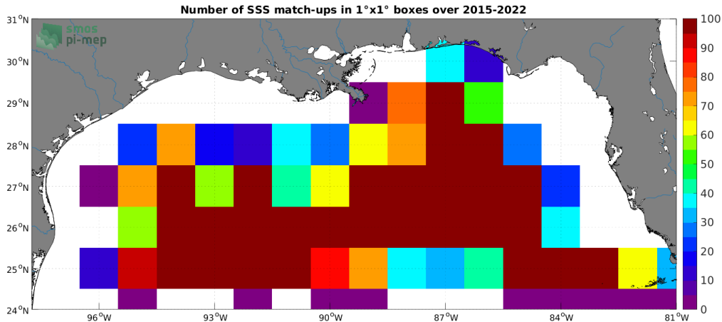
Figure 4: Number of SSS match-ups between Argo SSS and the SMAP SSS L2 v5 (RSS) SSS product for the Mississippi river plume Pi-MEP region over 1^\circ \times 1^\circ boxes and for the full satellite product period.
