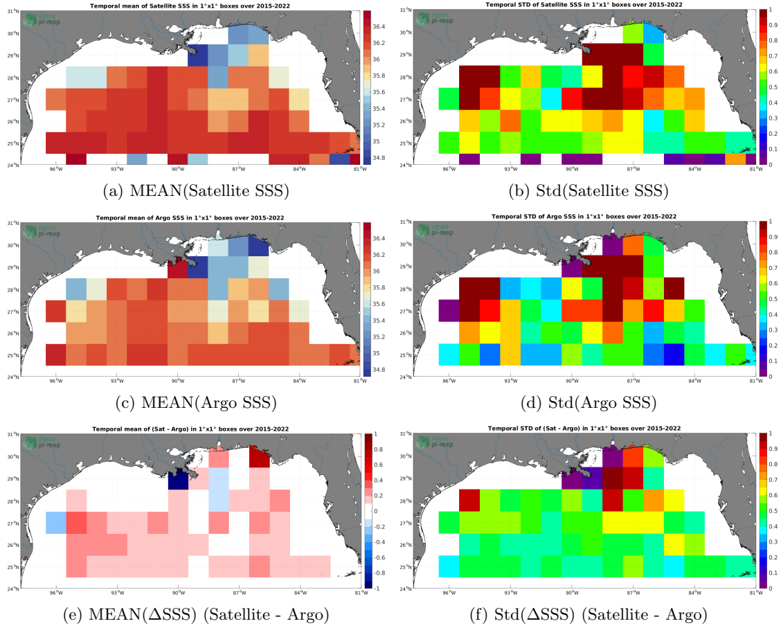
Figure 6: Temporal mean (left) and Std (right) of SSS from SMAP SSS L2 v5 (RSS) (top), Argo (middle), and of \Delta SSS (Satellite - Argo). Only match-up pairs are used to generate these maps.
