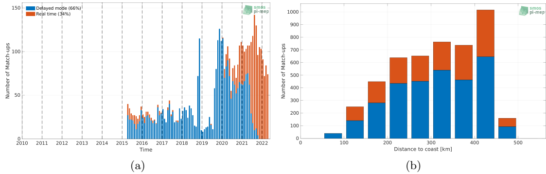
Figure 1: Number of match-ups between Argo and SMAP SSS L2 v5 (RSS) SSS as a function of time (a) and as function of the distance to coast (b) over the Mississippi river plume Pi-MEP region and for the full satellite product period.
