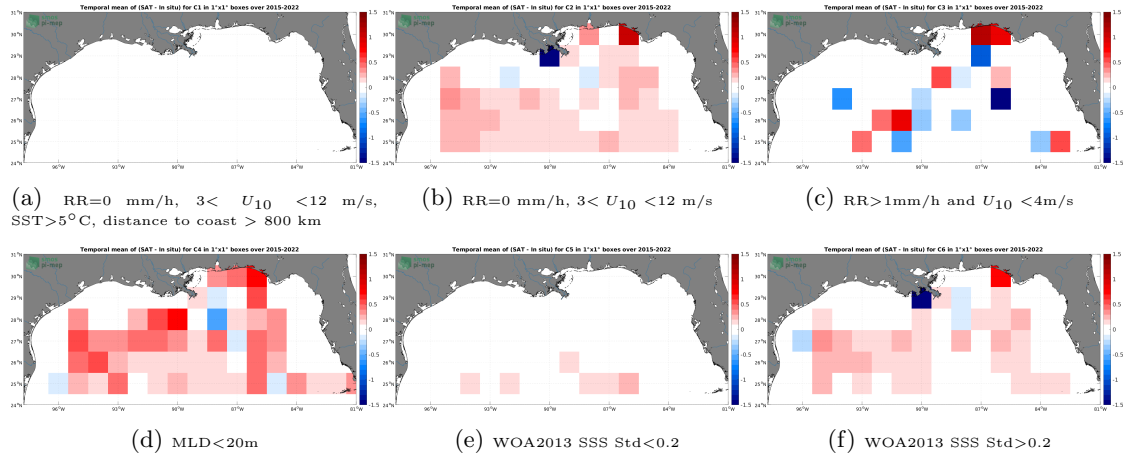
Figure 12: Temporal mean gridded over spatial boxes of size 1^{\circ}\times 1^{\circ} of \Delta\text{SSS} (SMAP SSS L2 v5 (RSS) - Argo) for 6 different subdatasets corresponding to:RR=0 mm/h, 3 < U_{10} < 12 m/s, SST > 5^{\circ}\text{C} , distance to coast > 800 km (a), RR=0 mm/h, 3 < U_{10} < 12 m/s (b), RR > 1\text{mm/h} and U_{10} < 4\text{m/s} (c),MLD < 20\text{m} (d),WOA2013 SSS Std < 0.2 (e),WOA2013 SSS Std > 0.2 (f).
