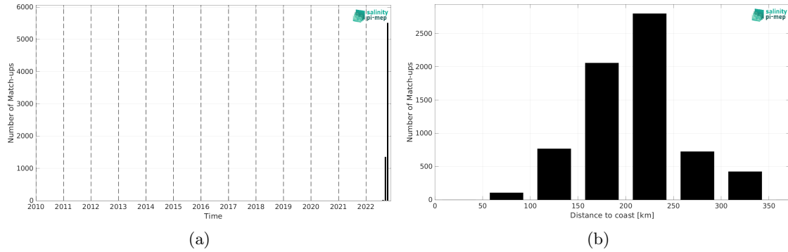
Figure 2: Number of match-ups between Sairdron and SMAP SSS L2 v5.3 (RSS) SSS as a function of time (a) and as function of the distance to coast (b) over the Mississippi river plume Pi-MEP region and for the full satellite product period.
