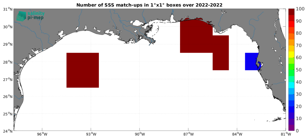
Figure 5: Number of SSS match-ups between Saildrone SSS and the SMAP SSS L2 v5.3 (RSS) SSS product for the Mississippi river plume Pi-MEP region over 1^\circ \times 1^\circ boxes and for the full satellite product period.
