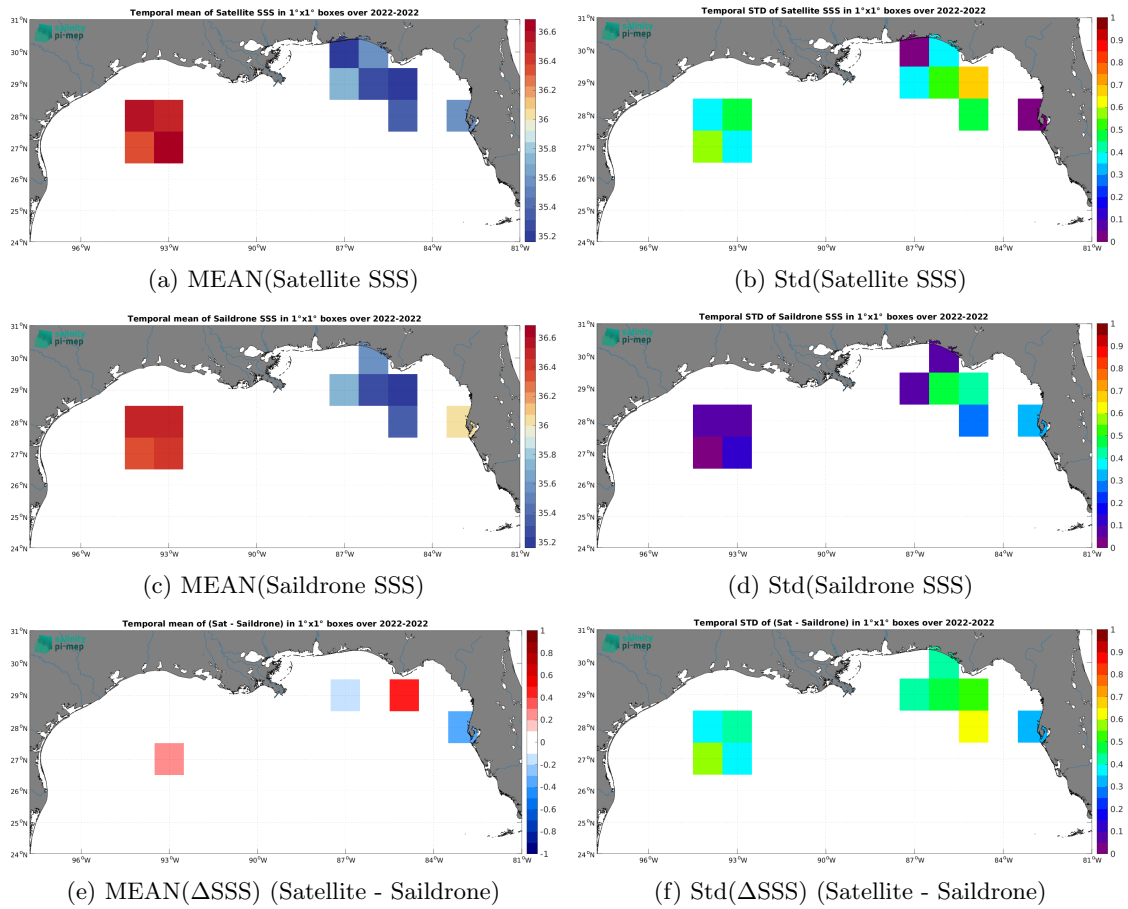
Figure 7: Temporal mean (left) and Std (right) of SSS from SMAP SSS L2 v5.3 (RSS) (top), Saildrone (middle), and of \Delta SSS (Satellite - Saildrone). Only match-up pairs are used to generate these maps.
