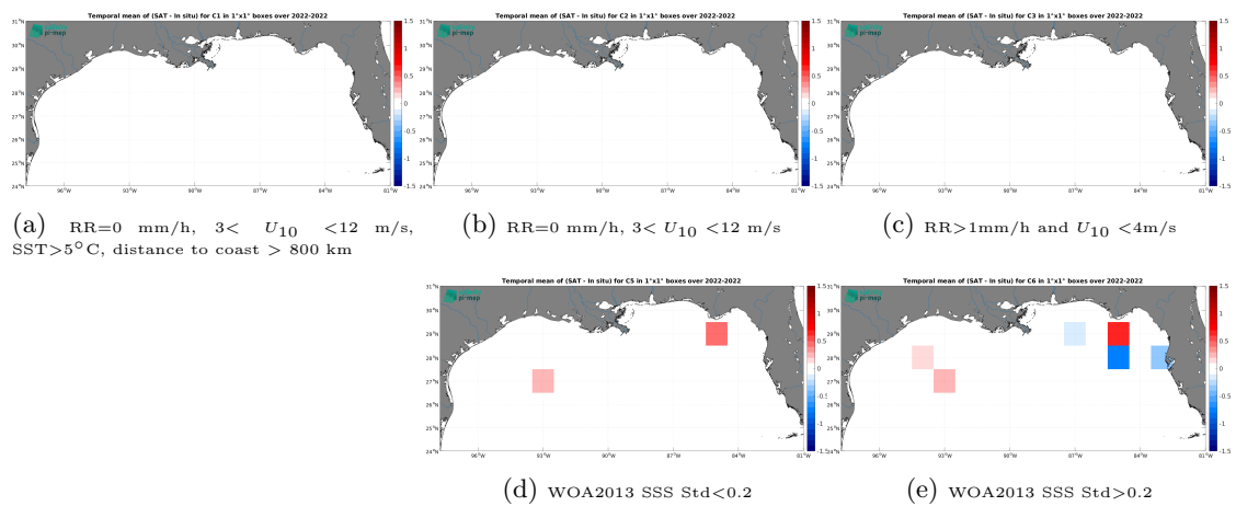
Figure 14: Temporal mean gridded over spatial boxes of size 1^\circ \times 1^\circ of \Delta SSS (SMAP SSS L2 v5.3 (RSS) - Saldrone) for 5 different subdatasets corresponding to:RR=0 mm/h, 3 < U_{10} < 12 m/s, SST > 5°C, distance to coast > 800 km (a), RR=0 mm/h, 3 < U_{10} < 12 m/s (b), RR > 1mm/h and U_{10} < 4 m/s (c), WOA2013 SSS Std < 0.2 (d), WOA2013 SSS Std > 0.2 (e).
