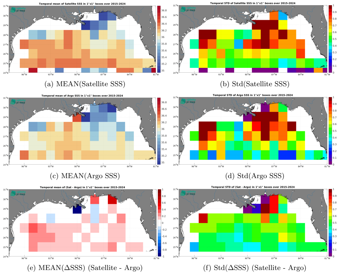
Figure 7: Temporal mean (left) and Std (right) of SSS from SMAP SSS L2 v5.3 (RSS) (top), Argo (middle), and of \Delta SSS (Satellite - Argo). Only match-up pairs are used to generate these maps.
