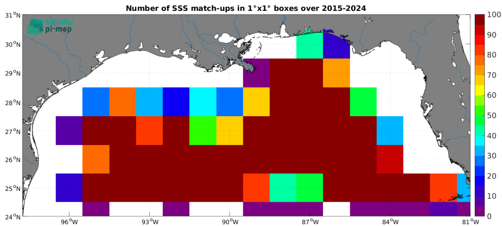
Figure 5: Number of SSS match-ups between Argo SSS and the SMAP SSS L2 v5.3 (RSS) SSS product for the Mississippi river plume Pi-MEP region over 1^{\circ} \times 1^{\circ} boxes and for the full satellite product period.
