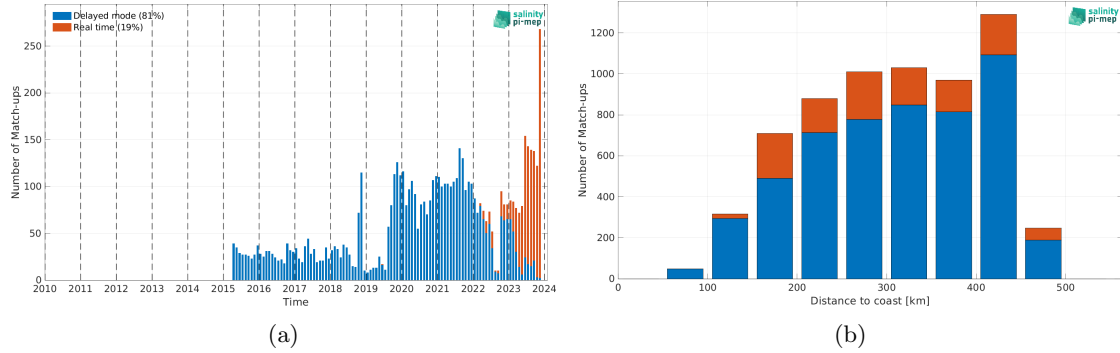
Figure 2: Number of match-ups between Argo and SMAP SSS L2 v5.3 (RSS) SSS as a function of time (a) and as function of the distance to coast (b) over the Mississippi river plume Pi-MEP region and for the full satellite product period.
