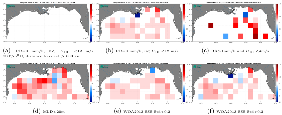
Figure 14: Temporal mean gridded over spatial boxes of size 1^\circ \times 1^\circ of \Delta SSS (SMAP SSS L2 v5.3 (RSS) - Argo) for 6 different subdatasets corresponding to:RR=0 mm/h, 3 < U_{10} < 12 m/s, SST>5°C, distance to coast > 800 km (a), RR=0 mm/h, 3 < U_{10} < 12 m/s (b), RR>1mm/h and U_{10} < 4 m/s (c),MLD<20m (d),WOA2013 SSS Std<0.2 (e),WOA2013 SSS Std>0.2 (f).
