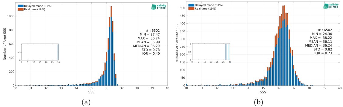
Figure 3: Histograms of SSS from Argo (a) and SMAP SSS L2 v5.3 (RSS) (b) considering all match-up pairs per bins of 0.1 over the Mississippi river plume Pi-MEP region and for the full satellite product period.
