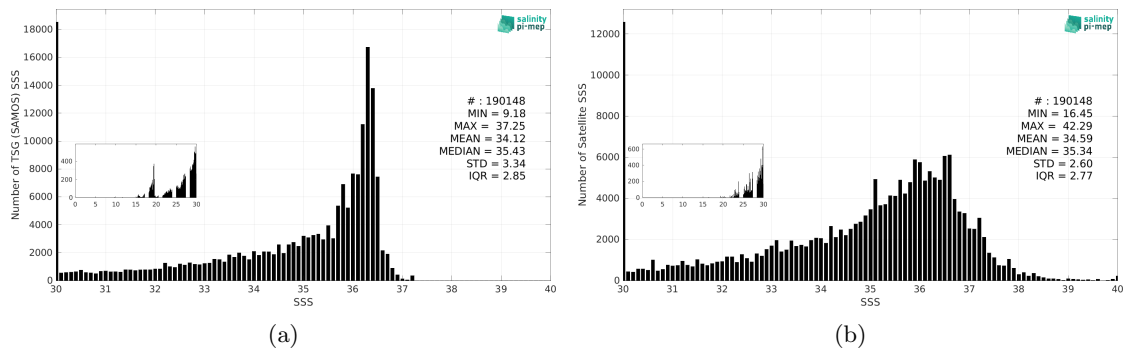
Figure 3: Histograms of SSS from TSG (SAMOS) (a) and SMAP SSS L2 v5.3 - 40 km (RSS) (b) considering all match-up pairs per bins of 0.1 over the Mississippi river plume Pi-MEP region and for the full satellite product period.
