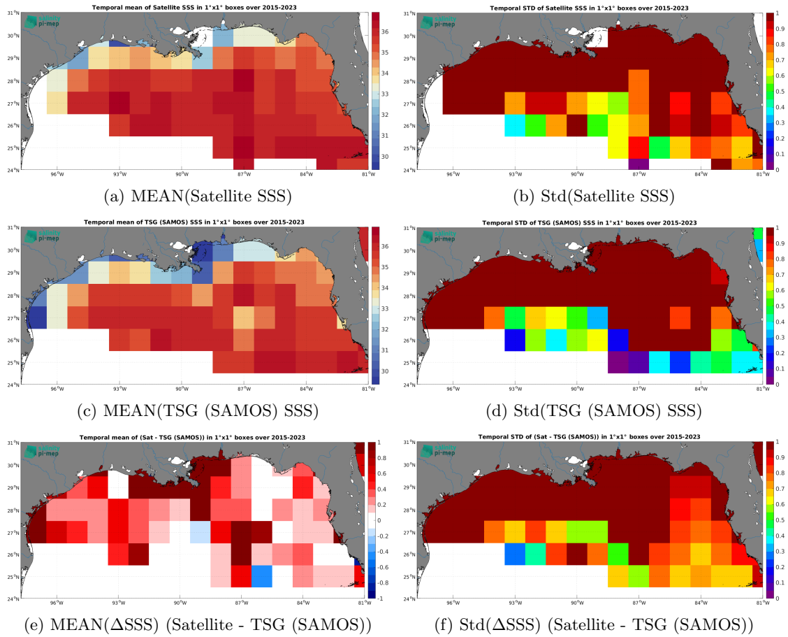
Figure 7: Temporal mean (left) and Std (right) of SSS from SMAP SSS L2 v5.3 - 40 km (RSS) (top), TSG (SAMOS) (middle), and of \Delta SSS (Satellite - TSG (SAMOS)). Only match-up pairs are used to generate these maps.
