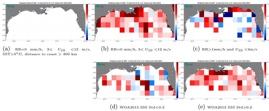
Figure 14: Temporal mean gridded over spatial boxes of size 1^\circ \times 1^\circ of \Delta SSS (SMAP SSS L2 v5.3 - 40 km (RSS) - TSG (SAMOS)) for 5 different subdatasets corresponding to: RR=0 mm/h, 3 < U_{10} < 12 m/s, SST > 5°C, distance to coast > 800 km (a), RR=0 mm/h, 3 < U_{10} < 12 m/s (b), RR > 1mm/h and U_{10} < 4 m/s (c), WOA2013 SSS Std < 0.2 (d), WOA2013 SSS Std > 0.2 (e).
