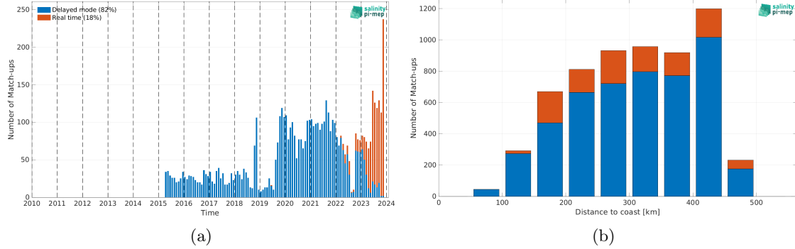
Figure 2: Number of match-ups between Argo and SMAP SSS L2 v5.3 - 40 km (RSS) SSS as a function of time (a) and as function of the distance to coast (b) over the Mississippi river plume Pi-MEP region and for the full satellite product period.
