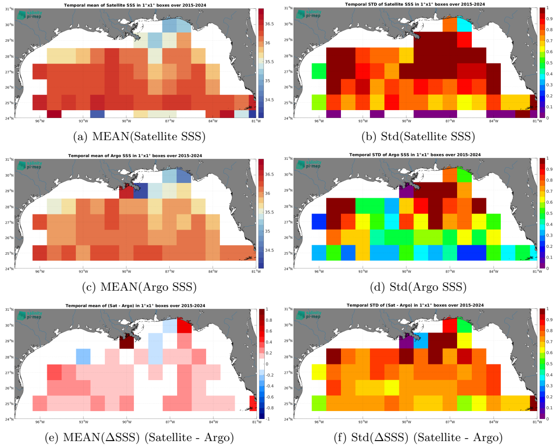
Figure 7: Temporal mean (left) and Std (right) of SSS from SMAP SSS L2 v5.3 - 40 km (RSS) (top), Argo (middle), and of \Delta SSS (Satellite - Argo). Only match-up pairs are used to generate these maps.
