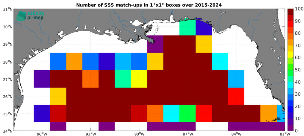
Figure 5: Number of SSS match-ups between Argo SSS and the SMAP SSS L2 v5.3 - 40 km (RSS) SSS product for the Mississippi river plume Pi-MEP region over 1^{\circ} \times 1^{\circ} boxes and for the full satellite product period.
