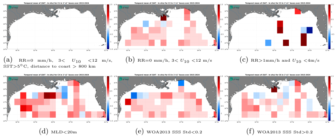
Figure 14: Temporal mean gridded over spatial boxes of size 1^\circ \times 1^\circ of \Delta SSS (SMAP SSS L2 v5.3 - 40 km (RSS) - Argo) for 6 different subdatasets corresponding to: RR=0 mm/h, 3 < U_{10} < 12 m/s, SST > 5^\circ\text{C} , distance to coast > 800 km (a), RR=0 mm/h, 3 < U_{10} < 12 m/s (b), RR > 1 mm/h and U_{10} < 4 m/s (c), MLD < 20 m (d), WOA2013 SSS Std < 0.2 (e), WOA2013 SSS Std > 0.2 (f).
