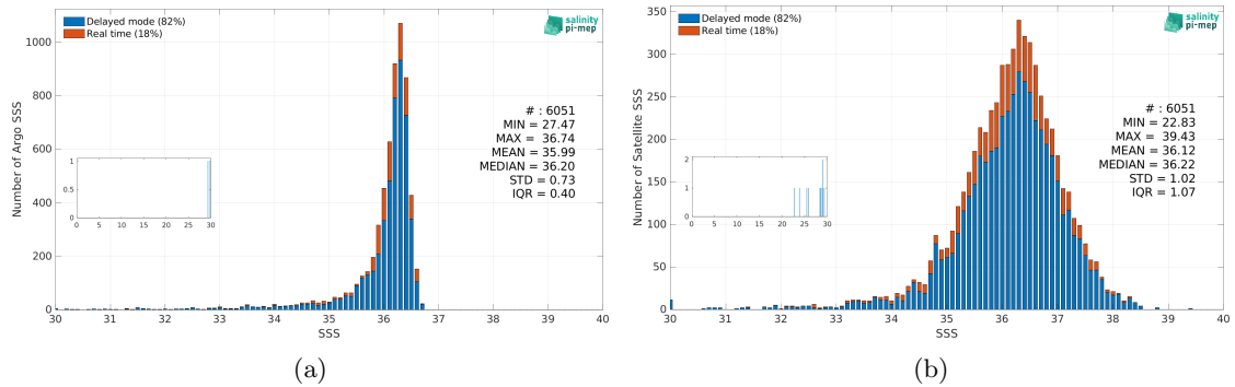
Figure 3: Histograms of SSS from Argo (a) and SMAP SSS L2 v5.3 - 40 km (RSS) (b) considering all match-up pairs per bins of 0.1 over the Mississippi river plume Pi-MEP region and for the full satellite product period.
