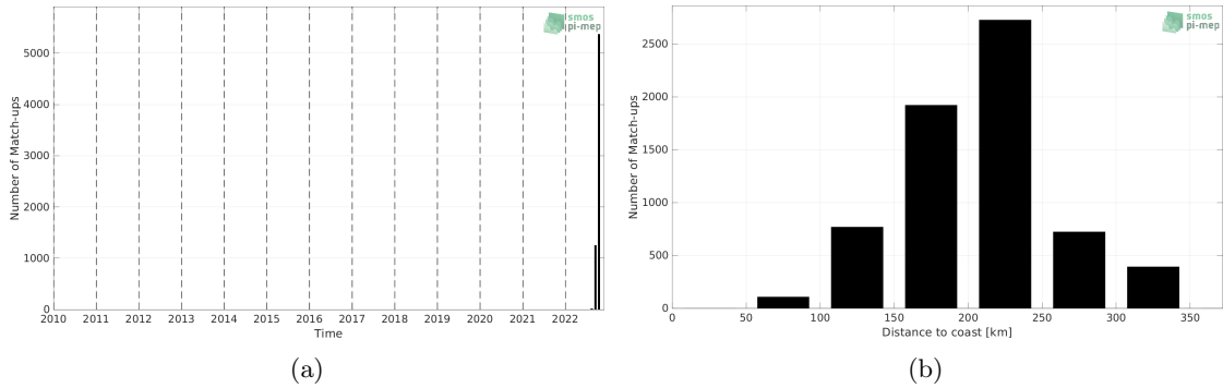
Figure 1: Number of match-ups between Saildrone and SMAP SSS L2 v5 - 40 km (RSS) SSS as a function of time (a) and as function of the distance to coast (b) over the Mississippi river plume Pi-MEP region and for the full satellite product period.
