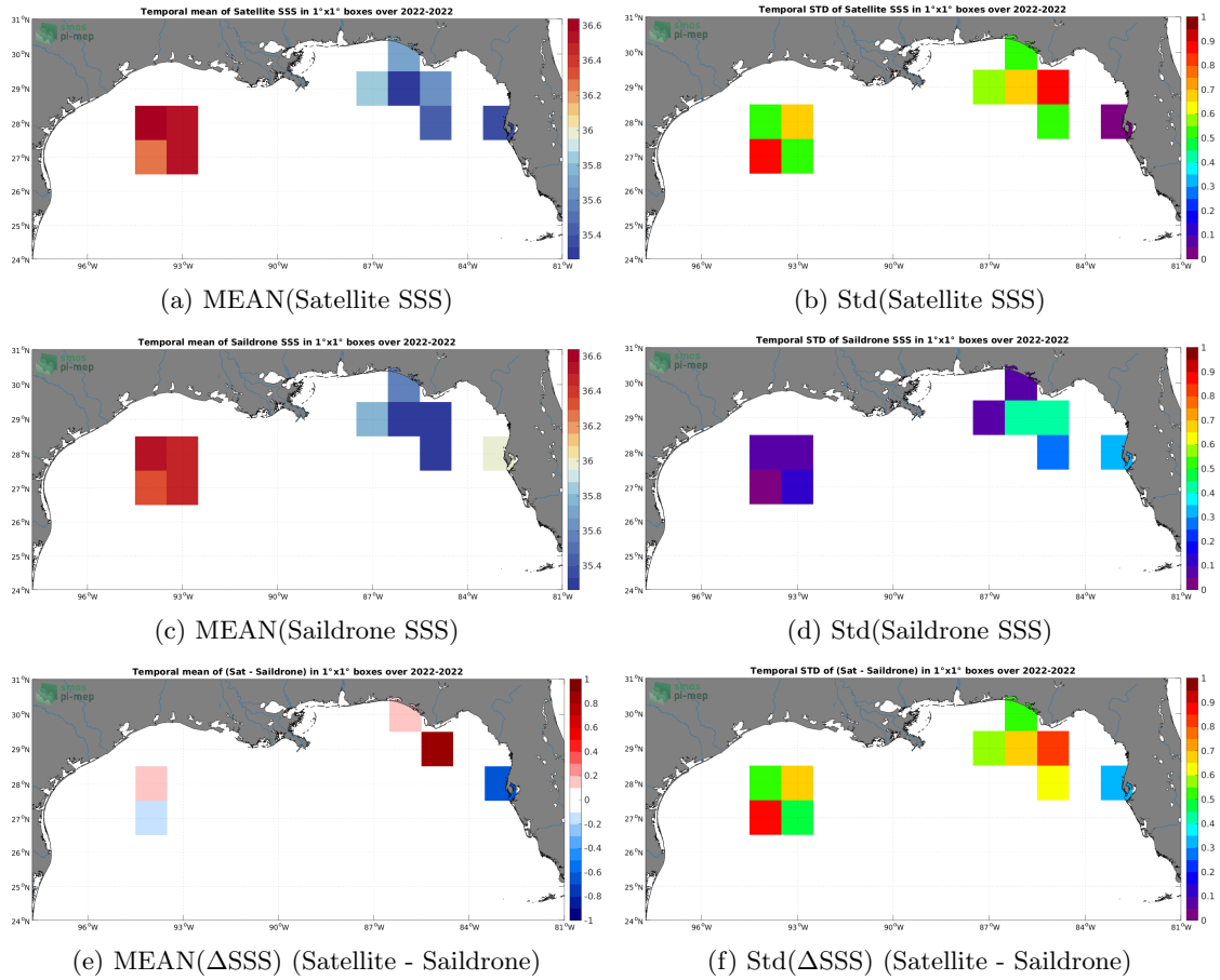
Figure 6: Temporal mean (left) and Std (right) of SSS from SMAP SSS L2 v5 - 40 km (RSS) (top), Saildrone (middle), and of \Delta SSS (Satellite - Saildrone). Only match-up pairs are used to generate these maps.
