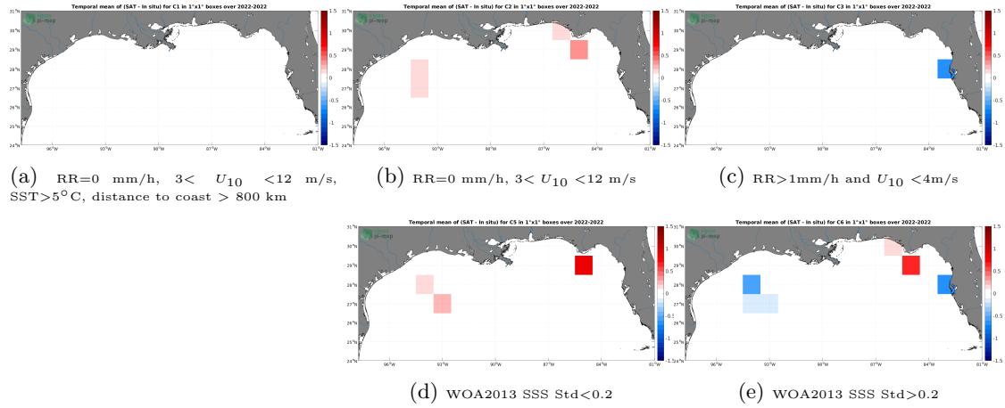
Figure 12: Temporal mean gridded over spatial boxes of size 1^{\circ}\times 1^{\circ} of \Delta\text{SSS} (SMAP SSS L2 v5 - 40 km (RSS) - Saldrone) for 5 different subdatasets corresponding to:RR=0 mm/h, 3 < U_{10} < 12 m/s, SST >5^{\circ}\text{C} , distance to coast > 800 km (a), RR=0 mm/h, 3 < U_{10} < 12 m/s (b), RR >1 mm/h and U_{10} < 4 m/s (c), WOA2013 SSS Std <0.2 (d), WOA2013 SSS Std >0.2 (e).
