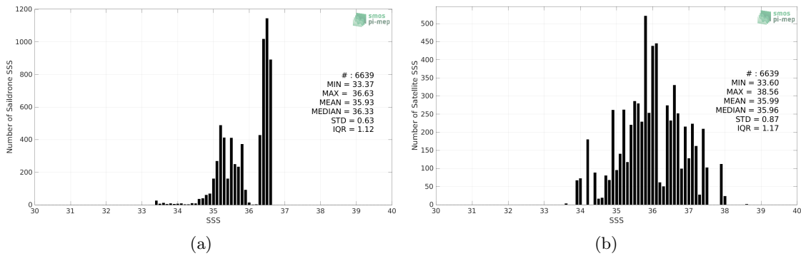
Figure 2: Histograms of SSS from Saildrone (a) and SMAP SSS L2 v5 - 40 km (RSS) (b) considering all match-up pairs per bins of 0.1 over the Mississippi river plume Pi-MEP region and for the full satellite product period.
