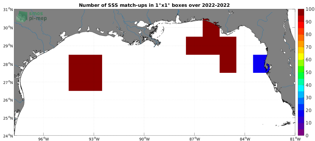
Figure 4: Number of SSS match-ups between Saildrone SSS and the SMAP SSS L2 v5 - 40 km (RSS) SSS product for the Mississippi river plume Pi-MEP region over 1^\circ \times 1^\circ boxes and for the full satellite product period.
