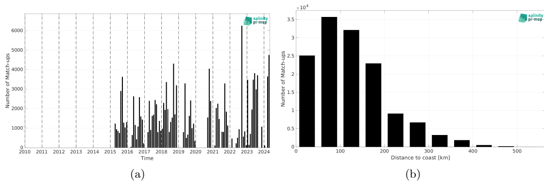
Figure 2: Number of match-ups between TSG (SAMOS) and SMAP SSS L2 v5.0 (JPL) SSS as a function of time (a) and as function of the distance to coast (b) over the Mississippi river plume Pi-MEP region and for the full satellite product period.
