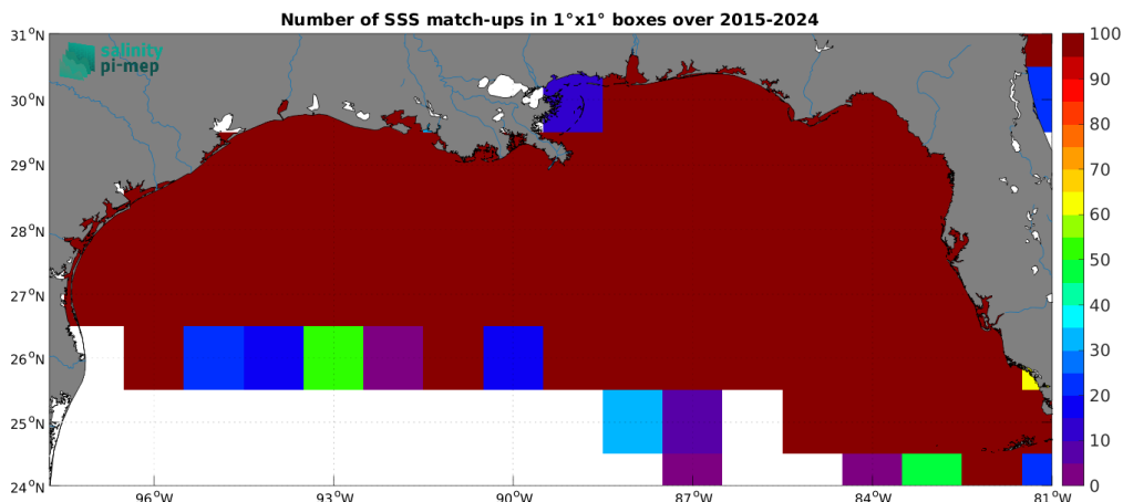
Figure 5: Number of SSS match-ups between TSG (SAMOS) SSS and the SMAP SSS L2 v5.0 (JPL) SSS product for the Mississippi river plume Pi-MEP region over 1^\circ \times 1^\circ boxes and for the full satellite product period.
