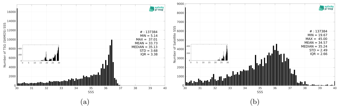
Figure 3: Histograms of SSS from TSG (SAMOS) (a) and SMAP SSS L2 v5.0 (JPL) (b) considering all match-up pairs per bins of 0.1 over the Mississippi river plume Pi-MEP region and for the full satellite product period.
