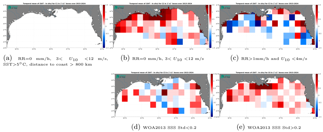
Figure 14: Temporal mean gridded over spatial boxes of size 1^\circ \times 1^\circ of \Delta SSS (SMAP SSS L2 v5.0 (JPL) - TSG (SAMOS)) for 5 different subdatasets corresponding to:RR=0 mm/h, 3 < U_{10} < 12 m/s, SST > 5°C, distance to coast > 800 km (a), RR=0 mm/h, 3 < U_{10} < 12 m/s (b), RR > 1mm/h and U_{10} < 4 m/s (c), WOA2013 SSS Std < 0.2 (d), WOA2013 SSS Std > 0.2 (e).
