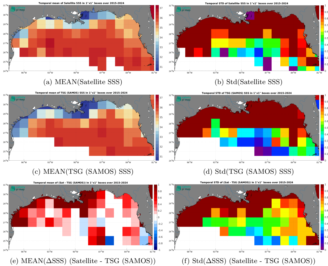
Figure 7: Temporal mean (left) and Std (right) of SSS from SMAP SSS L2 v5.0 (JPL) (top), TSG (SAMOS) (middle), and of \Delta SSS (Satellite - TSG (SAMOS)). Only match-up pairs are used to generate these maps.
