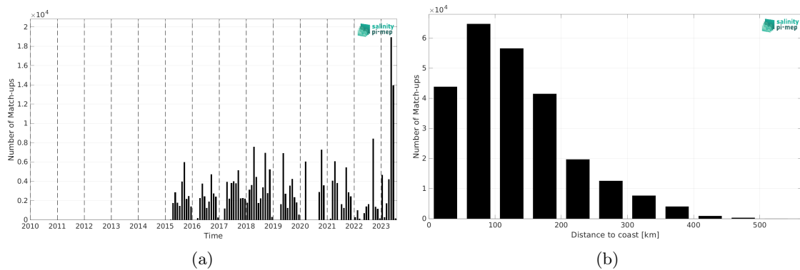
Figure 1: Number of match-ups between TSG (SAMOS) and SMAP SSS L2 v5.0 (JPL) SSS as a function of time (a) and as function of the distance to coast (b) over the Mississippi river plume Pi-MEP region and for the full satellite product period.
