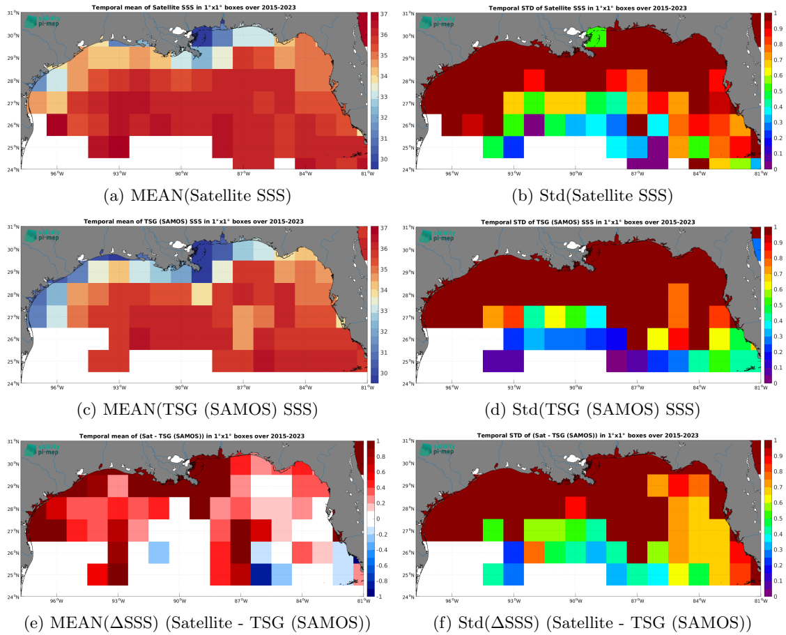
Figure 6: Temporal mean (left) and Std (right) of SSS from SMAP SSS L2 v5.0 (JPL) (top), TSG (SAMOS) (middle), and of \Delta SSS (Satellite - TSG (SAMOS)). Only match-up pairs are used to generate these maps.
