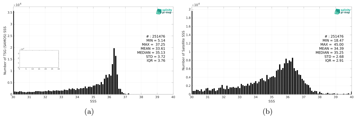
Figure 2: Histograms of SSS from TSG (SAMOS) (a) and SMAP SSS L2 v5.0 (JPL) (b) considering all match-up pairs per bins of 0.1 over the Mississippi river plume Pi-MEP region and for the full satellite product period.
