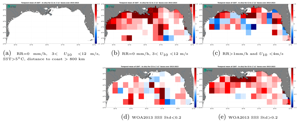
Figure 12: Temporal mean gridded over spatial boxes of size 1^{\circ}\times 1^{\circ} of \Delta\text{SSS} (SMAP SSS L2 v5.0 (JPL) - TSG (SAMOS)) for 5 different subdatasets corresponding to:RR=0 mm/h, 3 < U_{10} < 12 m/s, SST >5^{\circ}\text{C} , distance to coast > 800 km (a), RR=0 mm/h, 3 < U_{10} < 12 m/s (b), RR >1 mm/h and U_{10} < 4 m/s (c), WOA2013 SSS Std <0.2 (d), WOA2013 SSS Std >0.2 (e).
