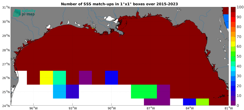
Figure 4: Number of SSS match-ups between TSG (SAMOS) SSS and the SMAP SSS L2 v5.0 (JPL) SSS product for the Mississippi river plume Pi-MEP region over 1^\circ \times 1^\circ boxes and for the full satellite product period.
