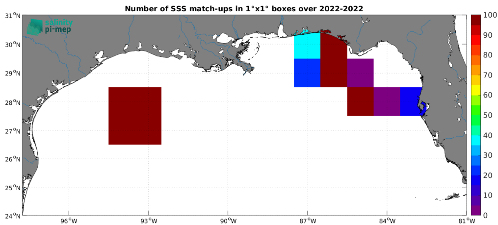
Figure 5: Number of SSS match-ups between Sailability SSS and the SMAP SSS L2 v5.0 (JPL) SSS product for the Mississippi river plume Pi-MEP region over 1^\circ \times 1^\circ boxes and for the full satellite product period.
