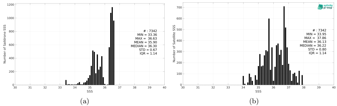
Figure 2: Histograms of SSS from Saildrone (a) and SMAP SSS L2 v5.0 (JPL) (b) considering all match-up pairs per bins of 0.1 over the Mississippi river plume Pi-MEP region and for the full satellite product period.
