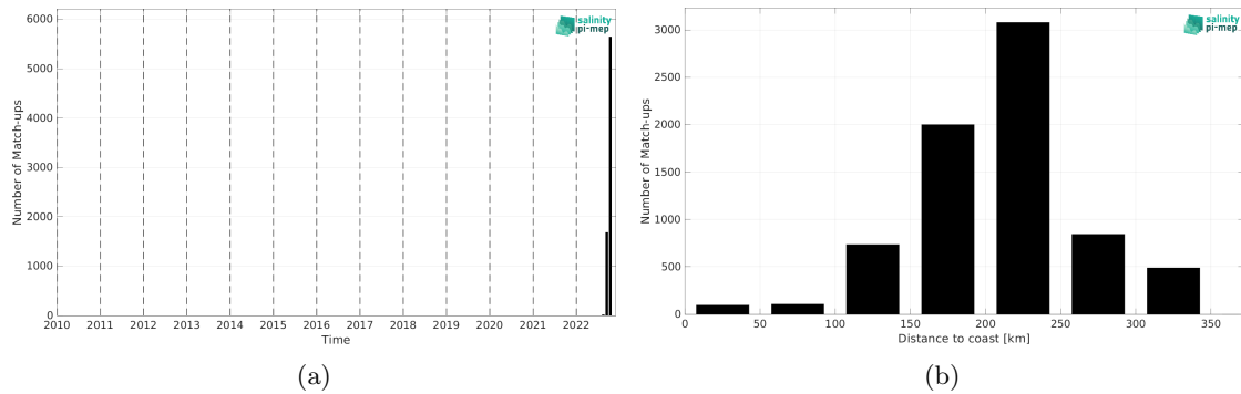
Figure 1: Number of match-ups between Saildrone and SMAP SSS L2 v5.0 (JPL) SSS as a function of time (a) and as function of the distance to coast (b) over the Mississippi river plume Pi-MEP region and for the full satellite product period.
