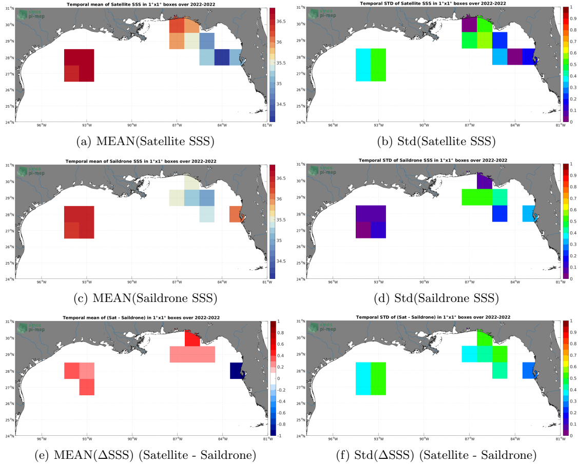
Figure 6: Temporal mean (left) and Std (right) of SSS from SMAP SSS L2 v5.0 (JPL) (top), Saildrone (middle), and of \Delta SSS (Satellite - Saildrone). Only match-up pairs are used to generate these maps.
