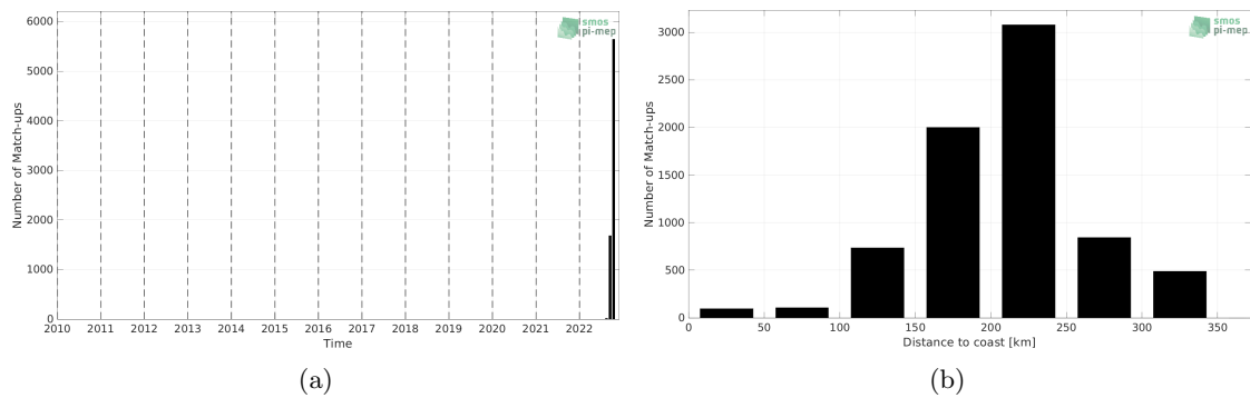
Figure 1: Number of match-ups between Sairdronne and SMAP SSS L2 v5.0 (JPL) SSS as a function of time (a) and as function of the distance to coast (b) over the Mississippi river plume Pi-MEP region and for the full satellite product period.
