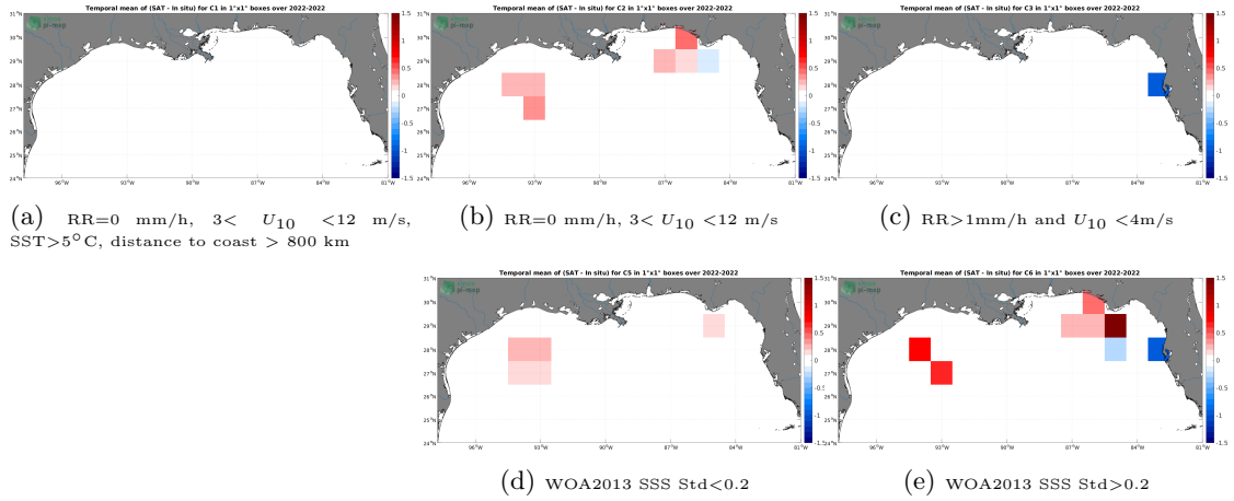
Figure 12: Temporal mean gridded over spatial boxes of size 1^{\circ}\times 1^{\circ} of \Delta\text{SSS} (SMAP SSS L2 v5.0 (JPL) - Saildrone) for 5 different subdatasets corresponding to:RR=0 mm/h, 3 < U_{10} < 12 m/s, SST >5^{\circ}\text{C} , distance to coast > 800 km (a), RR=0 mm/h, 3 < U_{10} < 12 m/s (b), RR >1 mm/h and U_{10} < 4 m/s (c), WOA2013 SSS Std <0.2 (d), WOA2013 SSS Std >0.2 (e).
