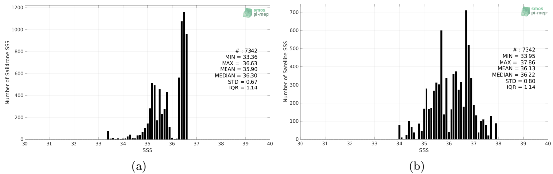
Figure 2: Histograms of SSS from Sairdronne (a) and SMAP SSS L2 v5.0 (JPL) (b) considering all match-up pairs per bins of 0.1 over the Mississippi river plume Pi-MEP region and for the full satellite product period.
