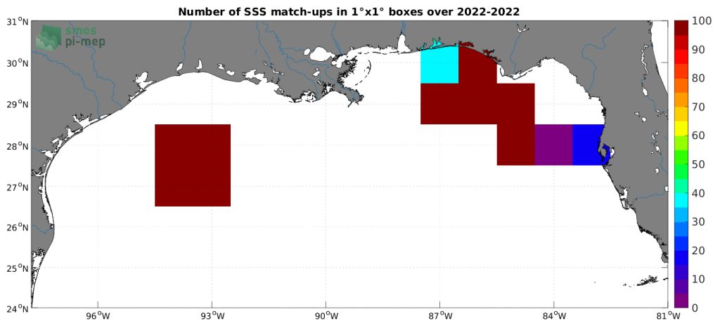
Figure 4: Number of SSS match-ups between Saildrone SSS and the SMAP SSS L2 v5.0 (JPL) SSS product for the Mississippi river plume Pi-MEP region over 1^\circ \times 1^\circ boxes and for the full satellite product period.
