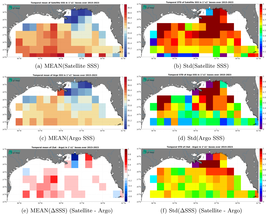
Figure 6: Temporal mean (left) and Std (right) of SSS from SMAP SSS L2 v5.0 (JPL) (top), Argo (middle), and of \Delta\text{SSS} (Satellite - Argo). Only match-up pairs are used to generate these maps.
