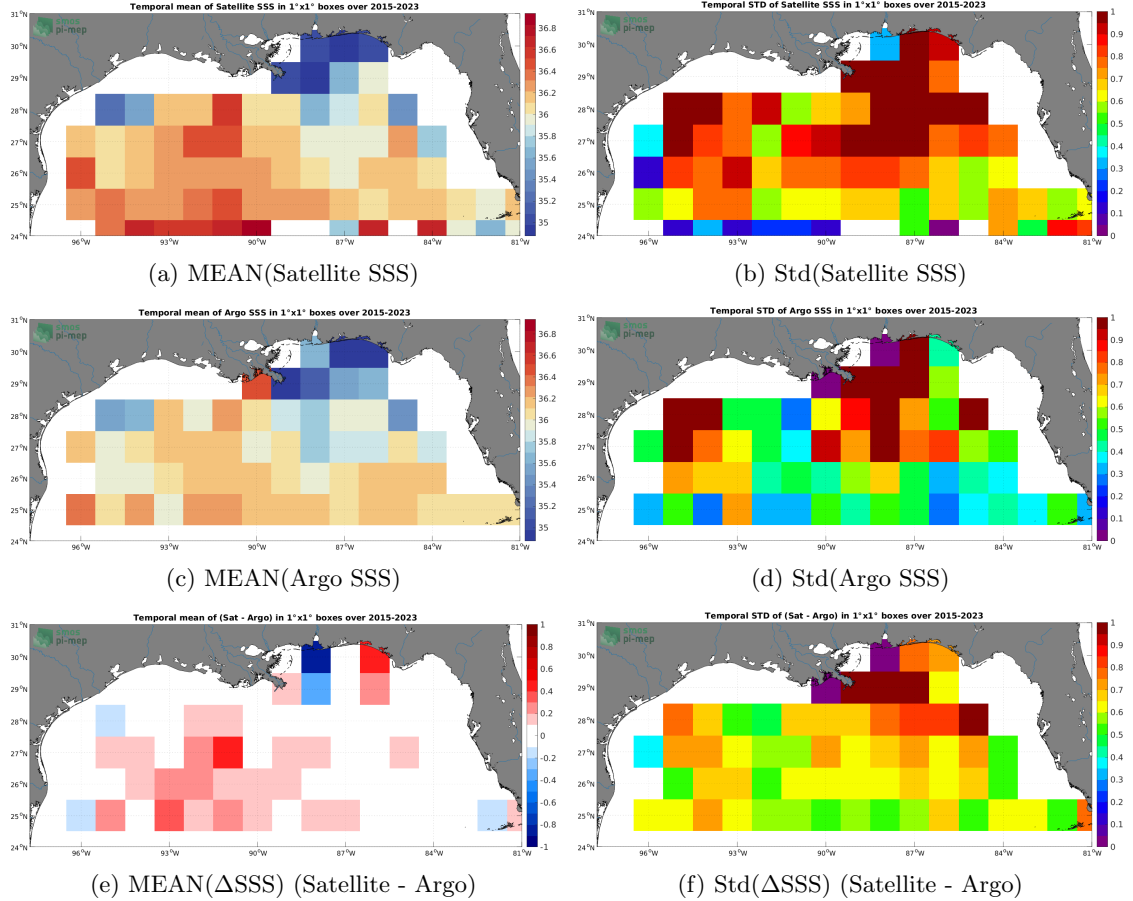
Figure 6: Temporal mean (left) and Std (right) of SSS from SMAP SSS L2 v5.0 (JPL) (top), Argo (middle), and of \Delta\text{SSS} (Satellite - Argo). Only match-up pairs are used to generate these maps.
