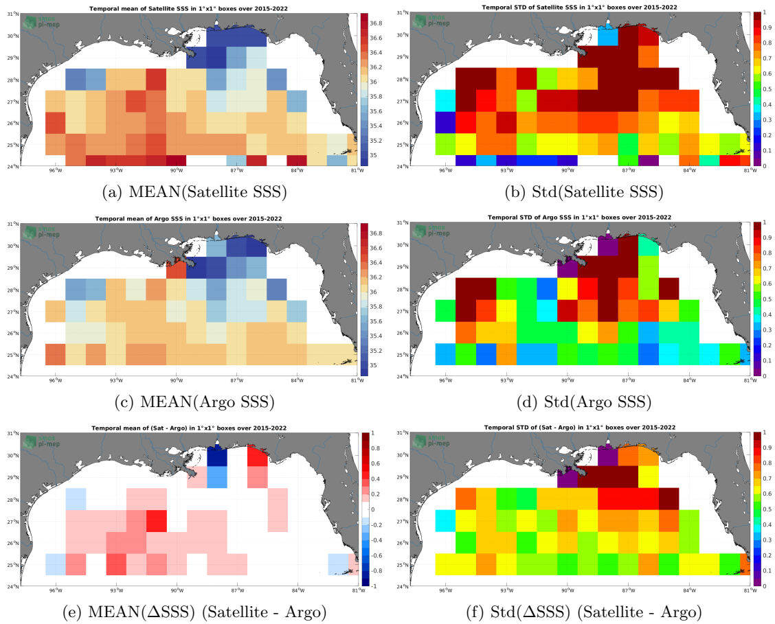
Figure 6: Temporal mean (left) and Std (right) of SSS from SMAP SSS L2 v5.0 (JPL) (top), Argo (middle), and of \Delta SSS (Satellite - Argo). Only match-up pairs are used to generate these maps.
