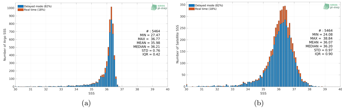
Figure 2: Histograms of SSS from Argo (a) and SMAP SSS L2 v5.0 (JPL) (b) considering all match-up pairs per bins of 0.1 over the Mississippi river plume Pi-MEP region and for the full satellite product period.
