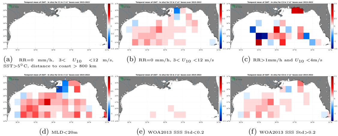
Figure 12: Temporal mean gridded over spatial boxes of size 1^{\circ}\times 1^{\circ} of \Delta\text{SSS} (SMAP SSS L2 v5.0 (JPL) - Argo) for 6 different subdatasets corresponding to:RR=0 mm/h, 3 < U_{10} < 12 m/s, SST > 5^{\circ}\text{C} , distance to coast > 800 km (a), RR=0 mm/h, 3 < U_{10} < 12 m/s (b), RR > 1 mm/h and U_{10} < 4 m/s (c),MLD < 20\text{m} (d),WOA2013 SSS Std < 0.2 (e),WOA2013 SSS Std > 0.2 (f).
