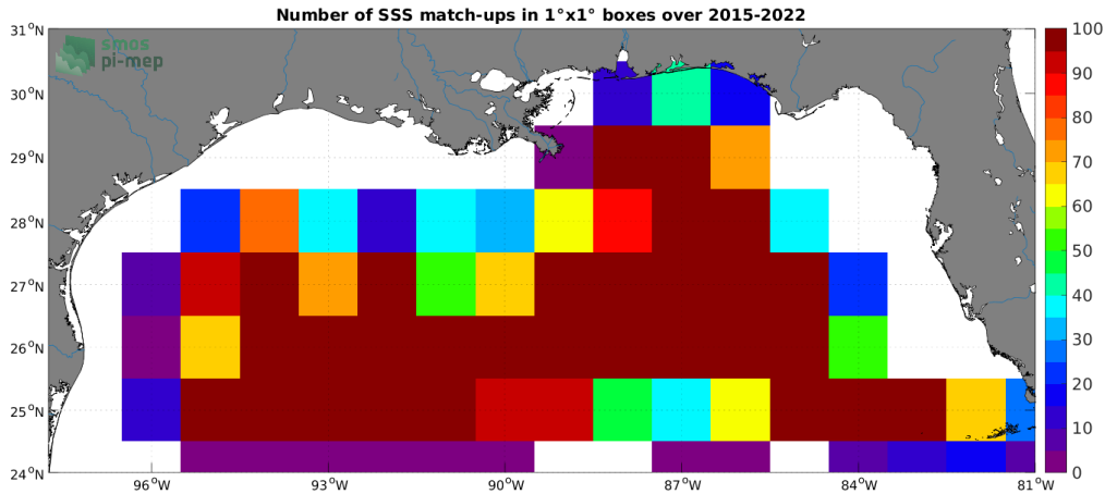
Figure 4: Number of SSS match-ups between Argo SSS and the SMAP SSS L2 v5.0 (JPL) SSS product for the Mississippi river plume Pi-MEP region over 1^\circ \times 1^\circ boxes and for the full satellite product period.
