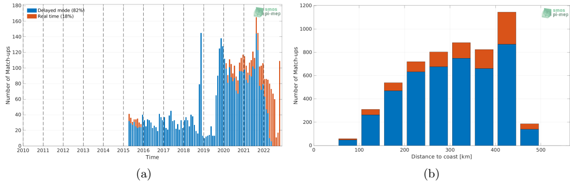
Figure 1: Number of match-ups between Argo and SMAP SSS L2 v5.0 (JPL) SSS as a function of time (a) and as function of the distance to coast (b) over the Mississippi river plume Pi-MEP region and for the full satellite product period.
