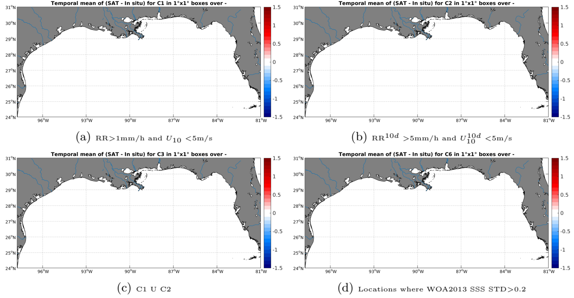
Figure 12: Temporal mean gridded over spatial boxes of size 1^\circ \times 1^\circ of \Delta SSS (SMAP-L2-JPL-V4 - TSG-LEGOS-DM) for 4 different subdatasets corresponding to: RR > 1\text{mm/h} and U_{10} < 5\text{m/s} (a), RR^{10d} > 5\text{mm/h} and U_{10}^{10d} < 5\text{m/s} (b), C1 U C2 (c), Locations where WOA2013 SSS STD > 0.2 (d).
