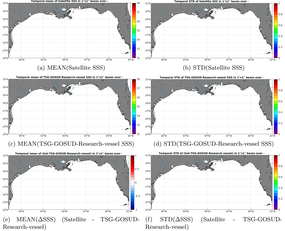
Figure 6: Temporal mean (left) and STD (right) of SSS from SMAP-L2-JPL-V4 (top), TSG-GOSUD-Research-vessel (middle), and of \Delta\text{SSS} (Satellite - TSG-GOSUD-Research-vessel). Only match-up pairs are used to generate these maps.
