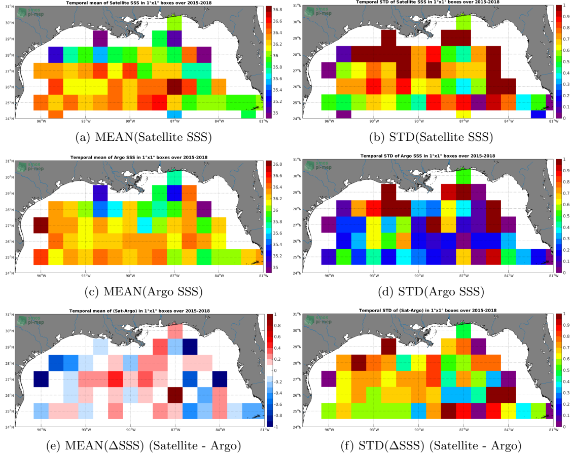
Figure 6: Temporal mean (left) and STD (right) of SSS from SMAP-L2-JPL-V4 (top), Argo (middle), and of \Delta SSS (Satellite - Argo). Only match-up pairs are used to generate these maps.
