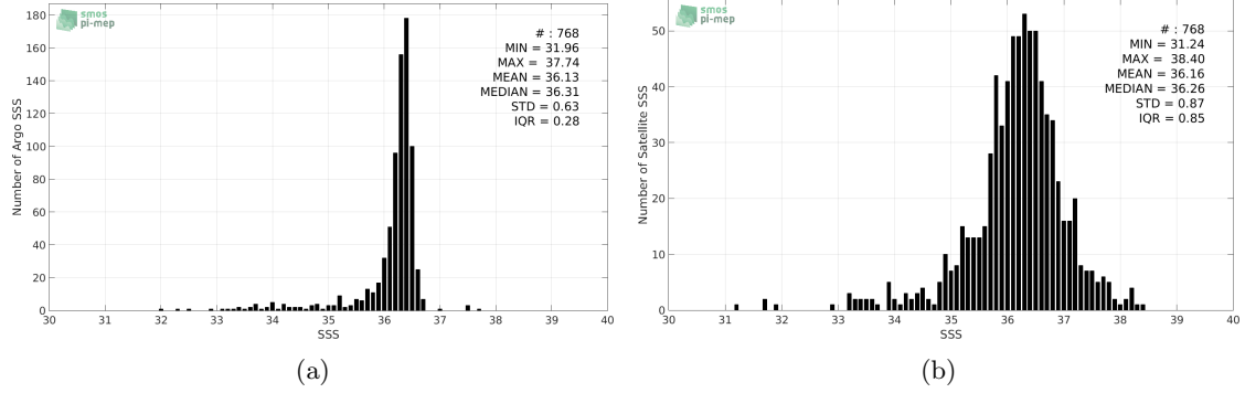
Figure 2: Histograms of SSS from Argo (a) and SMAP-L2-JPL-V4 (b) considering all match-up pairs per bins of 0.1 over the Mississippi river plume Pi-MEP region and for the full satellite product period.
