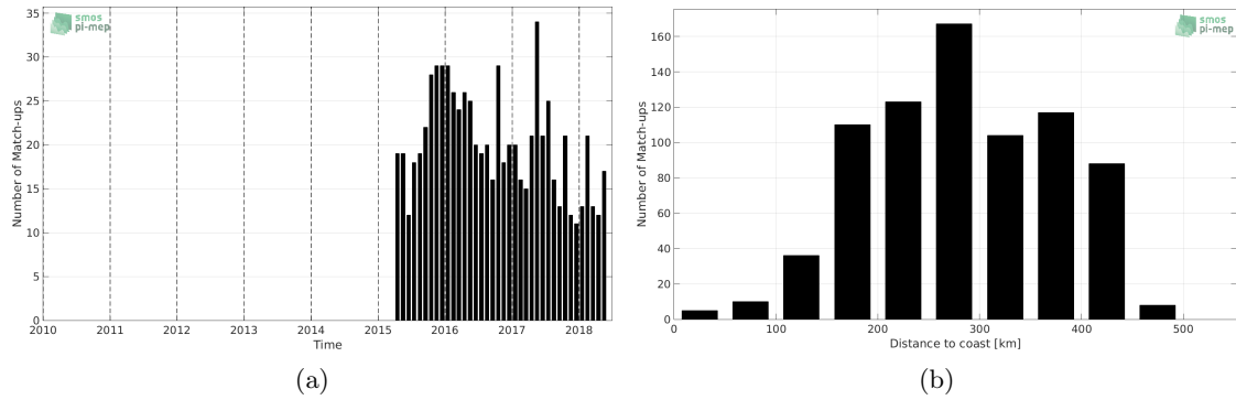
Figure 1: Number of match-ups between Argo and SMAP-L2-JPL-V4 SSS as a function of time (a) and as function of the distance to coast (b) over the Mississippi river plume Pi-MEP region and for the full satellite product period.
