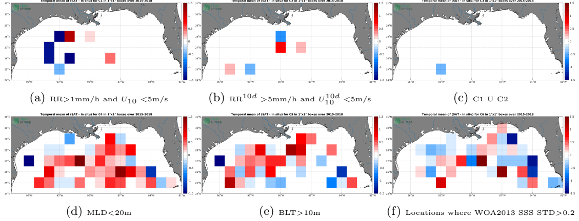
Figure 12: Temporal mean gridded over spatial boxes of size 1^\circ \times 1^\circ of \Delta SSS (SMAP-L2-JPL-V4 - Argo) for 6 different subdatasets corresponding to: RR > 1\text{mm/h} and U_{10} < 5\text{m/s} (a), RR^{10d} > 5\text{mm/h} and U_{10}^{10d} < 5\text{m/s} (b), C1 U C2 (c), MLD < 20\text{m} (d), BLT > 10\text{m} (e), Locations where WOA2013 SSS STD > 0.2 (f).
