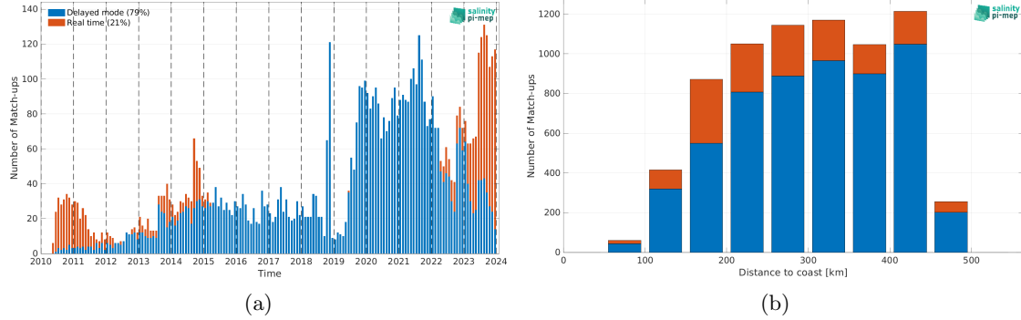
Figure 2: Number of match-ups between Argo and CCI SSS L4 Merged-OI v5.5 - 7-day running (ESA) SSS as a function of time (a) and as function of the distance to coast (b) over the Mississippi river plume Pi-MEP region and for the full satellite product period.
