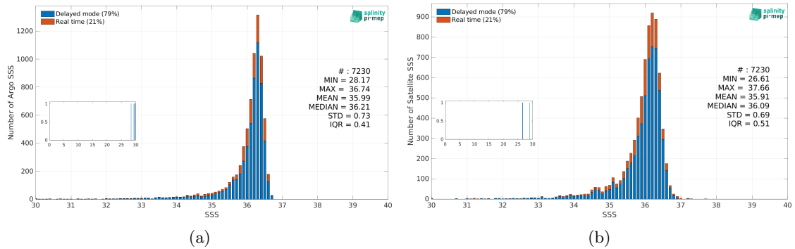
Figure 3: Histograms of SSS from Argo (a) and CCI SSS L4 Merged-OI v5.5 - 7-day running (ESA) (b) considering all match-up pairs per bins of 0.1 over the Mississippi river plume Pi-MEP region and for the full satellite product period.
