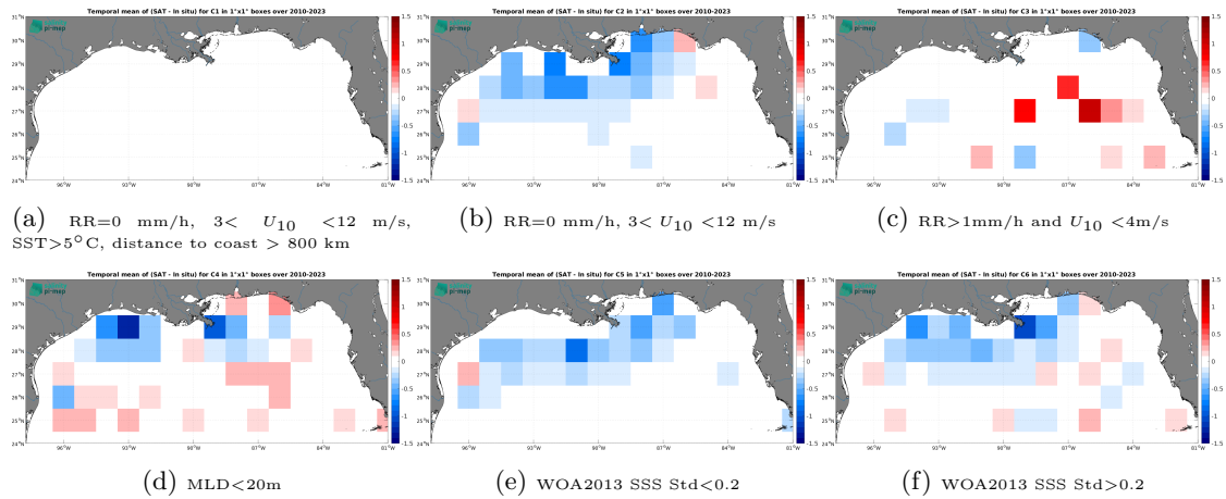
Figure 14: Temporal mean gridded over spatial boxes of size 1^\circ \times 1^\circ of \Delta SSS (CCI SSS L4 Merged-OI v5.5 - 7-day running (ESA) - Argo) for 6 different subdatasets corresponding to:RR=0 mm/h, 3 < U_{10} < 12 m/s, SST >5^\circ C, distance to coast > 800 km (a), RR=0 mm/h, 3 < U_{10} < 12 m/s (b), RR >1 mm/h and U_{10} < 4 m/s (c),MLD <20 m (d),WOA2013 SSS Std <0.2 (e),WOA2013 SSS Std >0.2 (f).
