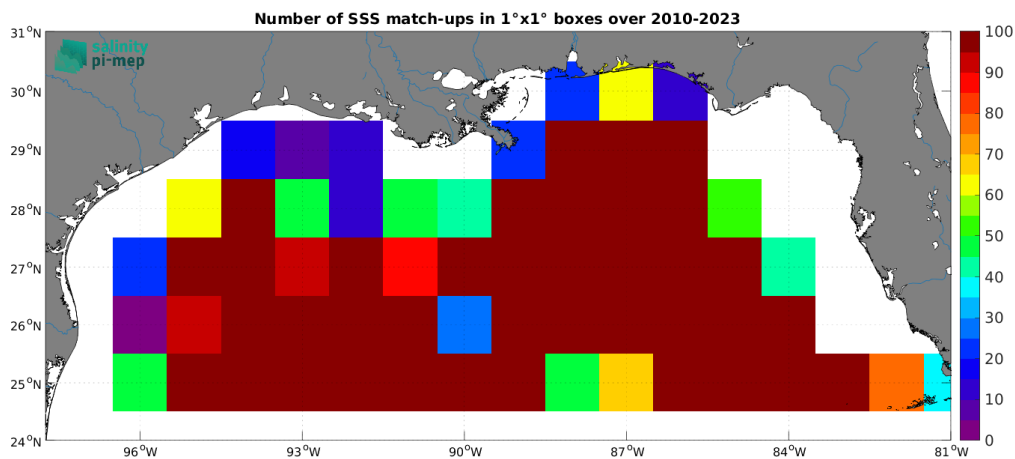
Figure 5: Number of SSS match-ups between Argo SSS and the CCI SSS L4 Merged-OI v5.5 - 7-day running (ESA) SSS product for the Mississippi river plume Pi-MEP region over 1^\circ \times 1^\circ boxes and for the full satellite product period.
