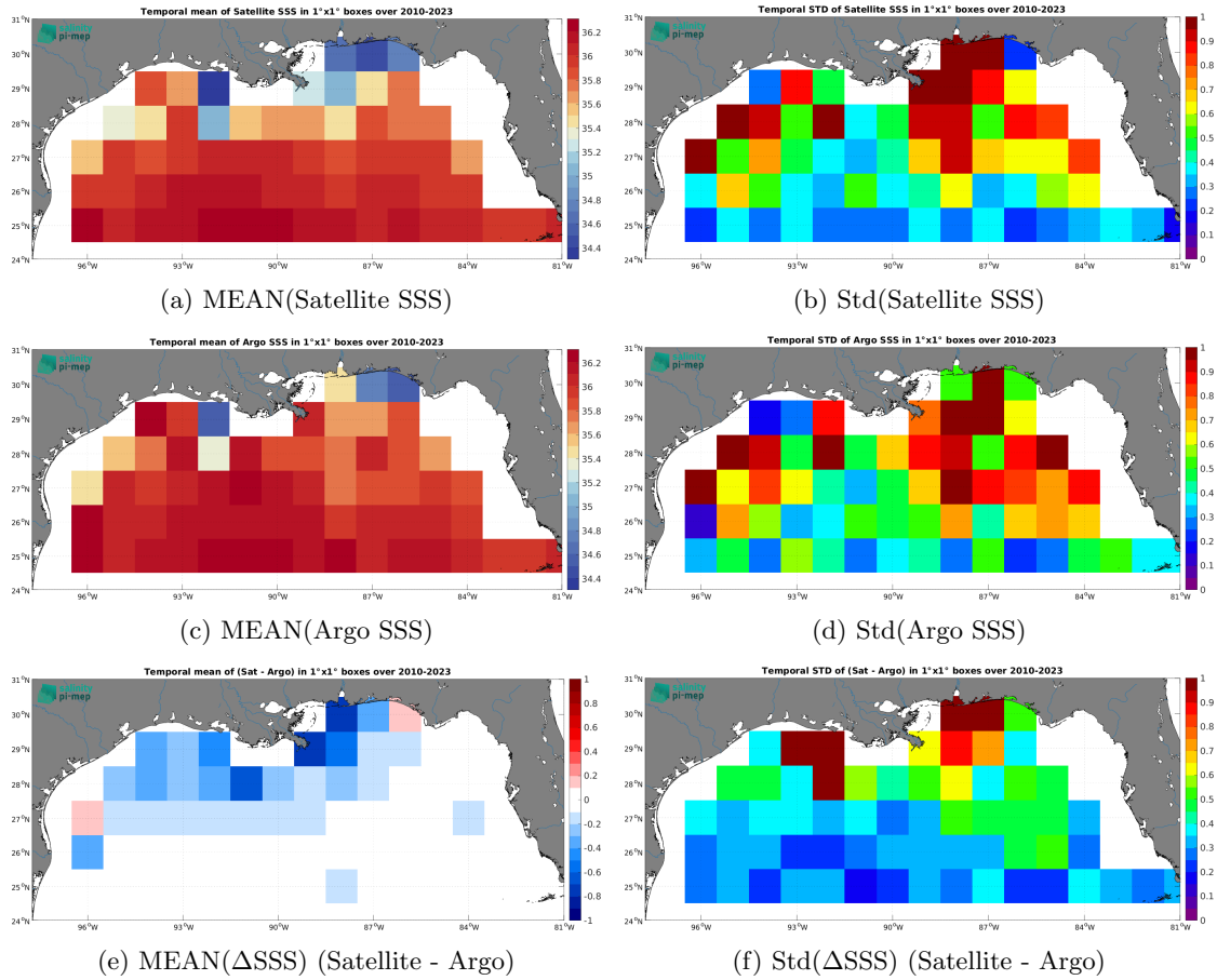
Figure 7: Temporal mean (left) and Std (right) of SSS from CCI SSS L4 Merged-OI v5.5 - 7-day running (ESA) (top), Argo (middle), and of \Delta SSS (Satellite - Argo). Only match-up pairs are used to generate these maps.
