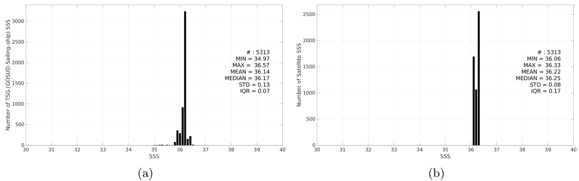
Figure 3: Histograms of SSS from TSG (GOSUD-Sailing-ship) (a) and CCI SSS L4 Merged-OI v5.5 - 30-day running (ESA) (b) considering all match-up pairs per bins of 0.1 over the Mississippi river plume Pi-MEP region and for the full satellite product period.
