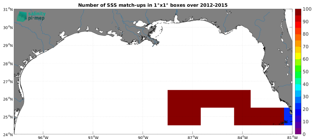
Figure 5: Number of SSS match-ups between TSG (GOSUD-Sailing-ship) SSS and the CCI SSS L4 Merged-OI v5.5 - 30-day running (ESA) SSS product for the Mississippi river plume Pi-MEP region over 1^\circ \times 1^\circ boxes and for the full satellite product period.
