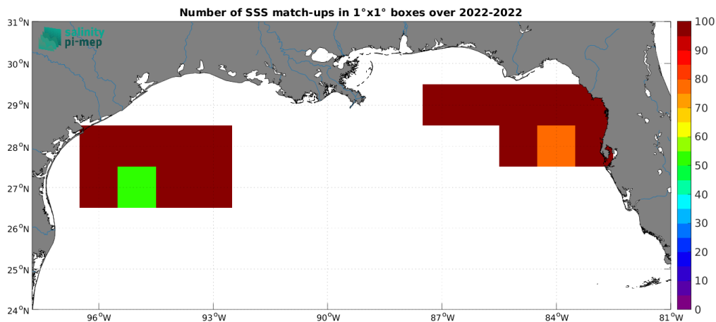
Figure 5: Number of SSS match-ups between Saildrone SSS and the CCI SSS L4 Merged-OI v5.5 - 30-day running (ESA) SSS product for the Mississippi river plume Pi-MEP region over 1^\circ \times 1^\circ boxes and for the full satellite product period.
