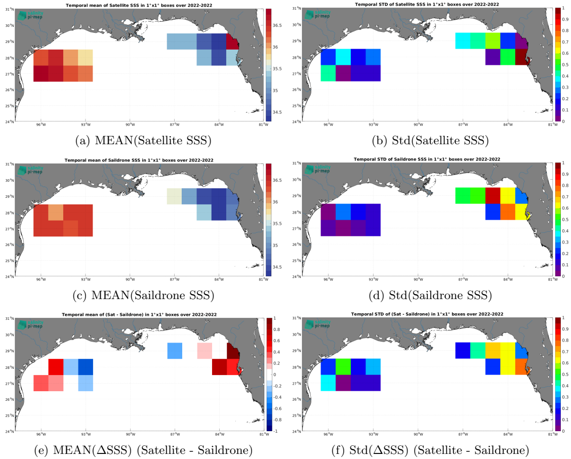
Figure 7: Temporal mean (left) and Std (right) of SSS from CCI SSS L4 Merged-OI v5.5 - 30-day running (ESA) (top), Saildrone (middle), and of \Delta SSS (Satellite - Saildrone). Only match-up pairs are used to generate these maps.
