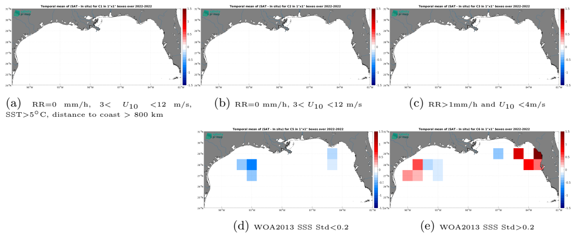
Figure 14: Temporal mean gridded over spatial boxes of size 1^\circ \times 1^\circ of \Delta SSS (CCI SSS L4 Merged-OI v5.5 - 30-day running (ESA) - Saildrone) for 5 different subdatasets corresponding to: RR=0 mm/h, 3 < U_{10} < 12 m/s, SST > 5°C, distance to coast > 800 km (a), RR=0 mm/h, 3 < U_{10} < 12 m/s (b), RR > 1 mm/h and U_{10} < 4 m/s (c), WOA2013 SSS Std < 0.2 (d), WOA2013 SSS Std > 0.2 (e).
