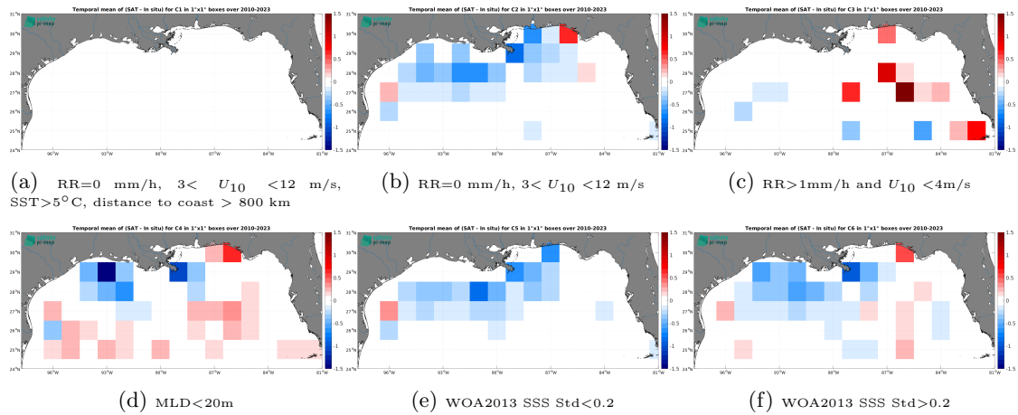
Figure 14: Temporal mean gridded over spatial boxes of size 1^\circ \times 1^\circ of \Delta SSS (CCI SSS L4 Merged-OI v5.5 - 30-day running (ESA) - Argo) for 6 different subdatasets corresponding to:RR=0 mm/h, 3 < U_{10} < 12 m/s, SST >5^\circ C, distance to coast > 800 km (a), RR=0 mm/h, 3 < U_{10} < 12 m/s (b), RR >1 mm/h and U_{10} < 4 m/s (c),MLD <20 m (d),WOA2013 SSS Std <0.2 (e),WOA2013 SSS Std >0.2 (f).
