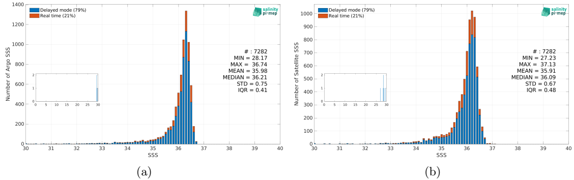
Figure 3: Histograms of SSS from Argo (a) and CCI SSS L4 Merged-OI v5.5 - 30-day running (ESA) (b) considering all match-up pairs per bins of 0.1 over the Mississippi river plume Pi-MEP region and for the full satellite product period.
