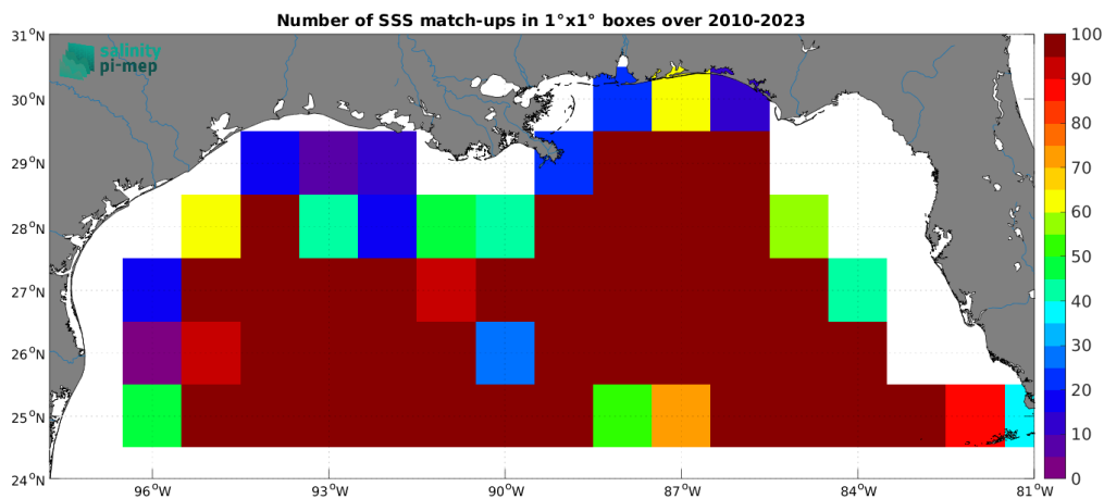
Figure 5: Number of SSS match-ups between Argo SSS and the CCI SSS L4 Merged-OI v5.5 - 30-day running (ESA) SSS product for the Mississippi river plume Pi-MEP region over 1^{\circ} \times 1^{\circ} boxes and for the full satellite product period.
