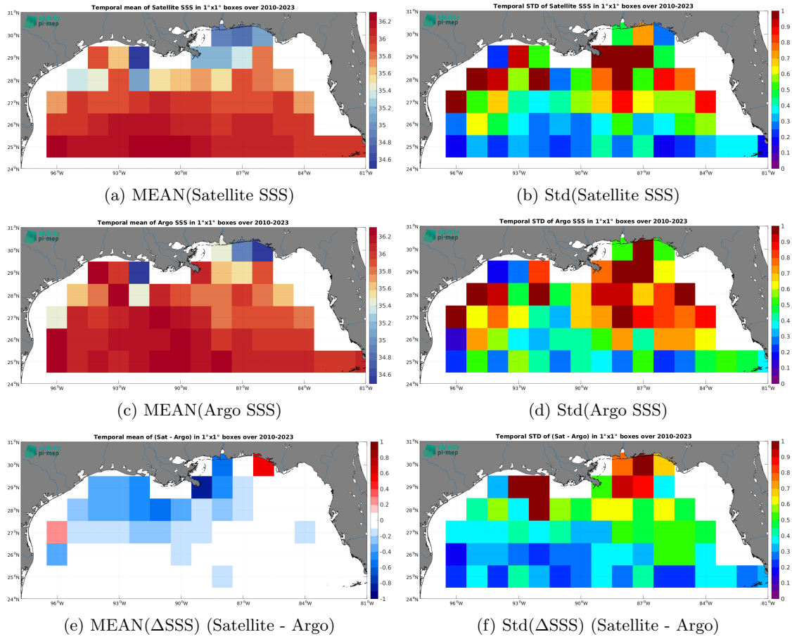
Figure 7: Temporal mean (left) and Std (right) of SSS from CCI SSS L4 Merged-OI v5.5 - 30-day running (ESA) (top), Argo (middle), and of \Delta SSS (Satellite - Argo). Only match-up pairs are used to generate these maps.
