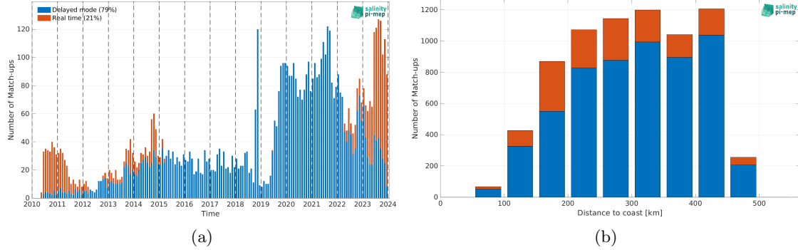
Figure 2: Number of match-ups between Argo and CCI SSS L4 Merged-OI v5.5 - 30-day running (ESA) SSS as a function of time (a) and as function of the distance to coast (b) over the Mississippi river plume Pi-MEP region and for the full satellite product period.
