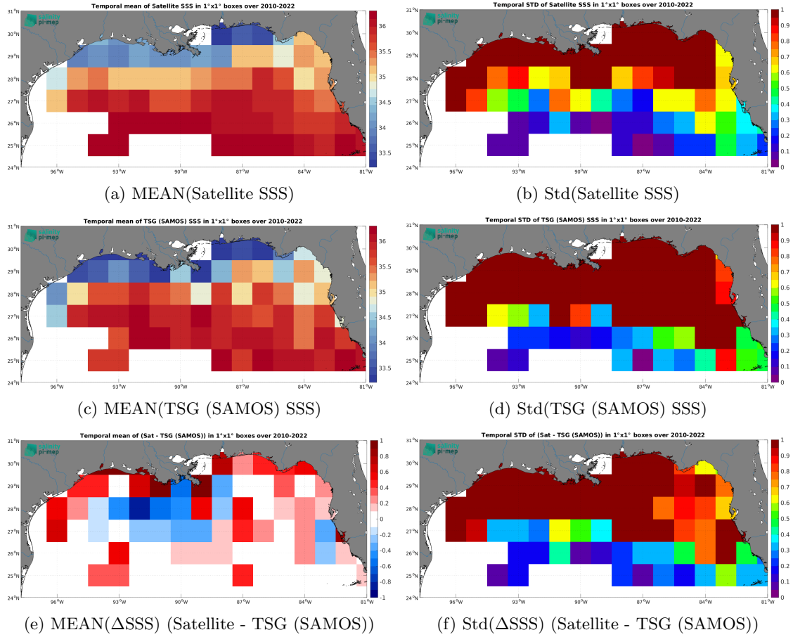
Figure 7: Temporal mean (left) and Std (right) of SSS from CCI SSS L4 Merged-OI v4.41 - 30-day running (ESA) (top), TSG (SAMOS) (middle), and of \Delta\text{SSS} (Satellite - TSG (SAMOS)). Only match-up pairs are used to generate these maps.
