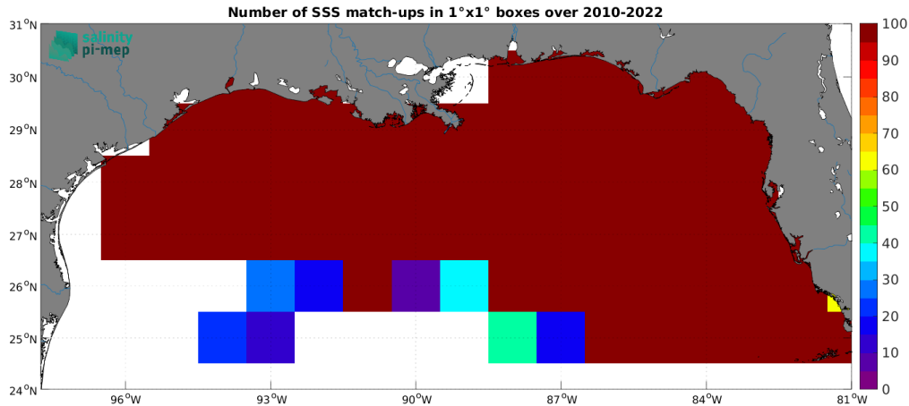
Figure 5: Number of SSS match-ups between TSG (SAMOS) SSS and the CCI SSS L4 Merged-OI v4.41 - 30-day running (ESA) SSS product for the Mississippi river plume Pi-MEP region over 1^\circ \times 1^\circ boxes and for the full satellite product period.
