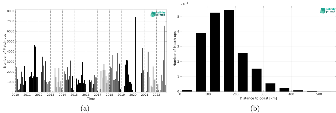
Figure 2: Number of match-ups between TSG (SAMOS) and CCI SSS L4 Merged-OI v4.41 - 30-day running (ESA) SSS as a function of time (a) and as function of the distance to coast (b) over the Mississippi river plume Pi-MEP region and for the full satellite product period.
