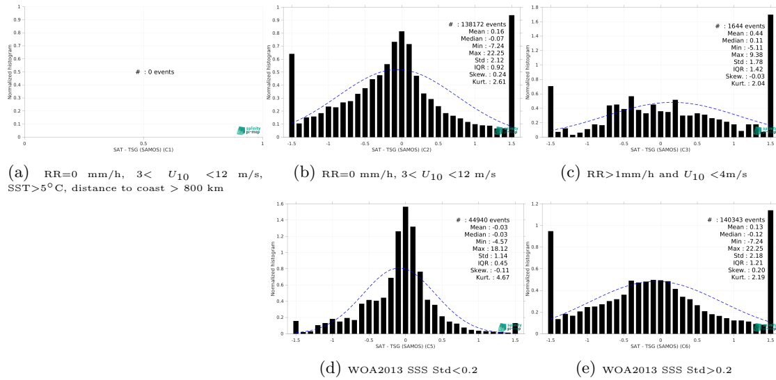
Figure 15: Normalized histogram of \Delta SSS (CCI SSS L4 Merged-OI v4.41 - 30-day running (ESA) - TSG (SAMOS)) for 5 different subdatasets corresponding to: RR=0 mm/h, 3 < U_{10} < 12 m/s, SST > 5°C, distance to coast > 800 km (a), RR=0 mm/h, 3 < U_{10} < 12 m/s (b), RR > 1mm/h and U_{10} < 4 m/s (c), WOA2013 SSS Std < 0.2 (d), WOA2013 SSS Std > 0.2 (e).
