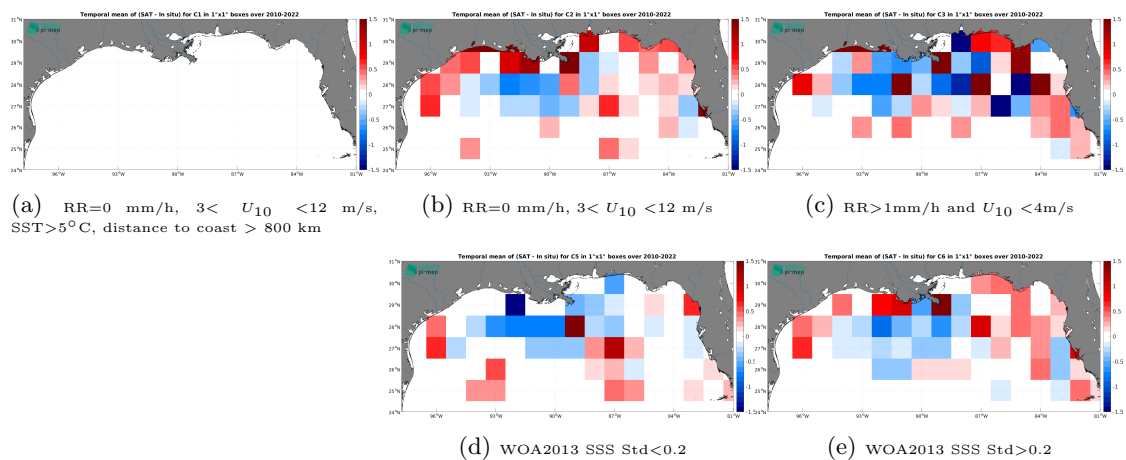
Figure 14: Temporal mean gridded over spatial boxes of size 1^\circ \times 1^\circ of \Delta\text{SSS} (CCI SSS L4 Merged-OI v4.41 - 30-day running (ESA) - TSG (SAMOS)) for 5 different subdatasets corresponding to:RR=0 mm/h, 3 < U_{10} < 12 m/s, SST >5^\circ\text{C} , distance to coast > 800 km (a), RR=0 mm/h, 3 < U_{10} < 12 m/s (b), RR >1 mm/h and U_{10} < 4 m/s (c), WOA2013 SSS Std <0.2 (d), WOA2013 SSS Std >0.2 (e).
