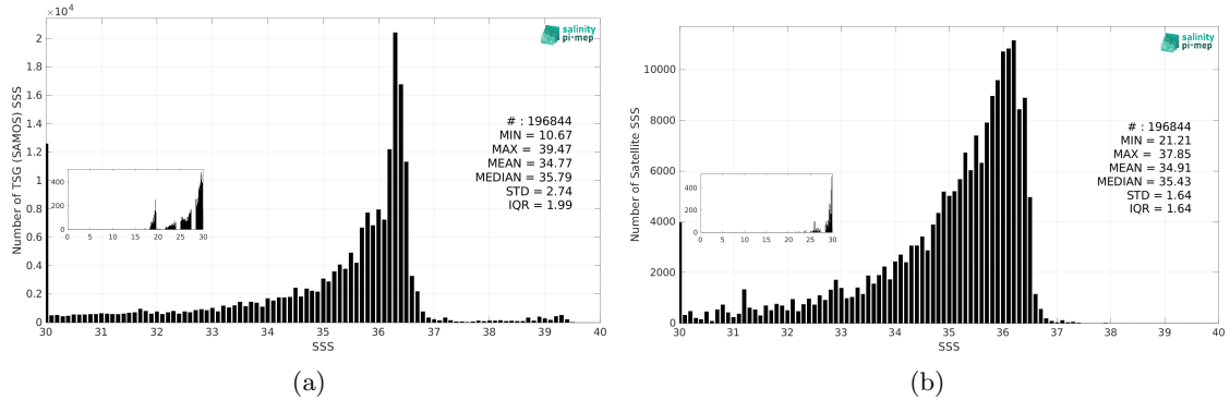
Figure 3: Histograms of SSS from TSG (SAMOS) (a) and CCI SSS L4 Merged-OI v4.41 - 30-day running (ESA) (b) considering all match-up pairs per bins of 0.1 over the Mississippi river plume Pi-MEP region and for the full satellite product period.
