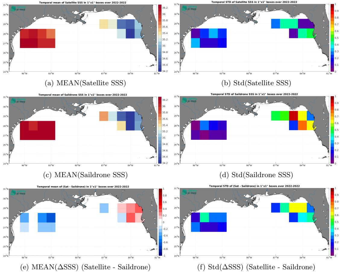
Figure 7: Temporal mean (left) and Std (right) of SSS from CCI SSS L4 Merged-OI v4.41 - 30-day running (ESA) (top), Saildrone (middle), and of \Delta\text{SSS} (Satellite - Saildrone). Only match-up pairs are used to generate these maps.
