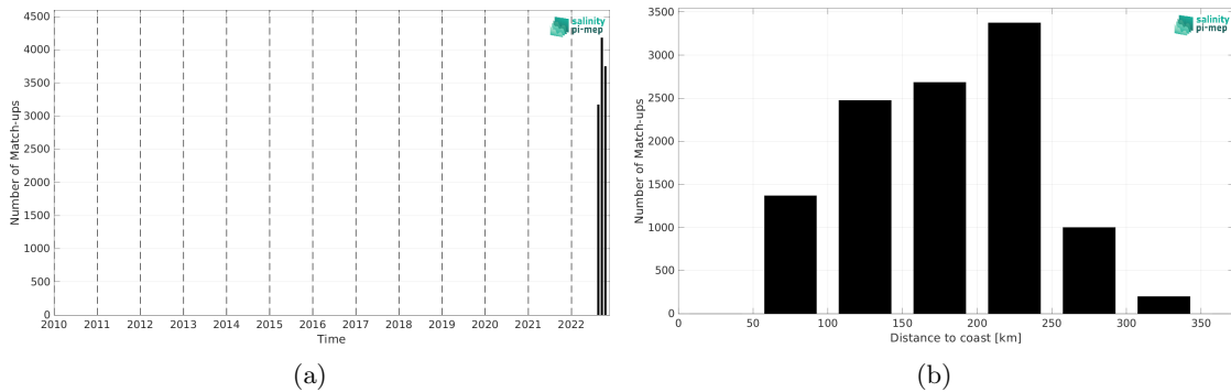
Figure 2: Number of match-ups between Saildrone and CCI SSS L4 Merged-OI v4.41 - 30-day running (ESA) SSS as a function of time (a) and as function of the distance to coast (b) over the Mississippi river plume Pi-MEP region and for the full satellite product period.
