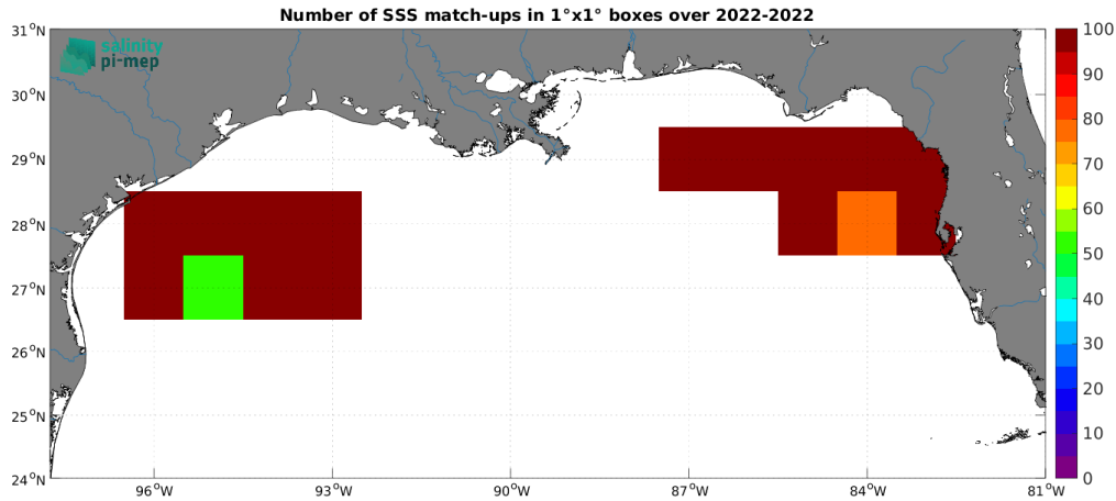
Figure 5: Number of SSS match-ups between Saildrone SSS and the CCI SSS L4 Merged-OI v4.41 - 30-day running (ESA) SSS product for the Mississippi river plume Pi-MEP region over 1^\circ \times 1^\circ boxes and for the full satellite product period.
