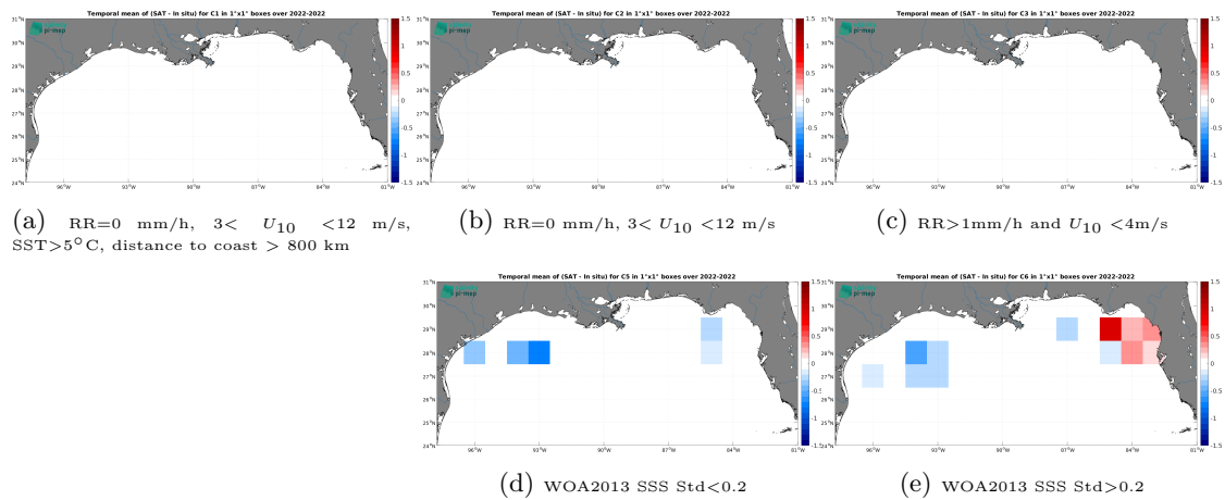
Figure 14: Temporal mean gridded over spatial boxes of size 1^\circ \times 1^\circ of \Delta SSS (CCI SSS L4 Merged-OI v4.41 - 30-day running (ESA) - Saildrone) for 5 different subdatasets corresponding to:RR=0 mm/h, 3 < U_{10} < 12 m/s, SST >5^\circ\text{C} , distance to coast > 800 km (a), RR=0 mm/h, 3 < U_{10} < 12 m/s (b), RR >1 mm/h and U_{10} < 4 m/s (c), WOA2013 SSS Std <0.2 (d), WOA2013 SSS Std >0.2 (e).
