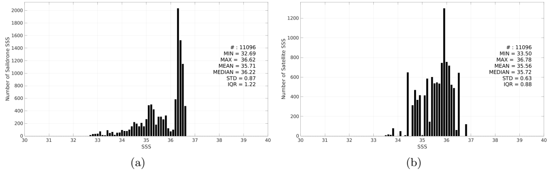
Figure 3: Histograms of SSS from Saildrone (a) and CCI SSS L4 Merged-OI v4.41 - 30-day running (ESA) (b) considering all match-up pairs per bins of 0.1 over the Mississippi river plume Pi-MEP region and for the full satellite product period.
